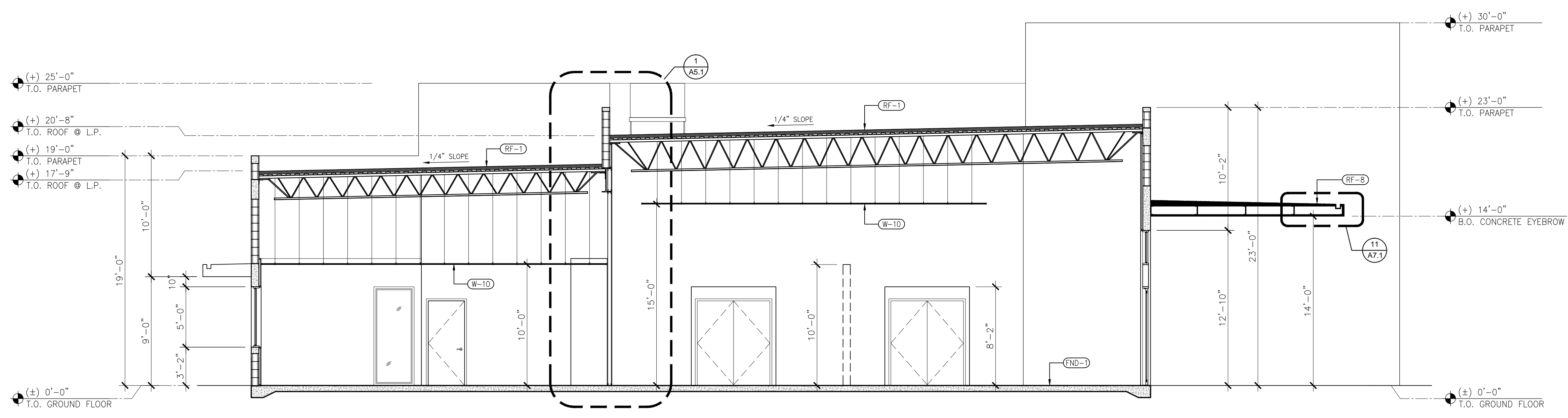
C BUILDING SECTION
