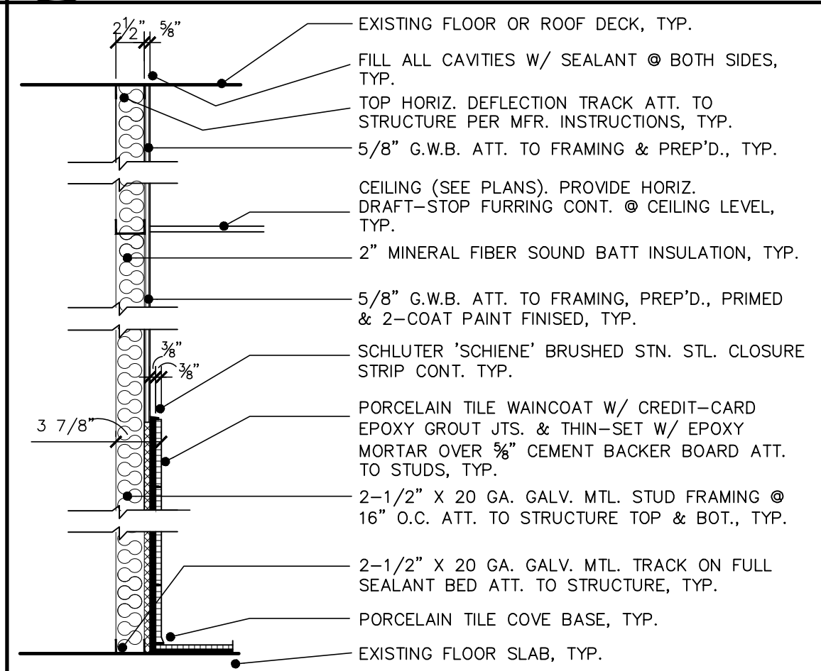
9 FURRED PARTITION TYPE 9 A904 NOT TO SCALE
