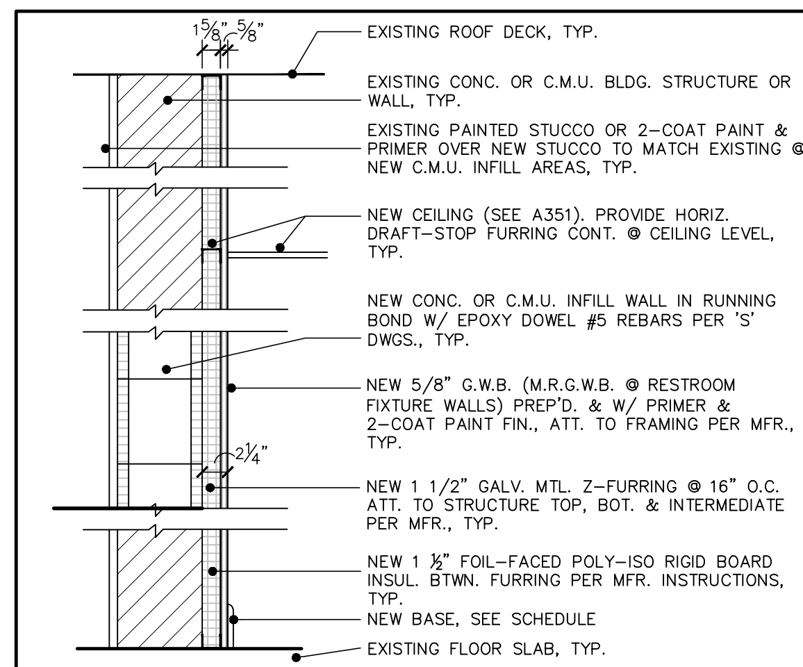
1 FURRED NEW & EXIST. MAS. TYPE 1 A904 NOT TO SCALE
