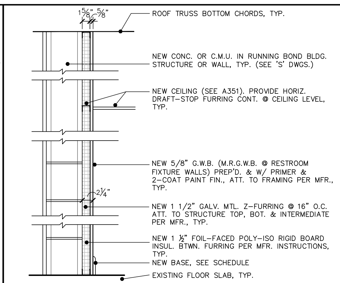
3 FURRED EXISTING MAS. TYPE 3 A904 NOT TO SCALE
