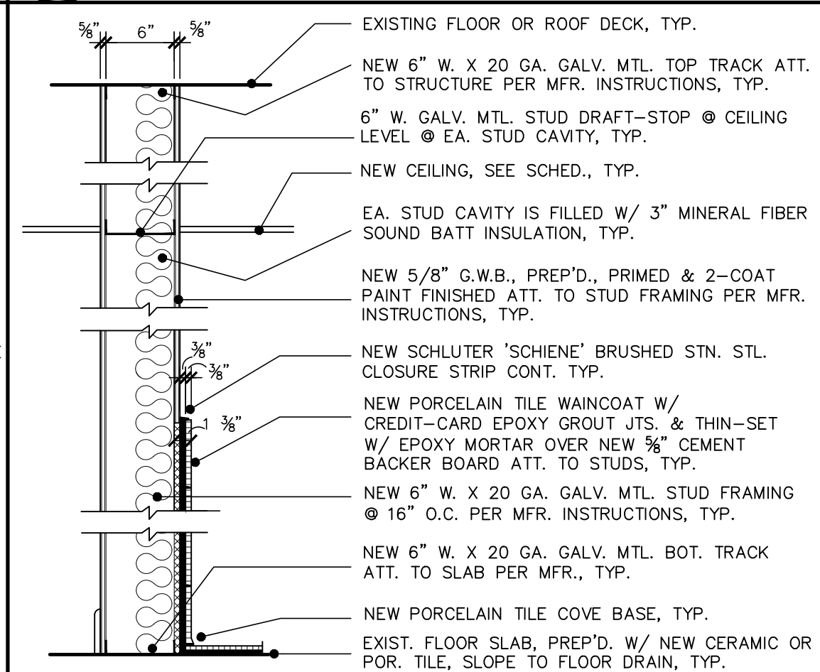
8 PARTITION TYPE 8 A904 NOT TO SCALE
