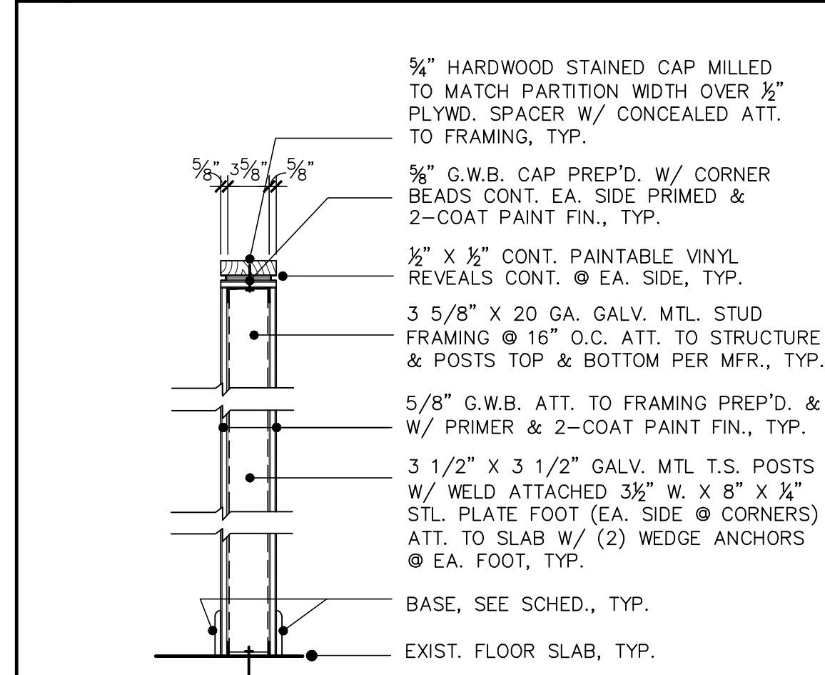
11 PARTITION TYPE 11 A904 NOT TO SCALE
