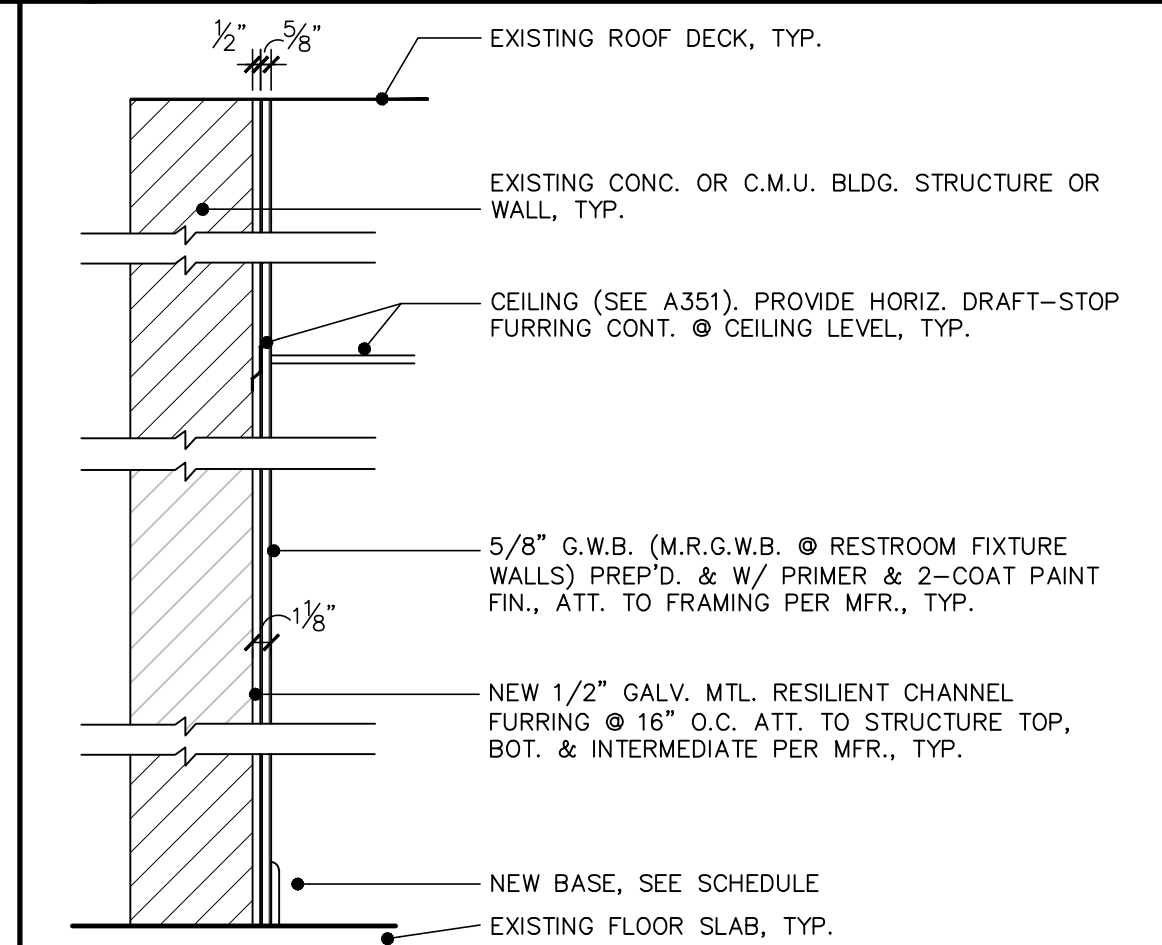
12 FURRED WALL TYPE 14 A904 NOT TO SCALE
