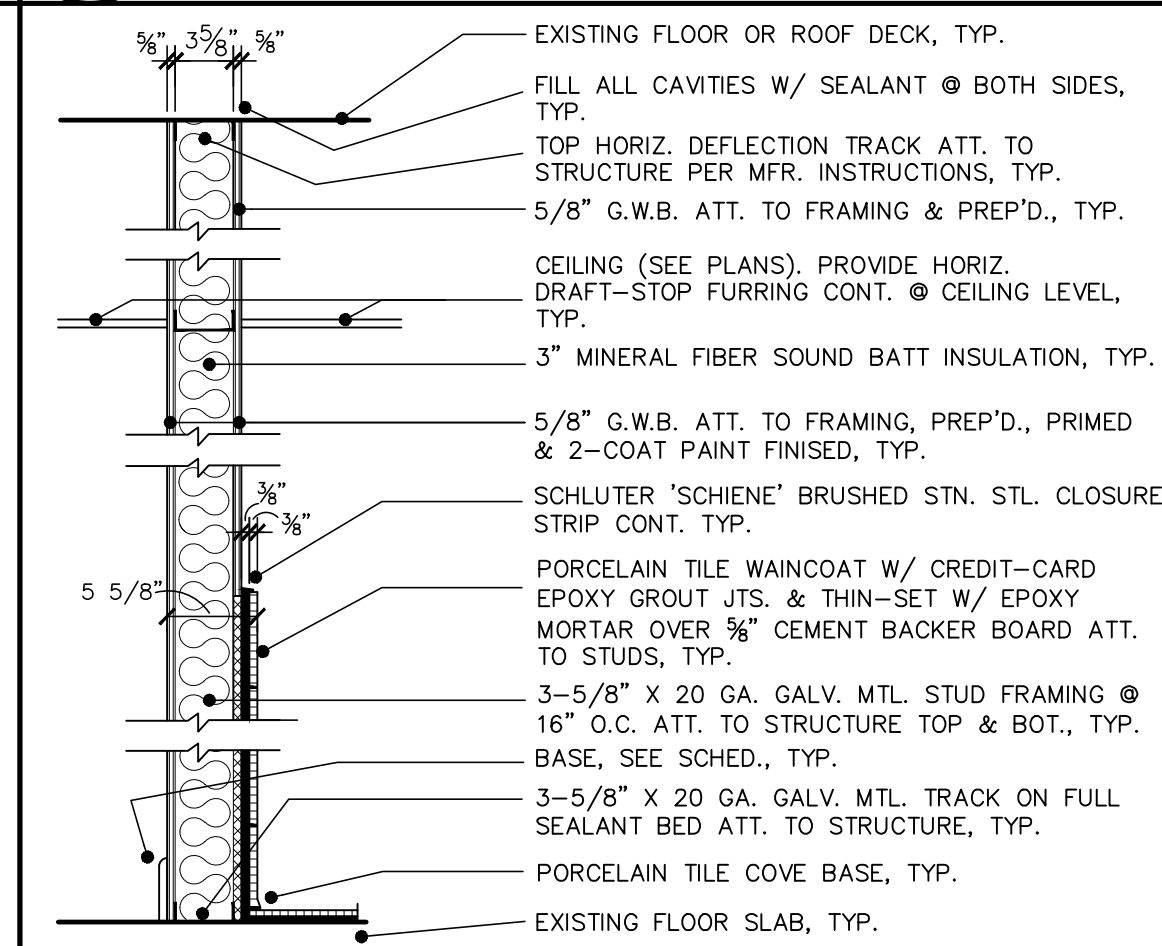
7 PARTITION TYPE 7 A904 NOT TO SCALE
