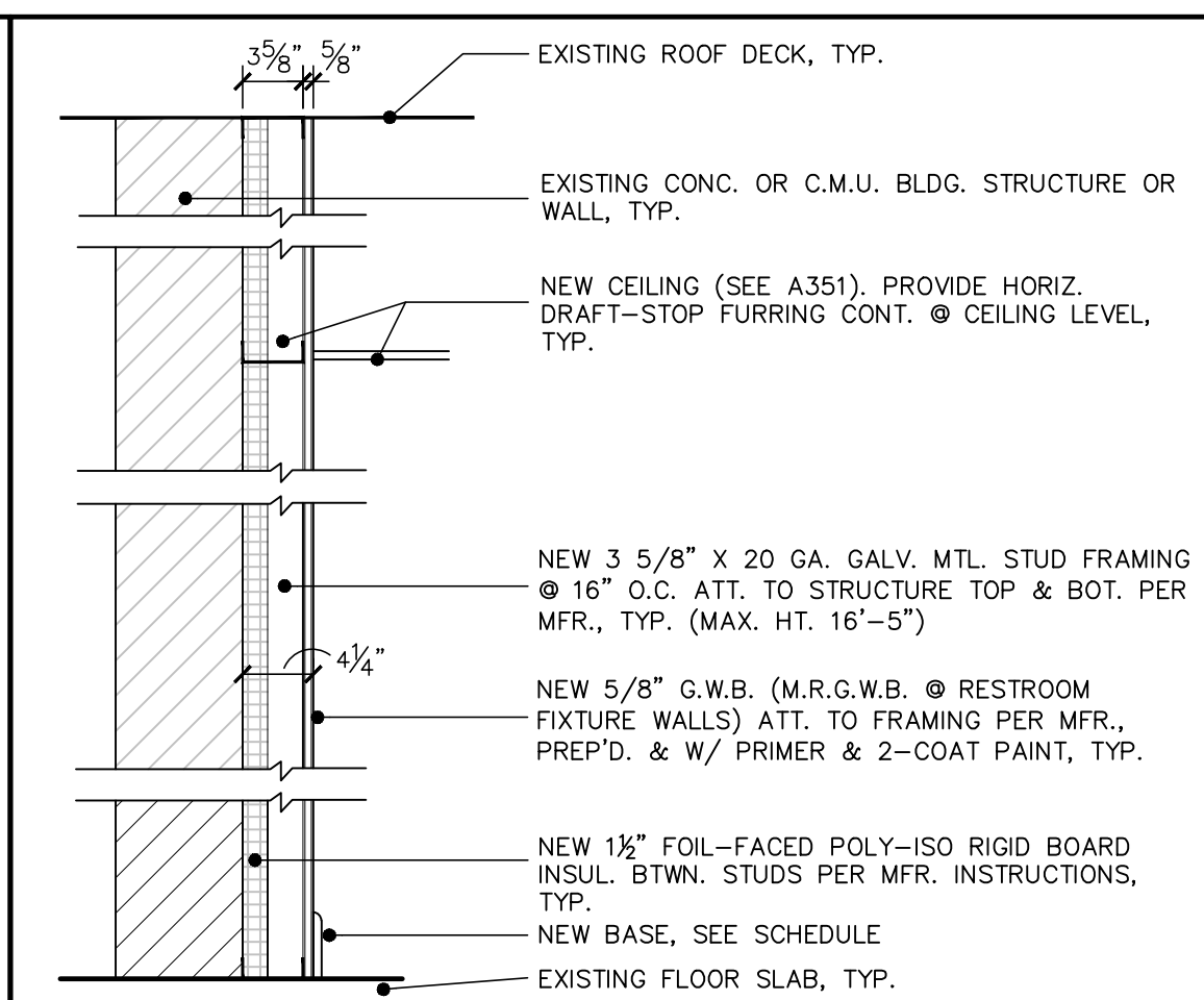
4 FURRED EXIST. C.M.U. TYPE 4 A904 NOT TO SCALE
