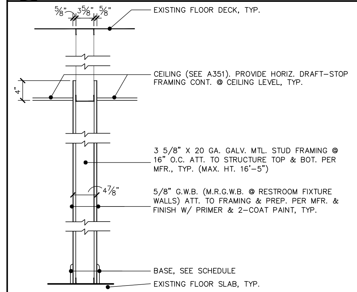
6 PARTITION TYPE 6 A904 NOT TO SCALE
