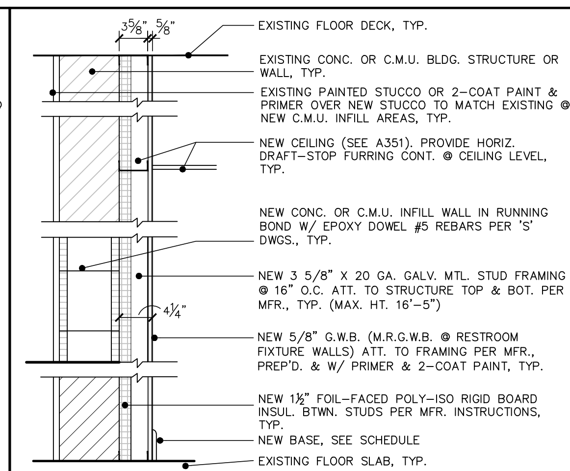
2 FURRED NEW & EXIST. MAS. TYPE 2 A904 NOT TO SCALE
