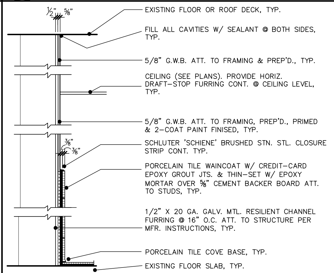
10 FURRED PARTITION TYPE 10 A904 NOT TO SCALE
