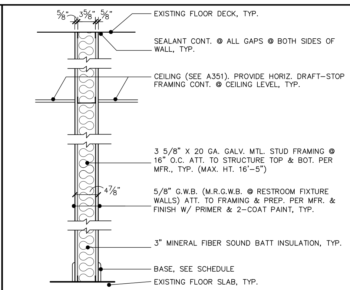
5 PARTITION TYPE 5 A904 NOT TO SCALE
