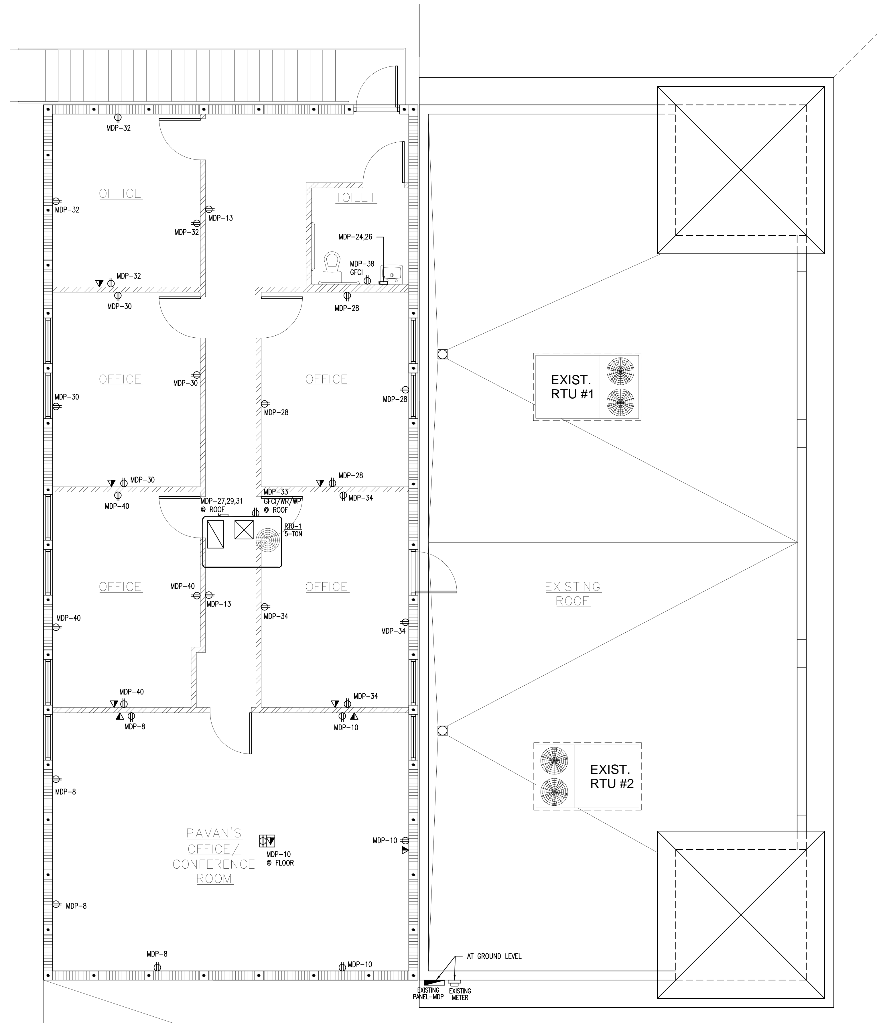
2ND FLOOR POWER PLAN SCALE: 1/4" = 1'-0"
