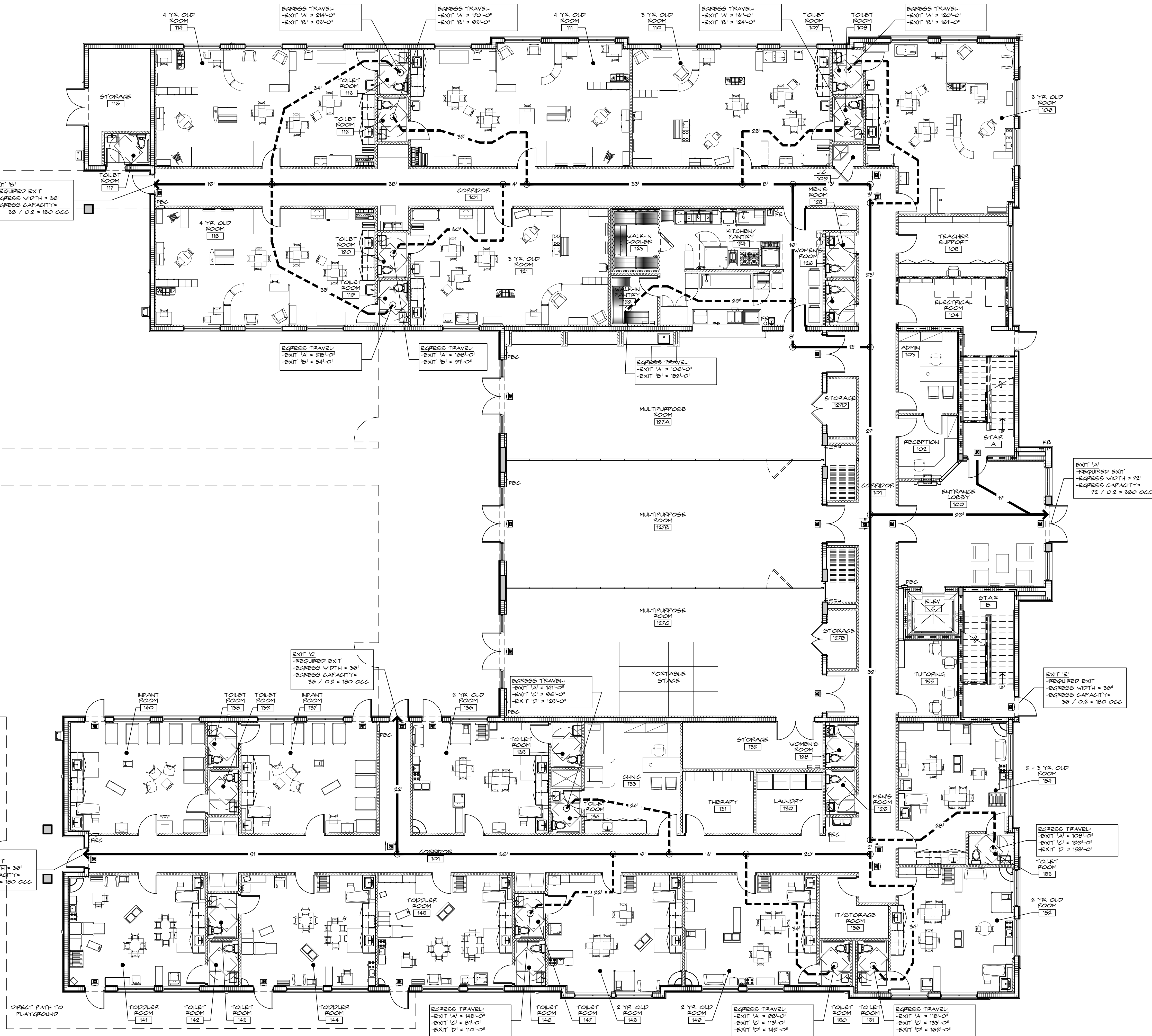
1 FIRST FLOOR LIFE SAFETY PLAN SCALE: 1/8" = 1'-0"
