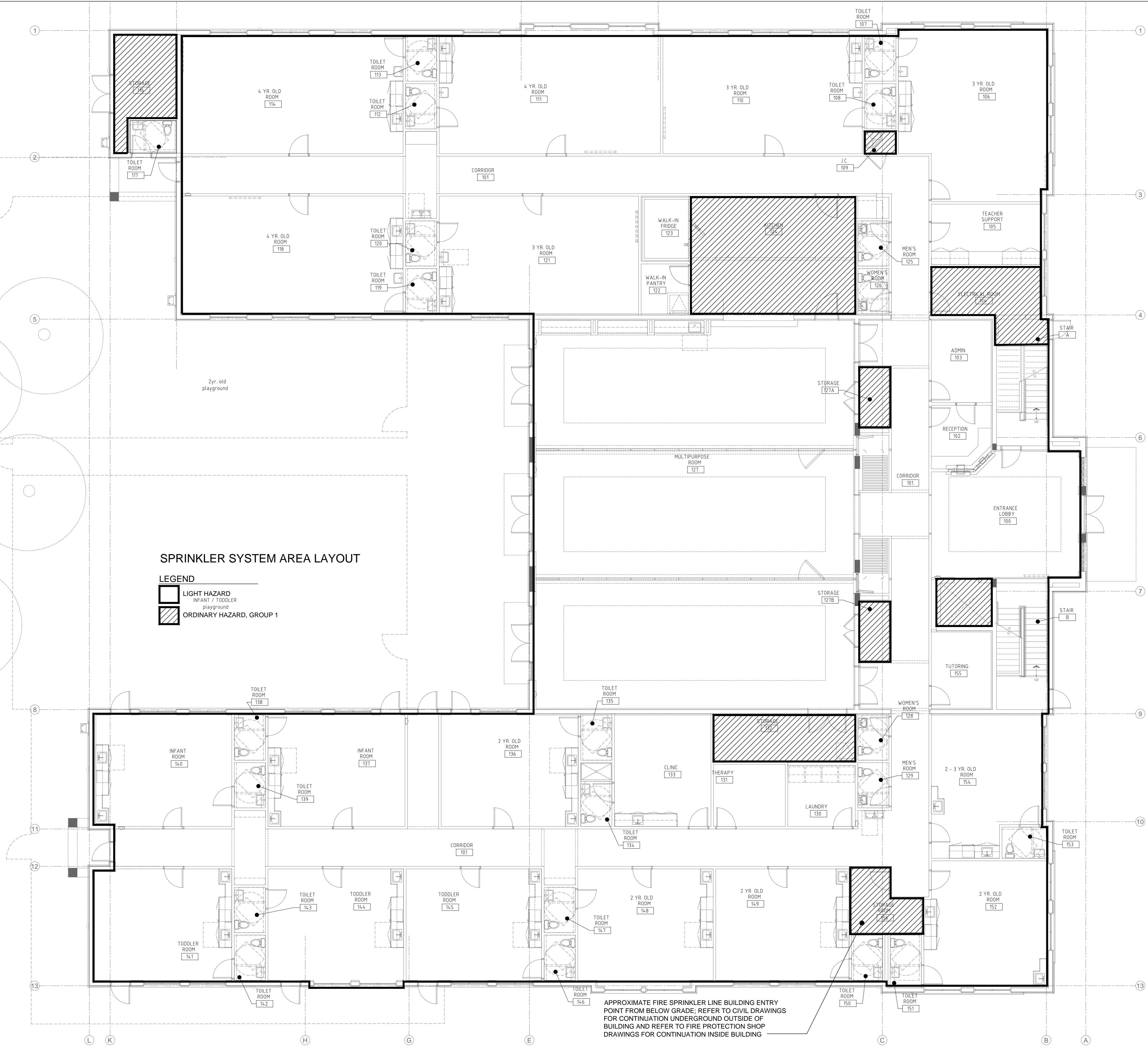
1 FIRST FLOOR FIRE PROTECTION PLAN SCALE: 1/8" = 1'-0"
