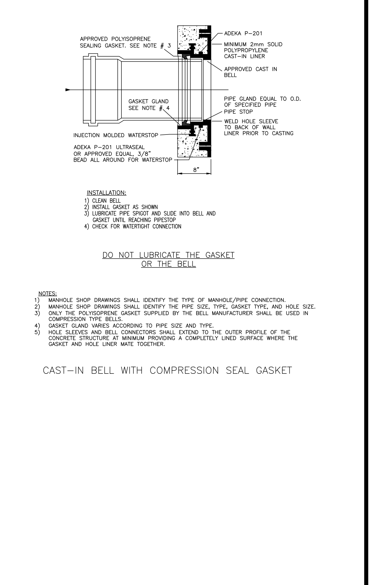
PIPE TO MANHOLE CONNECTION - TYPE "B" 22S
