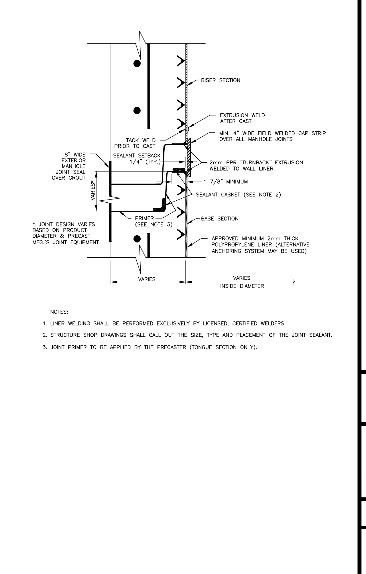
TURN BACK JOINT INSTALLED PRIOR TO CAST 27S
