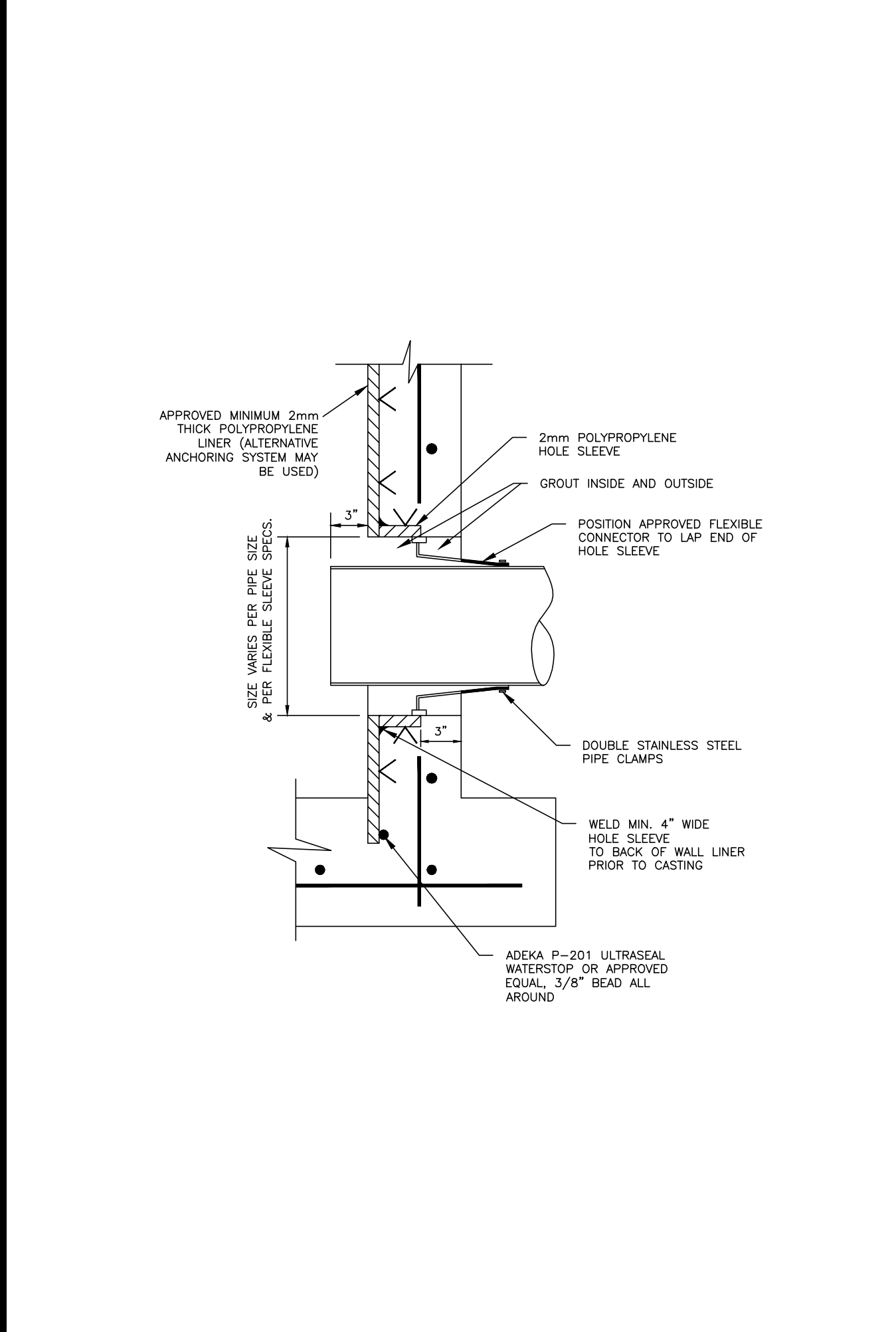
PIPE TO MANHOLE CONNECTION - TYPE "A" 21S
