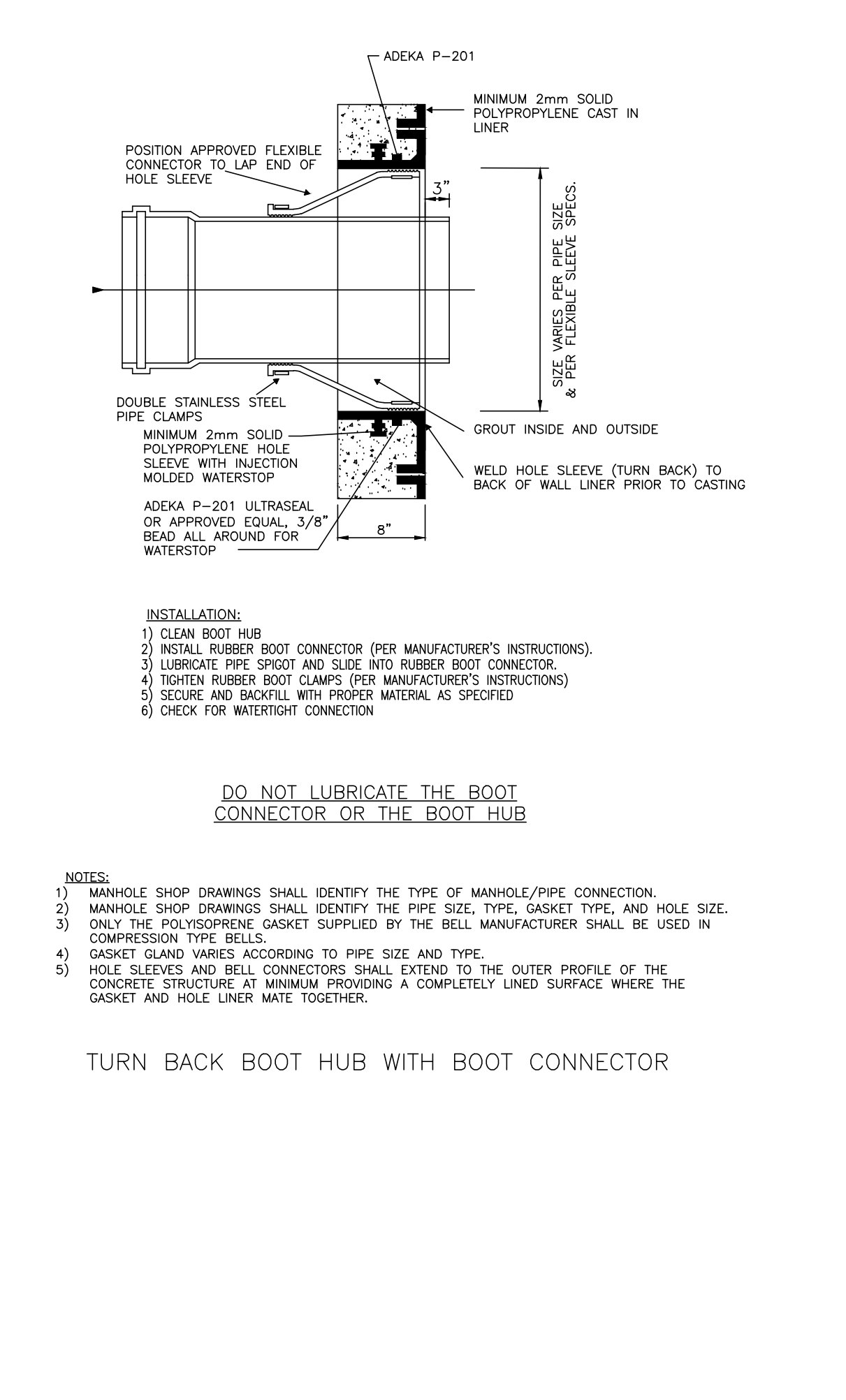
TURN BACK BOOT HUB WITH BOOT CONNECTOR 23S
