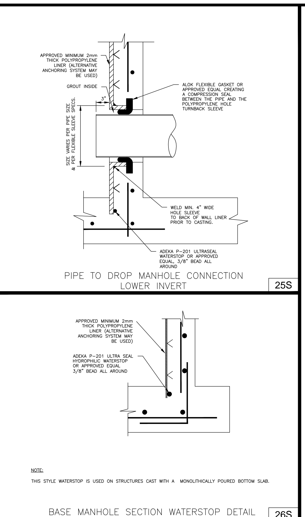
PIPE TO DROP MANHOLE CONNECTION LOWER INVERT 25S
