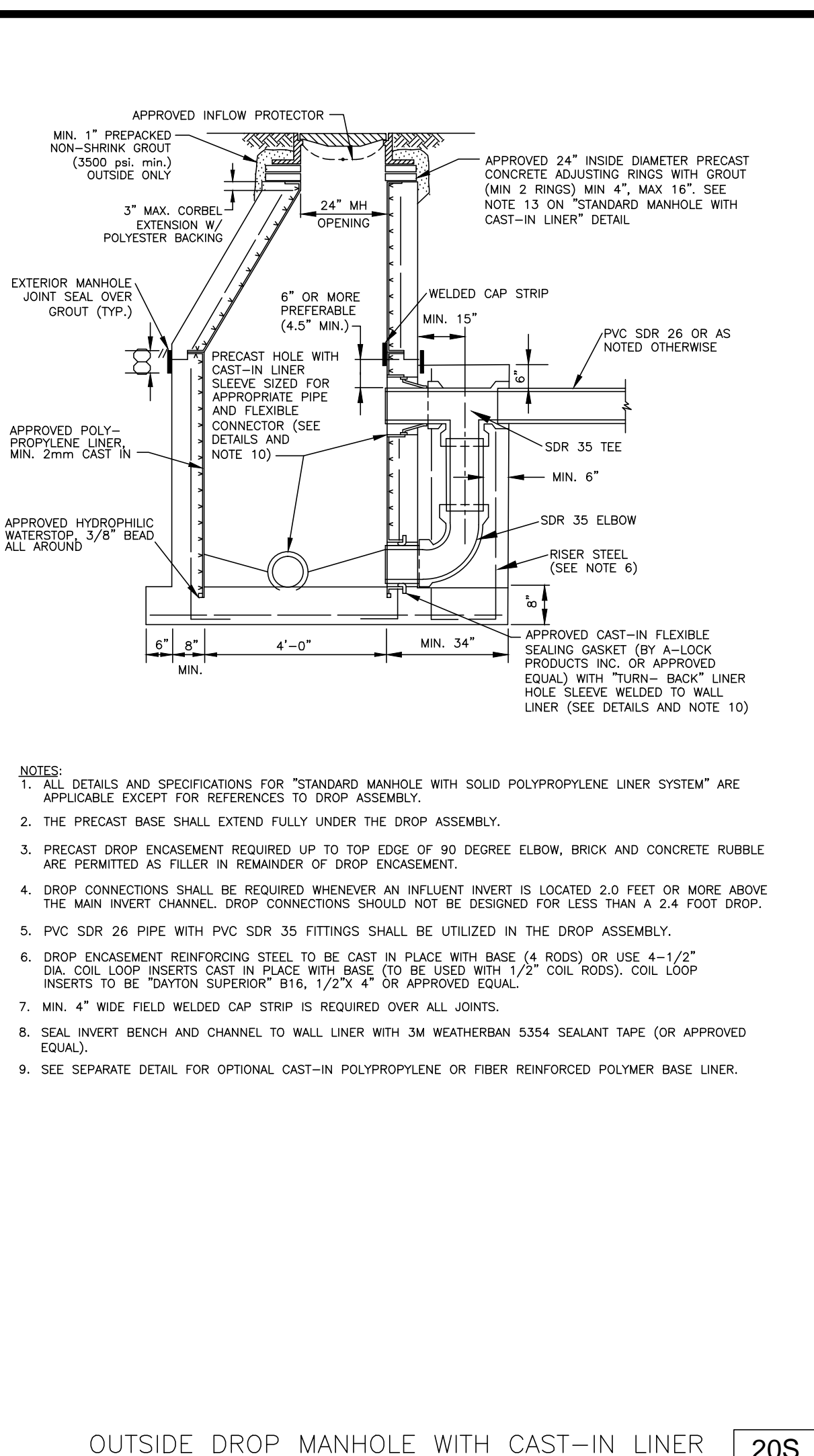
OUTSIDE DROP MANHOLE WITH CAST-IN LINER 20S
