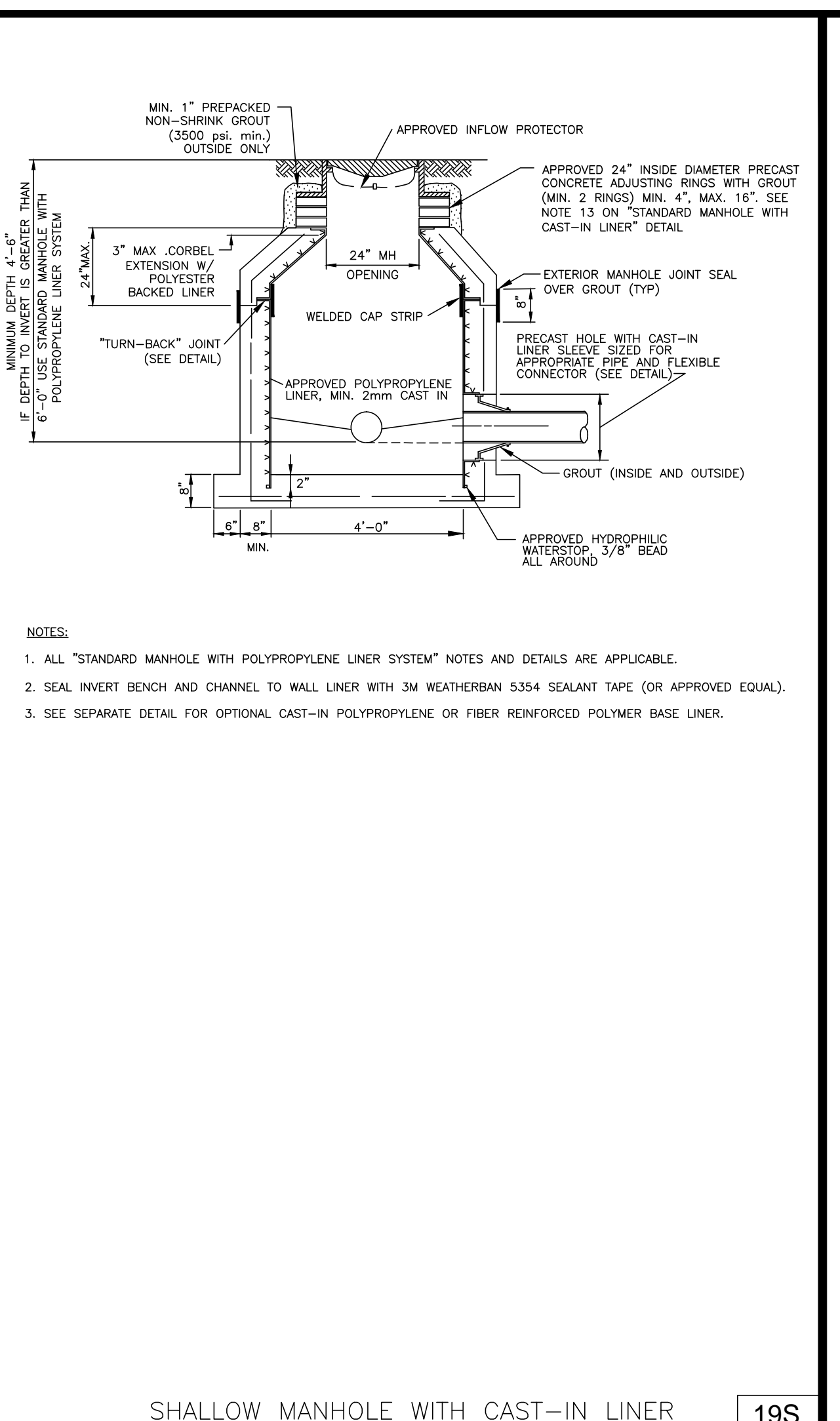
SHALLOW MANHOLE WITH CAST-IN LINER 19S
