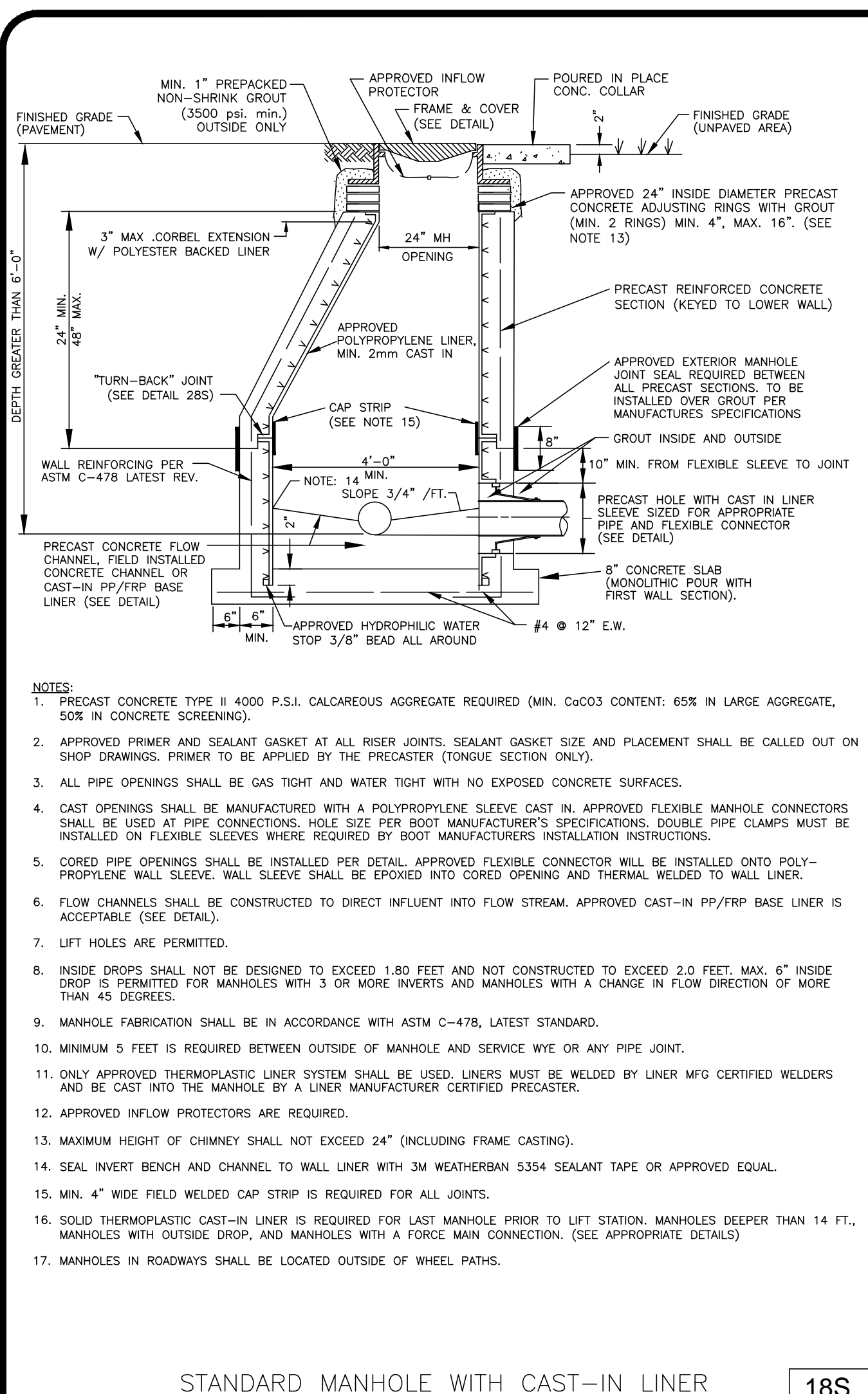
STANDARD MANHOLE WITH CAST-IN LINER 18S
