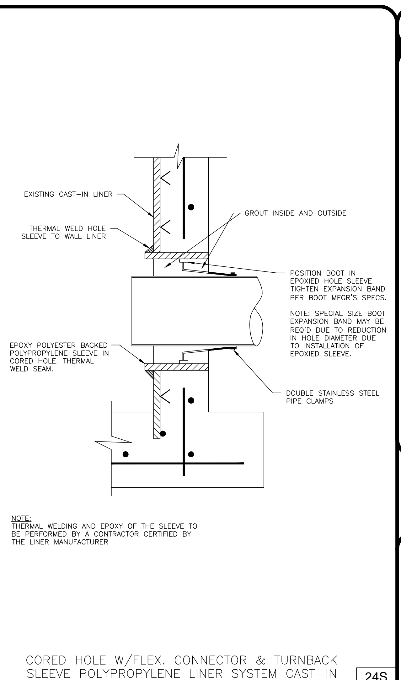
CORED HOLE W/FLEX. CONNECTOR & TURNBACK SLEEVE POLYPROPYLENE LINER SYSTEM CAST-IN 24S
