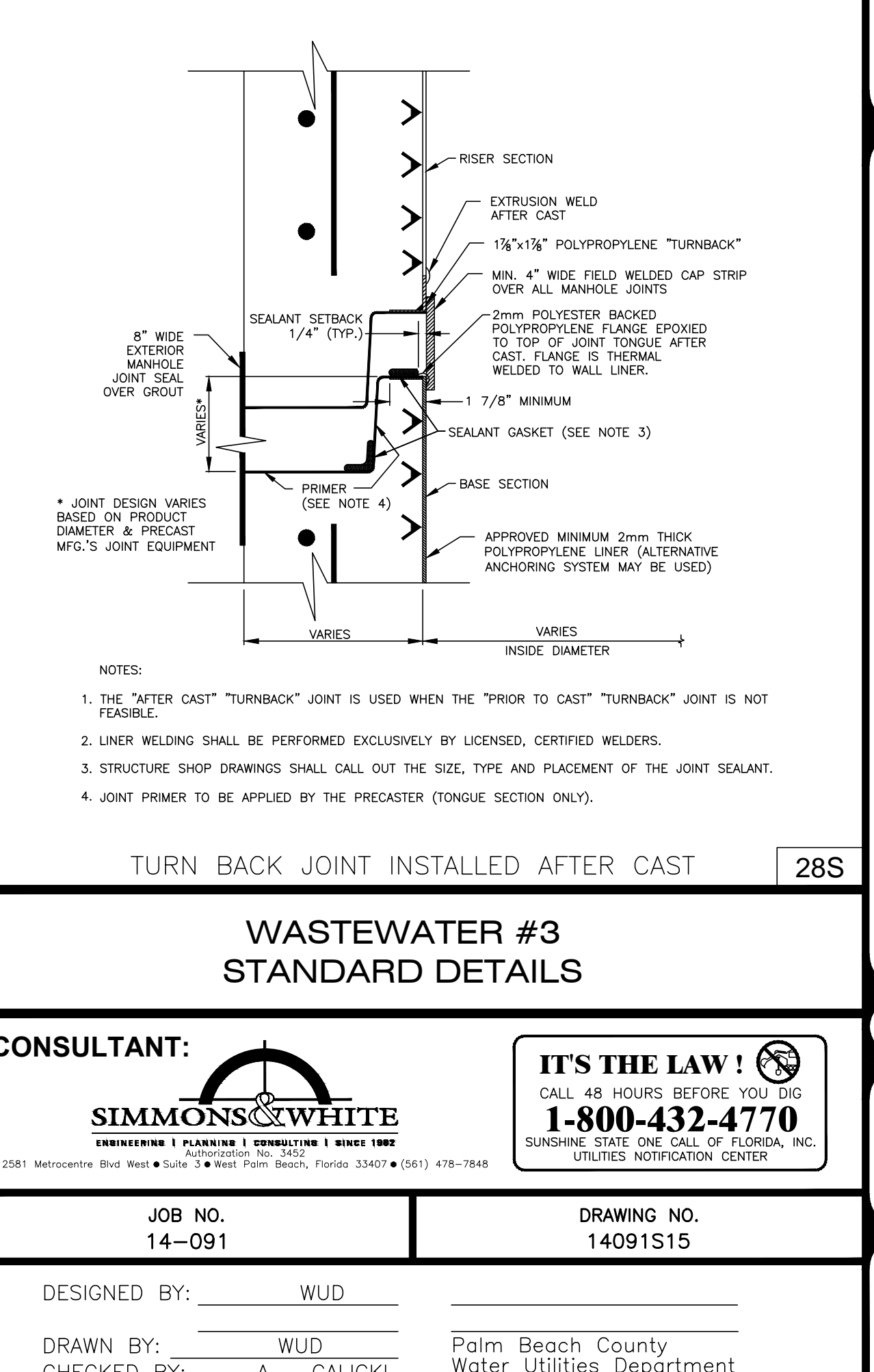
TURN BACK JOINT INSTALLED AFTER CAST 28S
