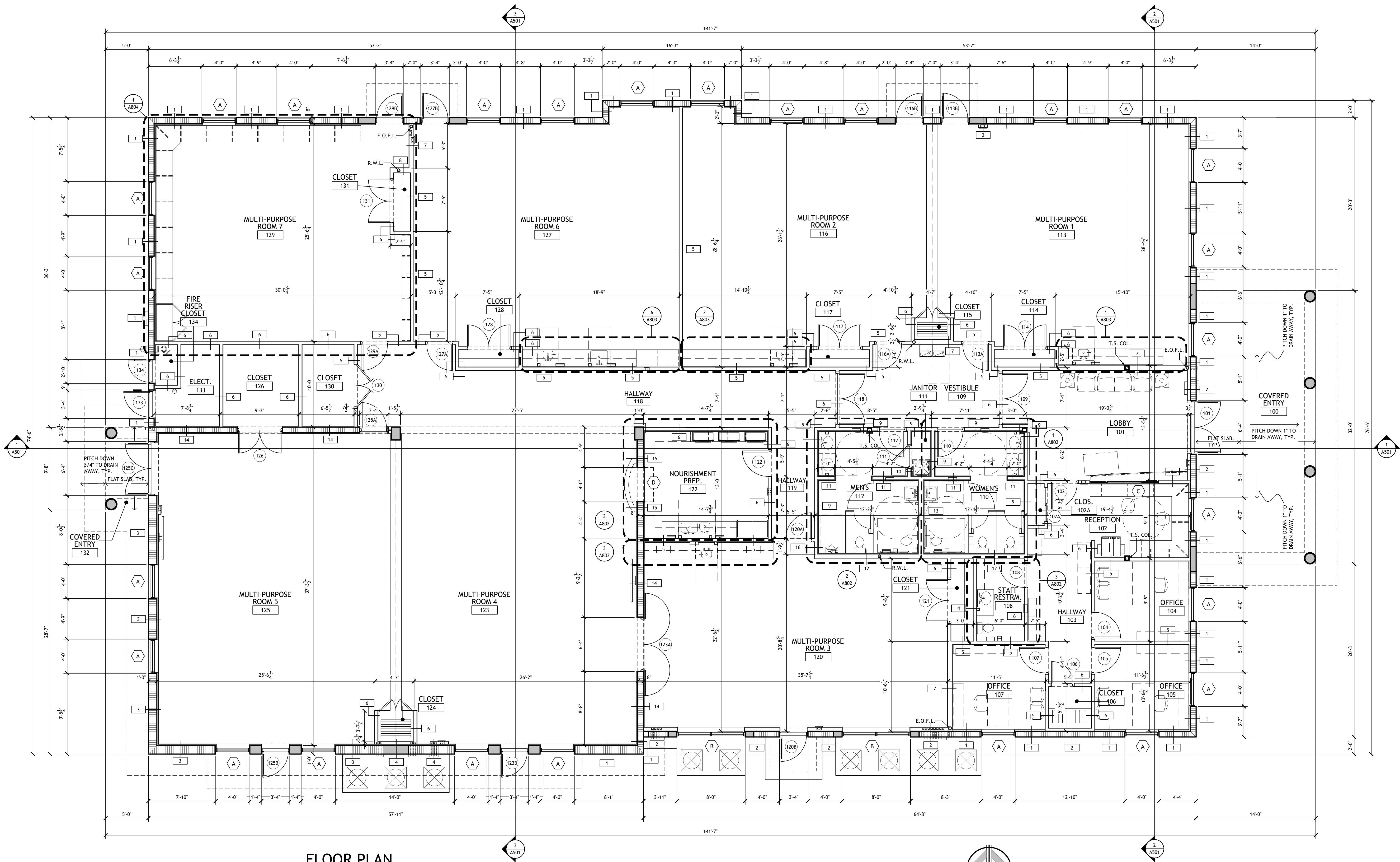
FLOOR PLAN
