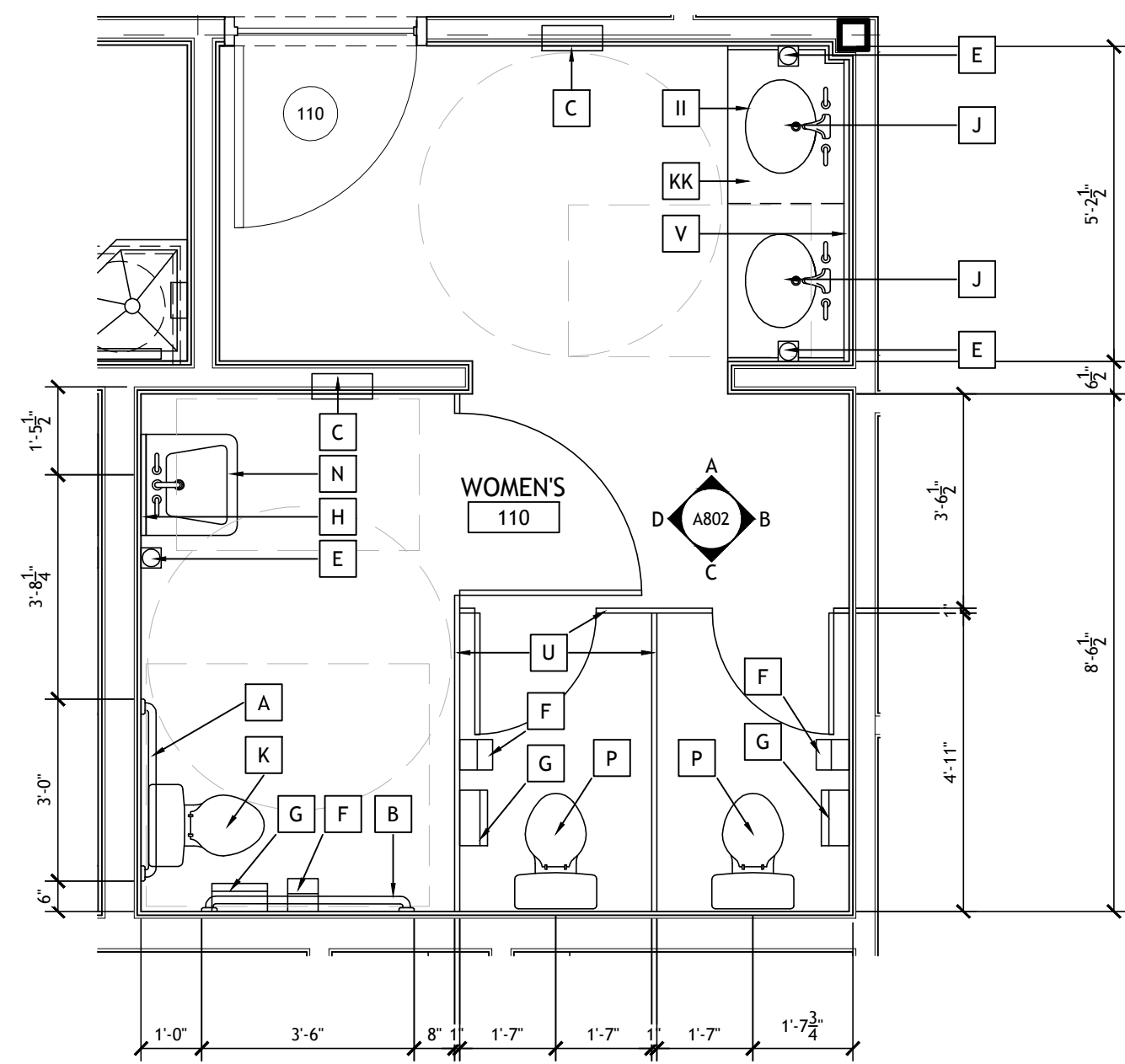
1 WOMEN'S - 110 A802 SCALE: 3/8" = 1'-0"
