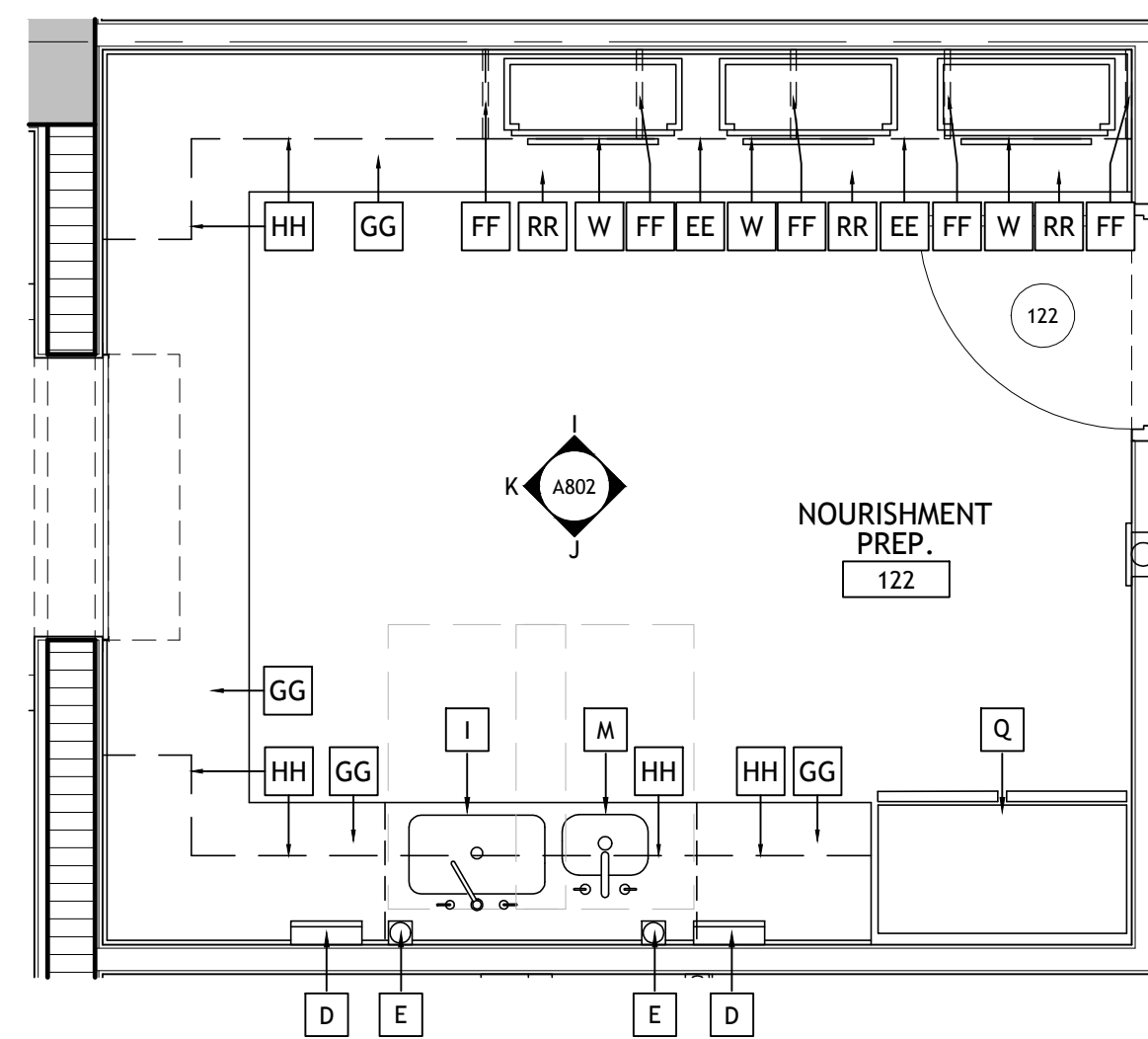
3 NOURISHMENT PREP. - 122 A802 SCALE: 3/8" = 1'-0"
