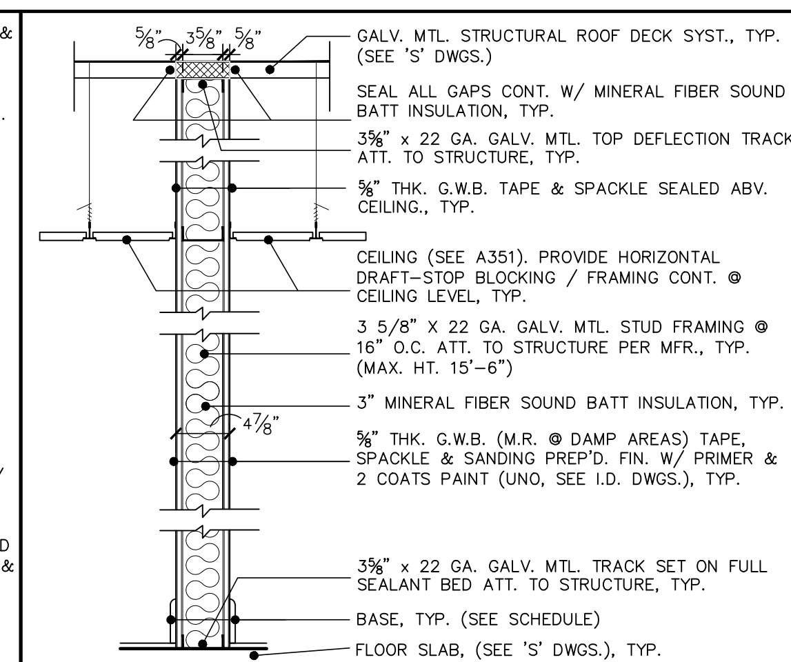
5 PARTITION TYPE 5 A903 NOT TO SCALE
