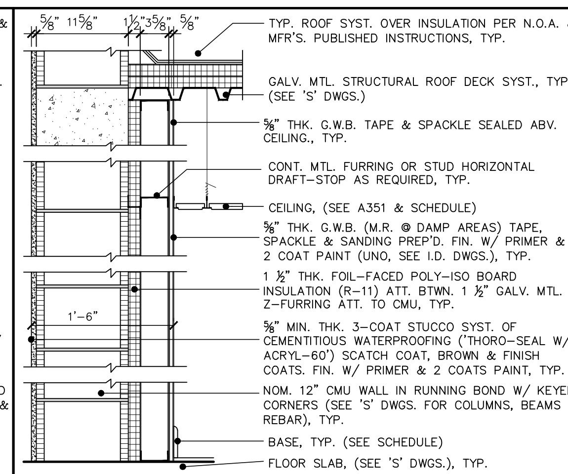
4 EXTERIOR C.M.U. WALL TYPE 4 A903 NOT TO SCALE
