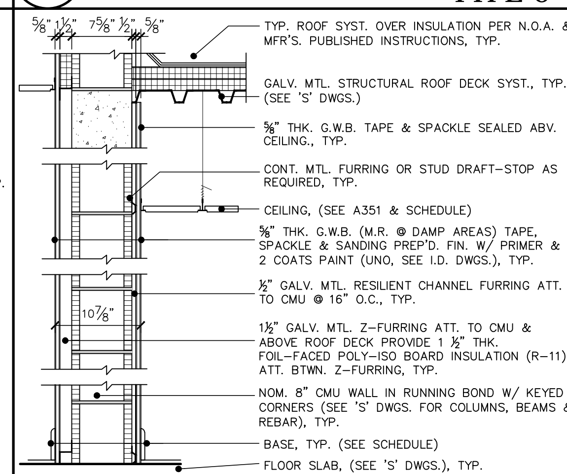
14 INTERIOR WALL TYPE 14 A903 NOT TO SCALE
