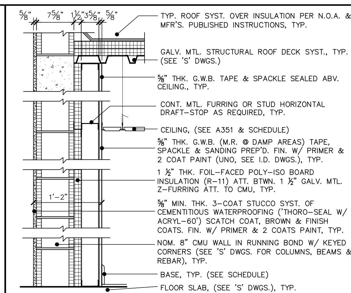
2 EXTERIOR C.M.U. WALL TYPE 2 A903 NOT TO SCALE
