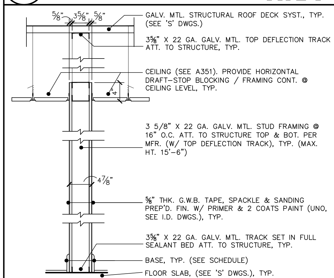
6 PARTITION TYPE 6 A903 NOT TO SCALE
