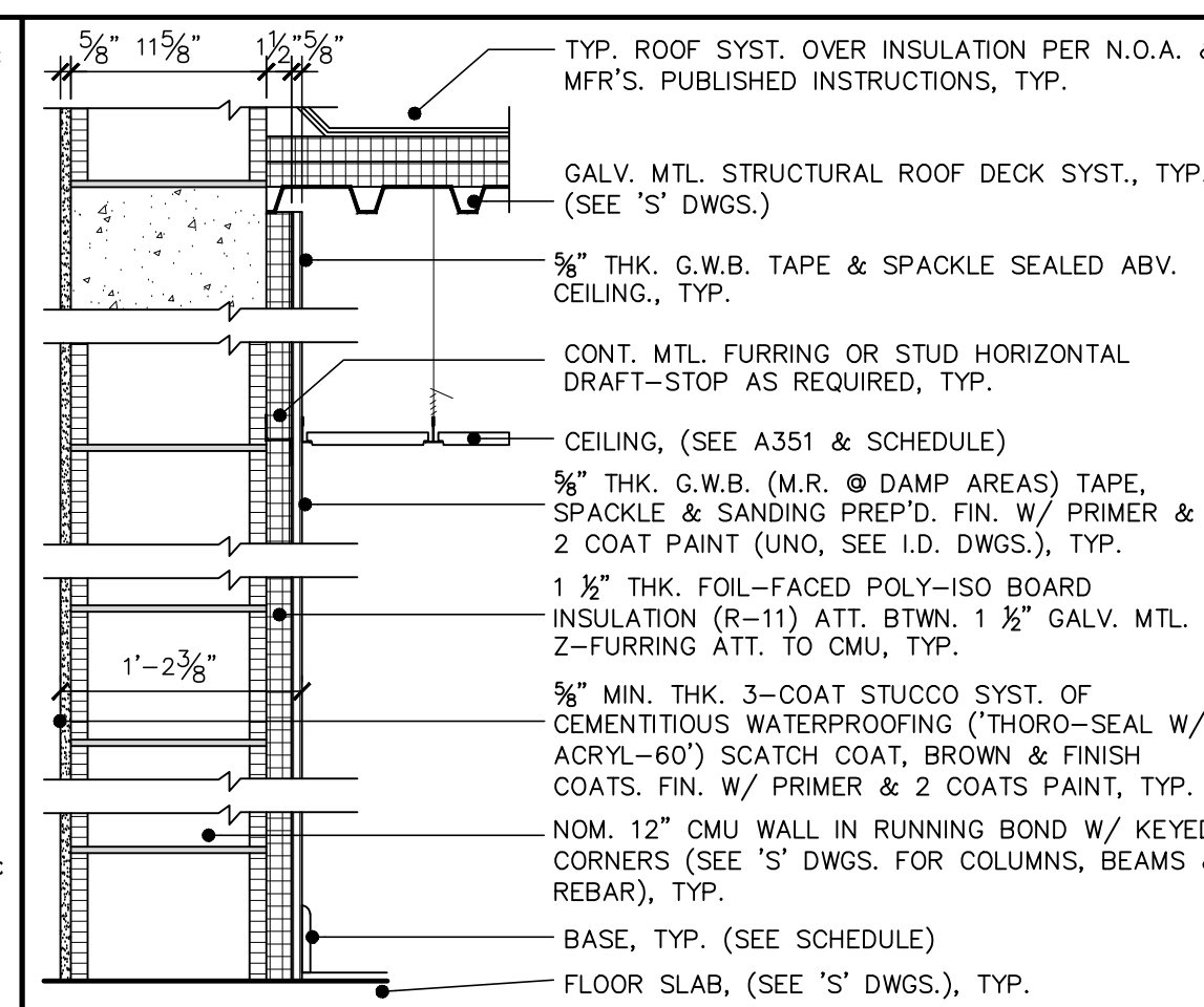
3 EXTERIOR C.M.U. WALL TYPE 3 A903 NOT TO SCALE
