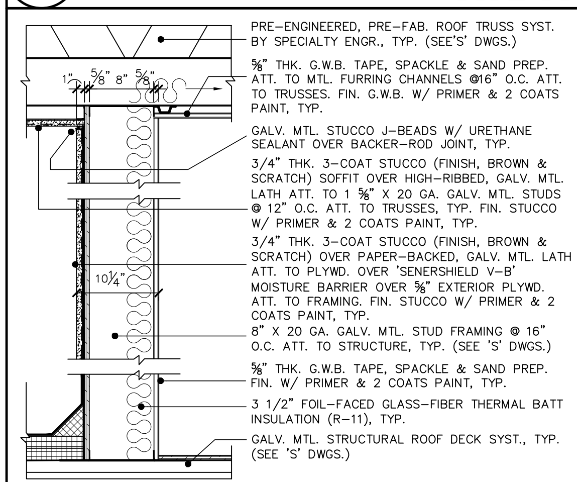
16 EXTERIOR C.M.U. WALL TYPE 16 A903 NOT TO SCALE
