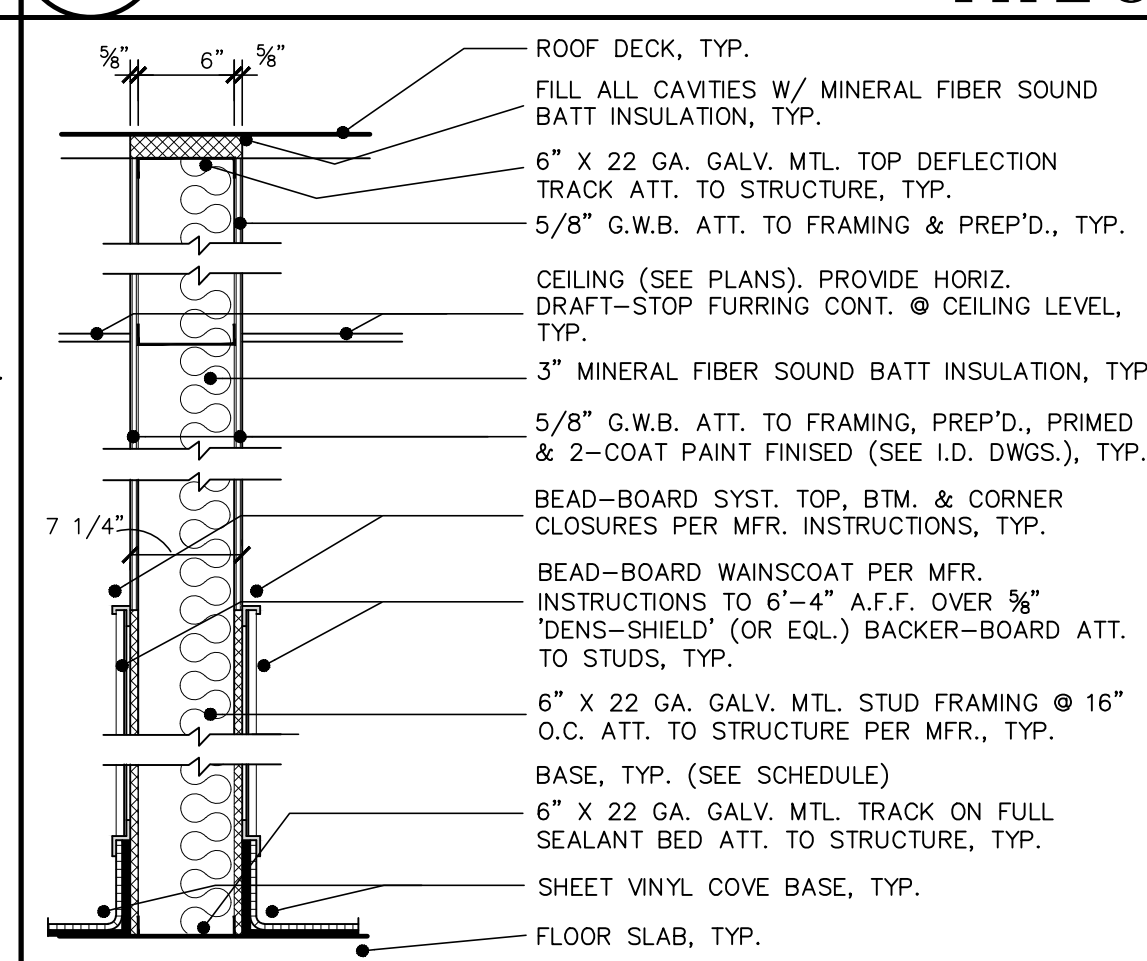
13 PARTITION TYPE 13 A903 NOT TO SCALE
