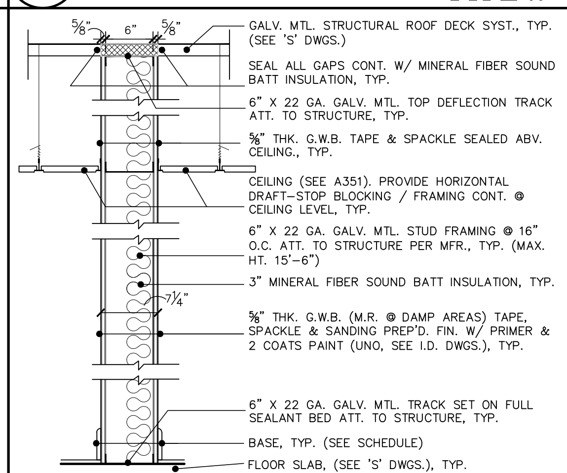
7 PARTITION TYPE 7 A903 NOT TO SCALE
