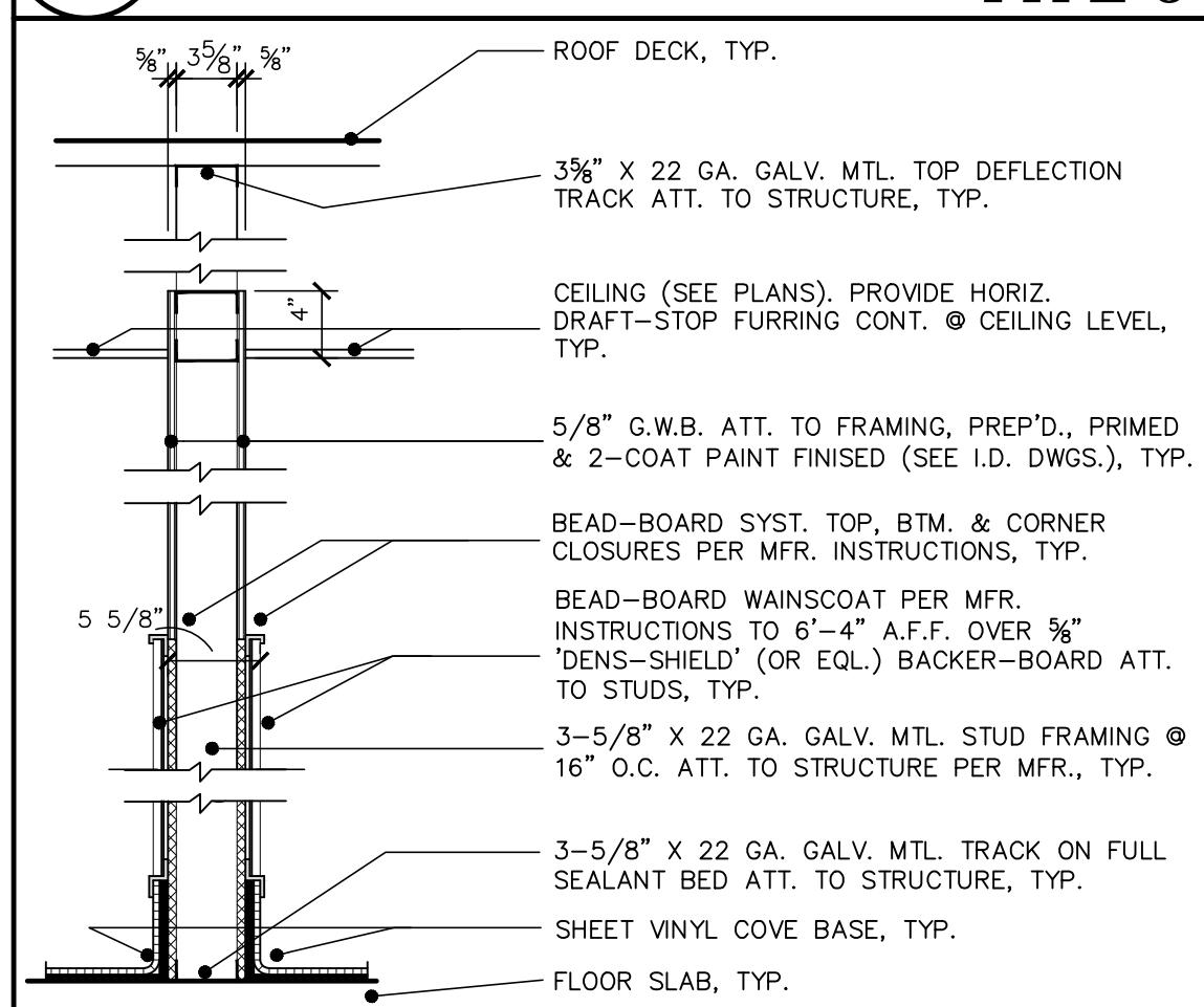
11 PARTITION TYPE 11 A903 NOT TO SCALE
