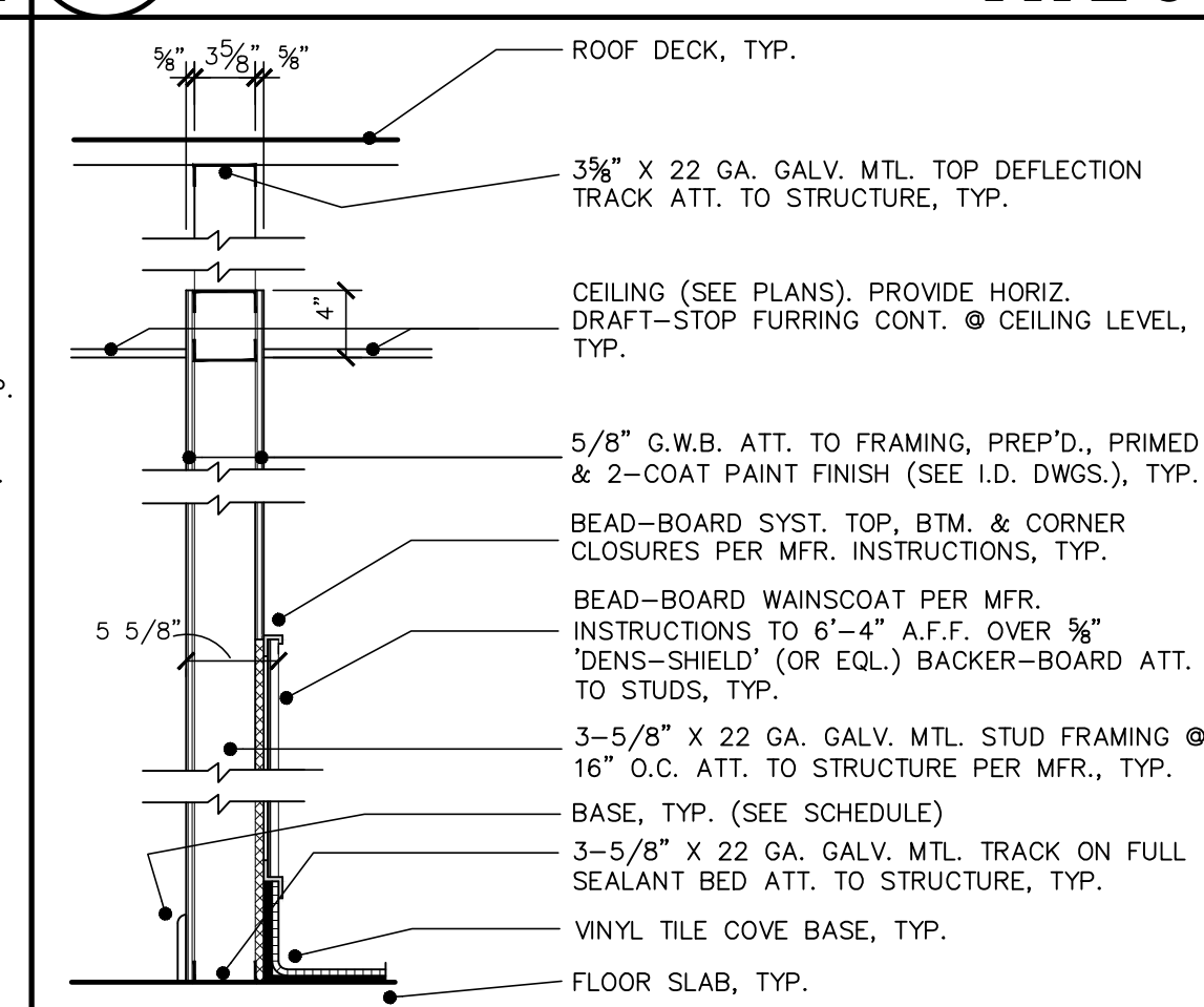
10 PARTITION TYPE 10 A903 NOT TO SCALE
