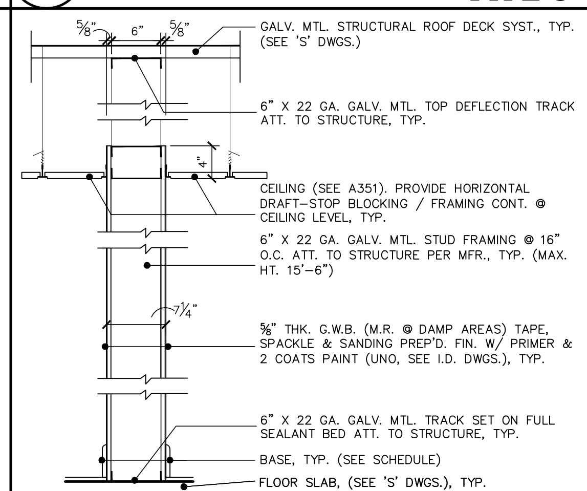
8 PARTITION TYPE 8 A903 NOT TO SCALE
