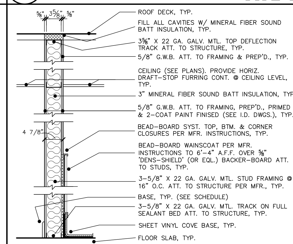
9 PARTITION TYPE 9 A903 NOT TO SCALE
