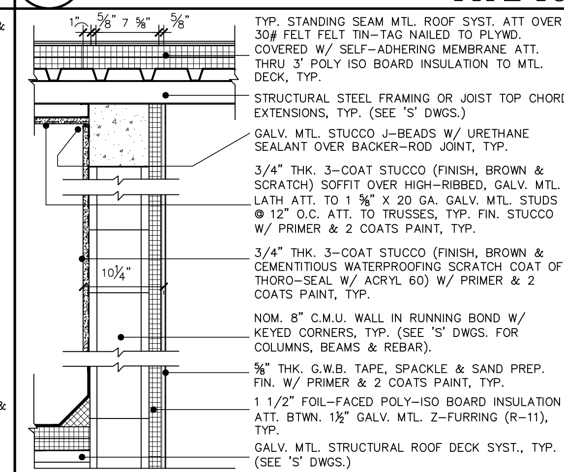
15 EXTERIOR C.M.U. WALL TYPE 15 A903 NOT TO SCALE
