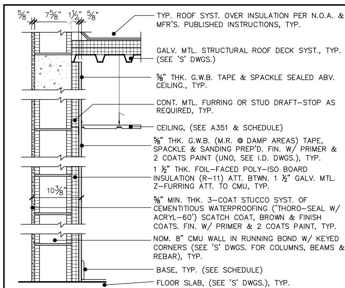
1 EXTERIOR C.M.U. WALL TYPE 1 A903 NOT TO SCALE
