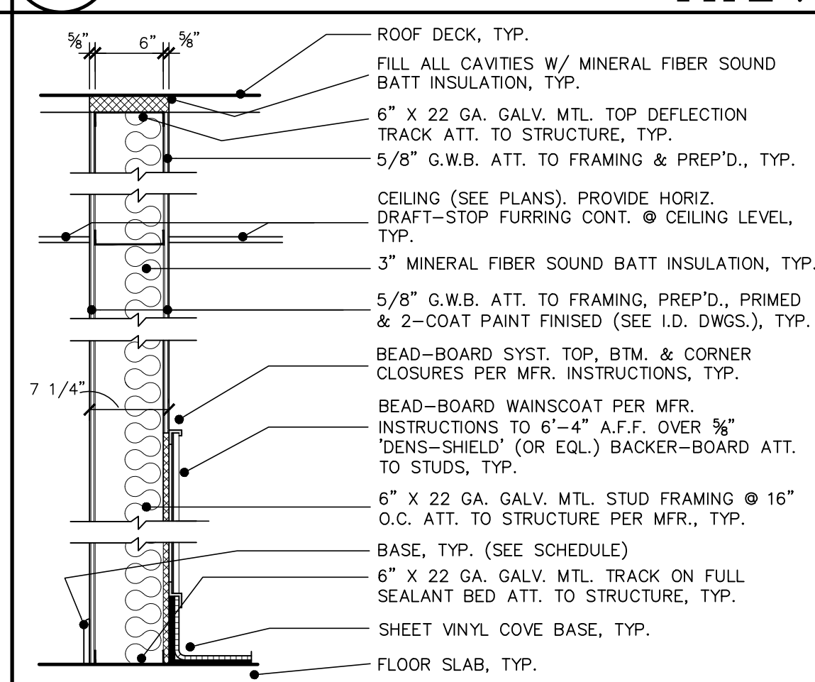
12 PARTITION TYPE 12 A903 NOT TO SCALE
