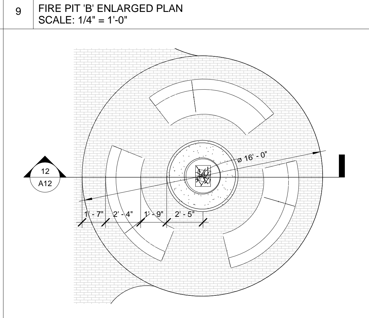
9 FIRE PIT 'B' ENLARGED PLAN SCALE: 1/4" = 1'-0"
