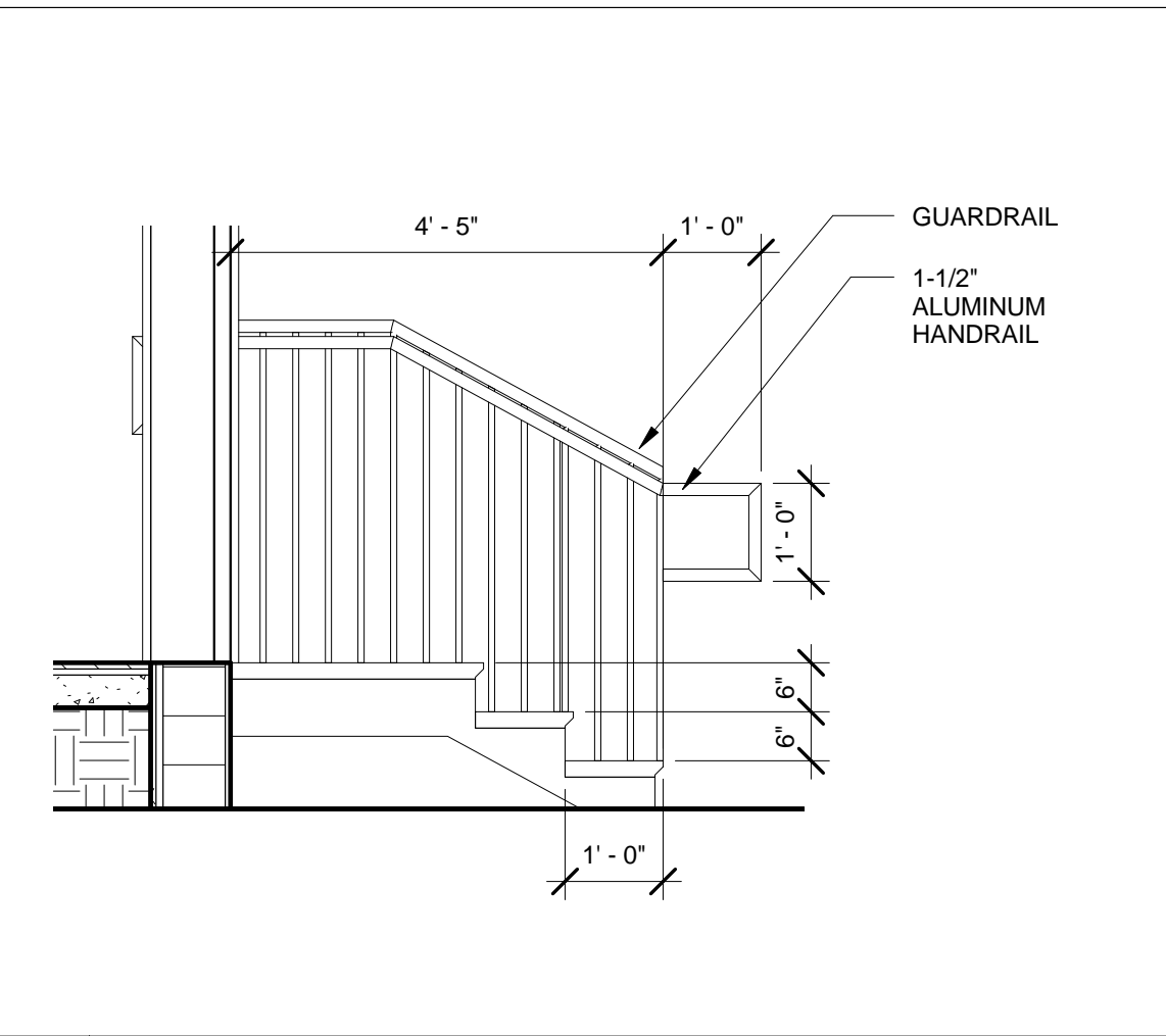
15 ALUMINUM STAIR SECTION DETAIL SCALE: 1/2" = 1'-0"
