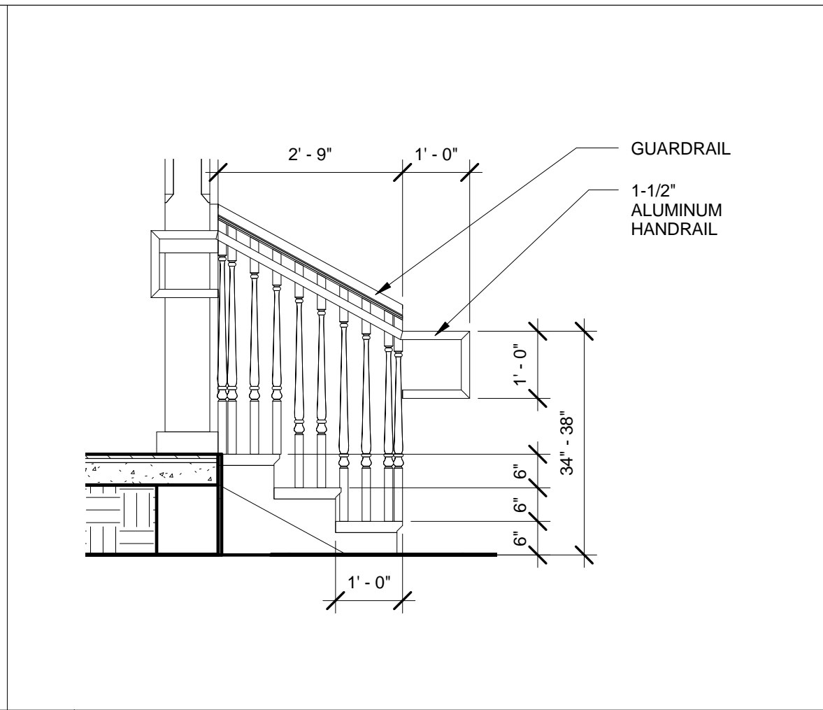
11 WOOD STAIR SECTION DETAIL SCALE: 1/2" = 1'-0"
