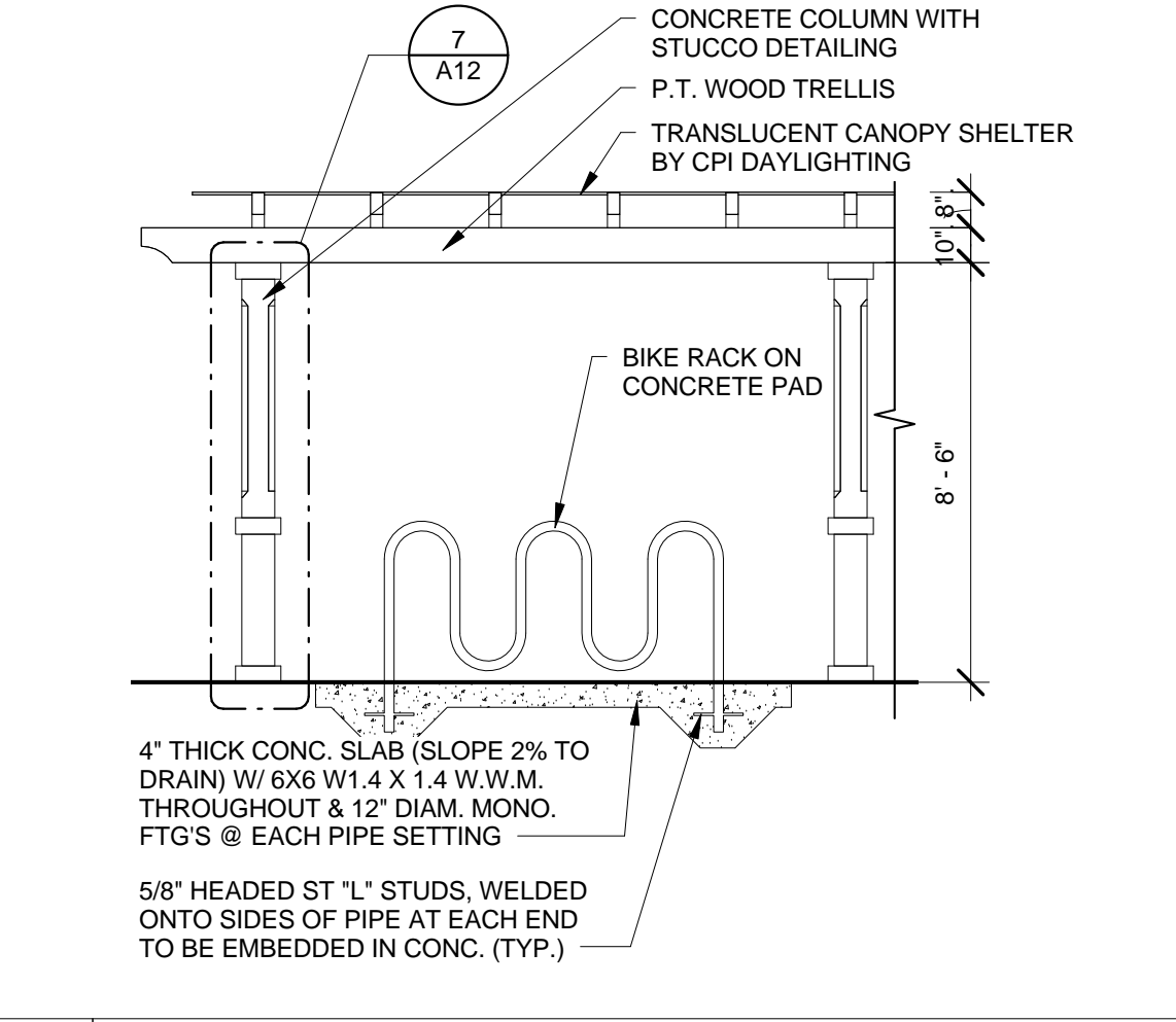
6 PARTIAL TRELLIS ELEVATION SCALE: 1/4" = 1'-0"
