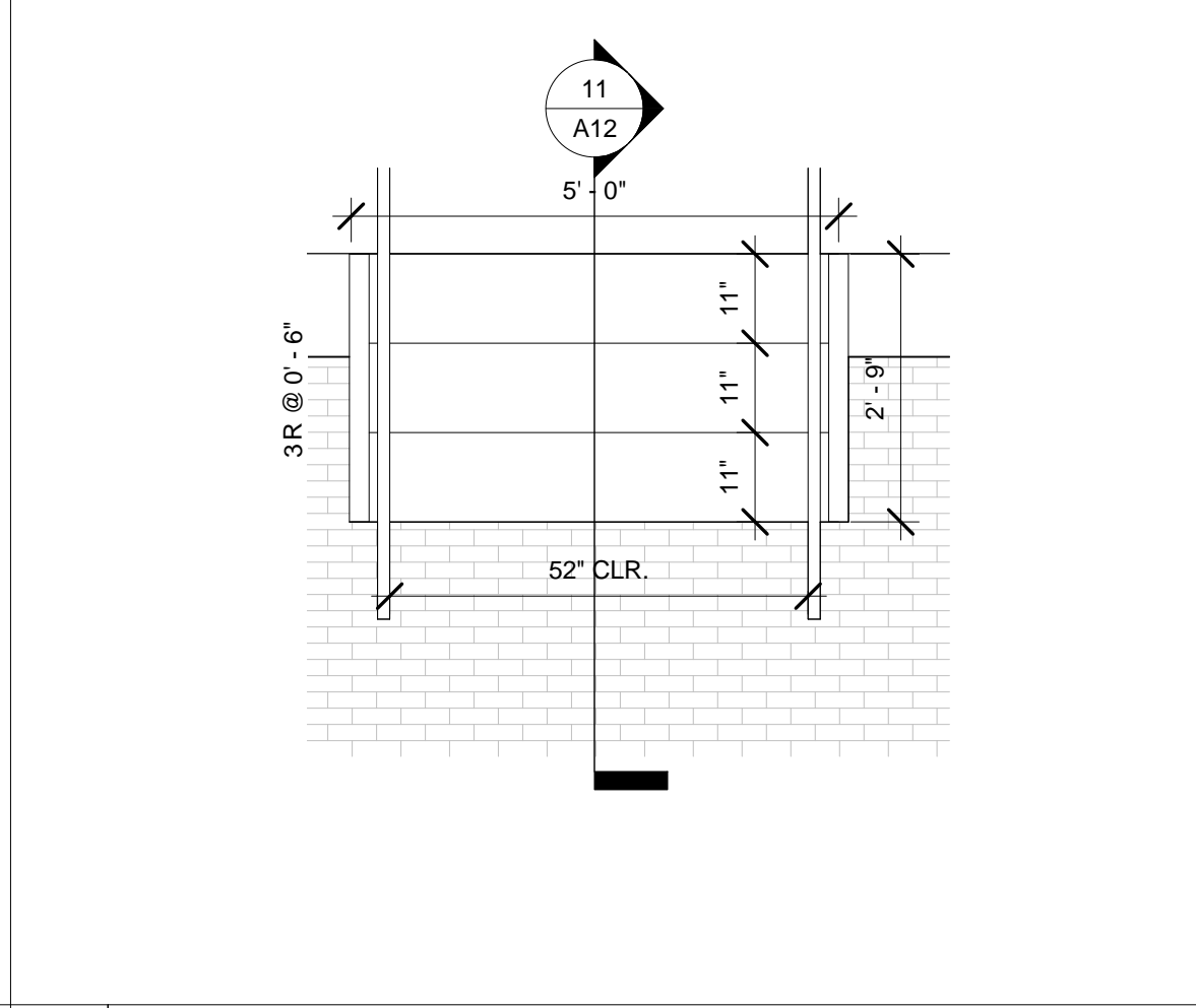
10 WOOD STAIR ENLARGED PLAN SCALE: 1/2" = 1'-0"
