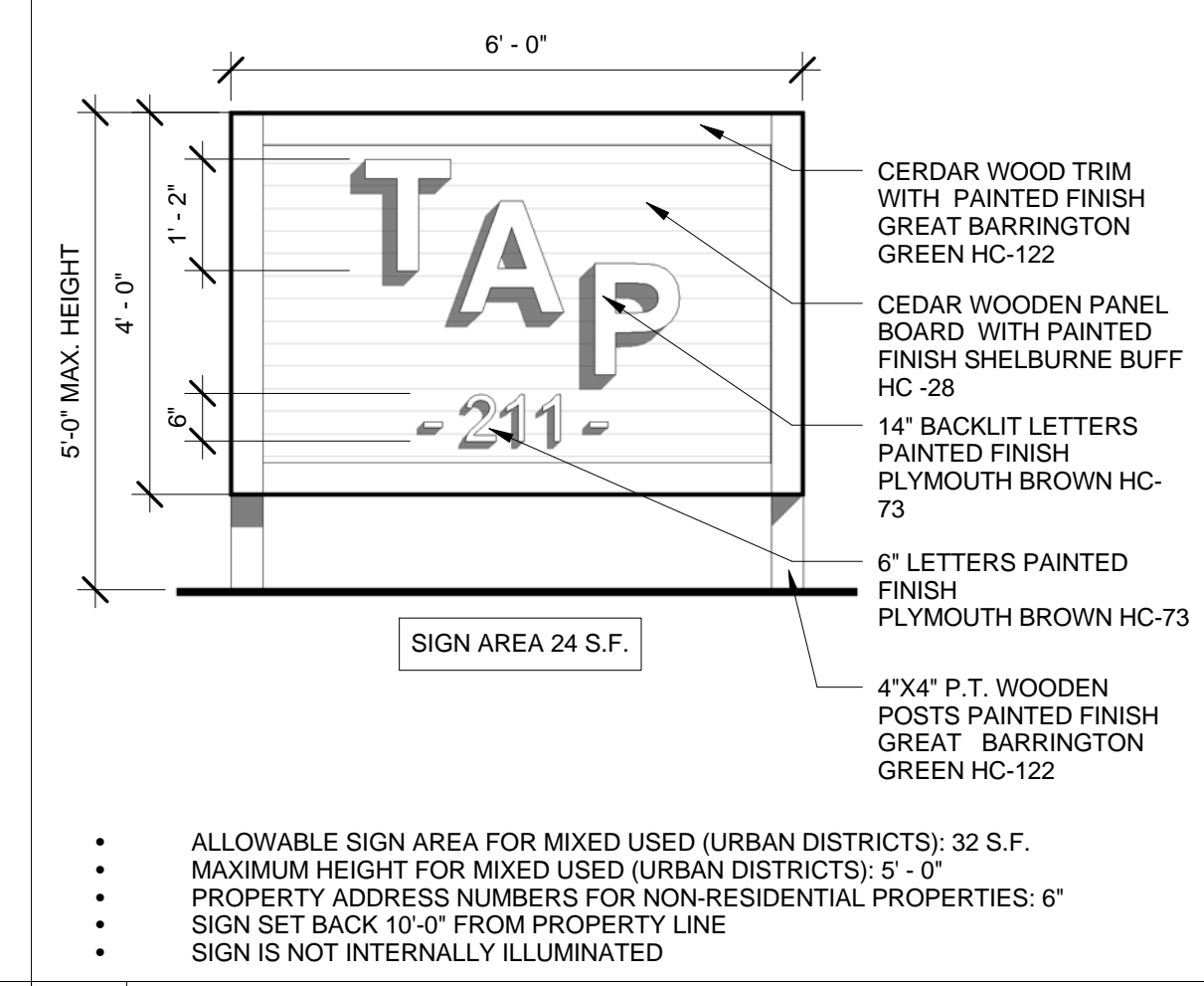
2 BUILDING SIGN ELEVATION SCALE: 1/2" = 1'-0"
