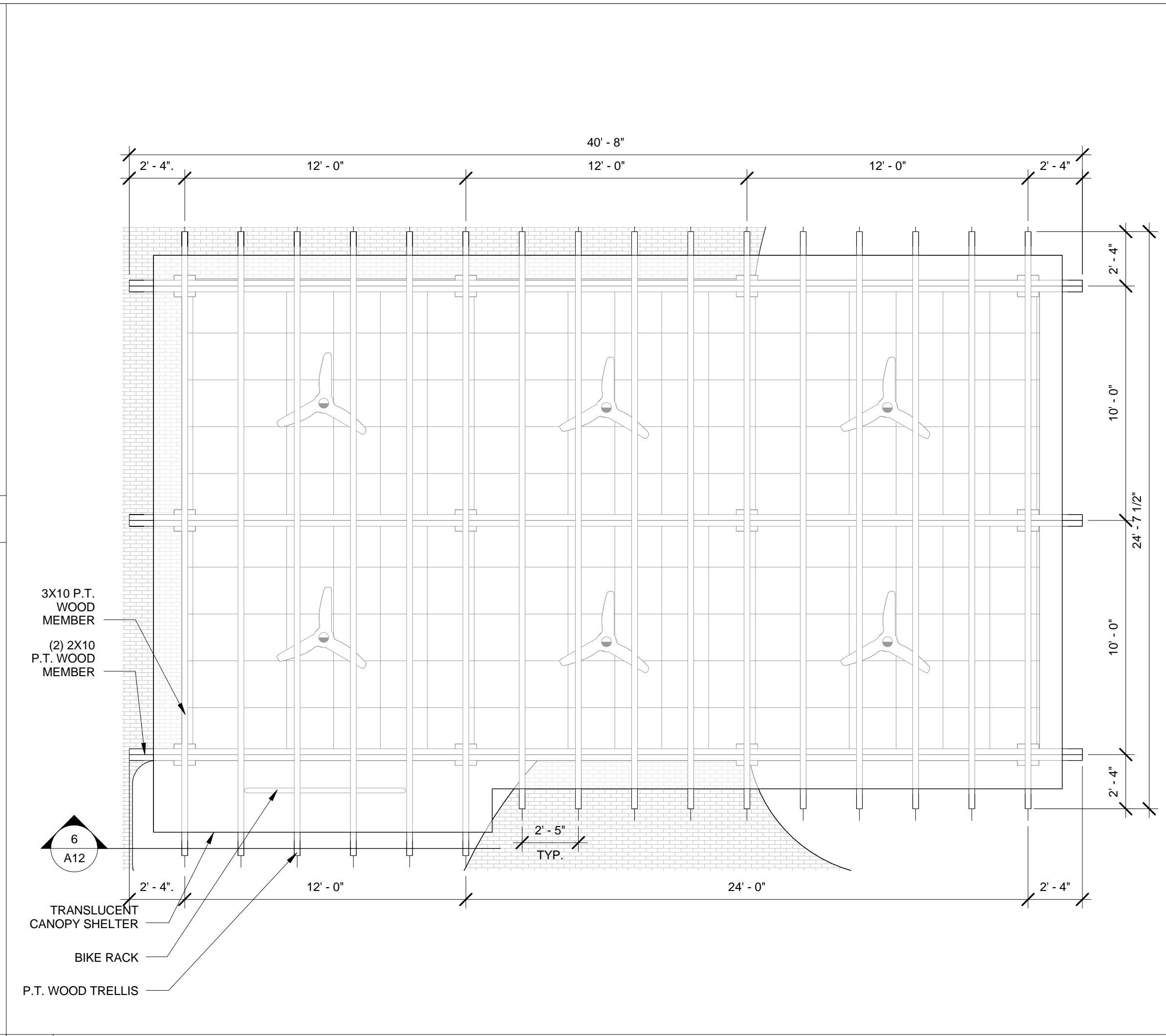
3 TRELLIS ENLARGED PLAN SCALE: 1/4" = 1'-0"
