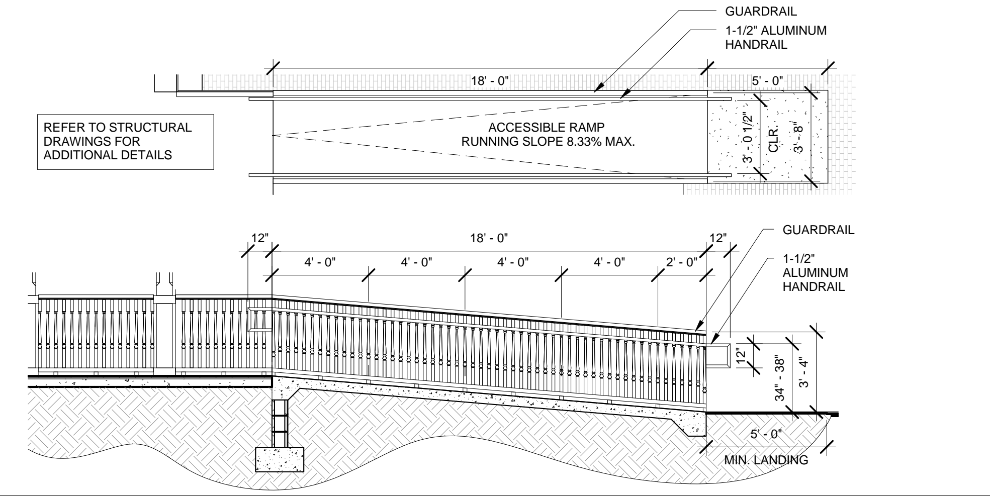
5 RAMP ENLARGED PLAN AND SECTION DETAIL SCALE: 1/4" = 1'-0"
