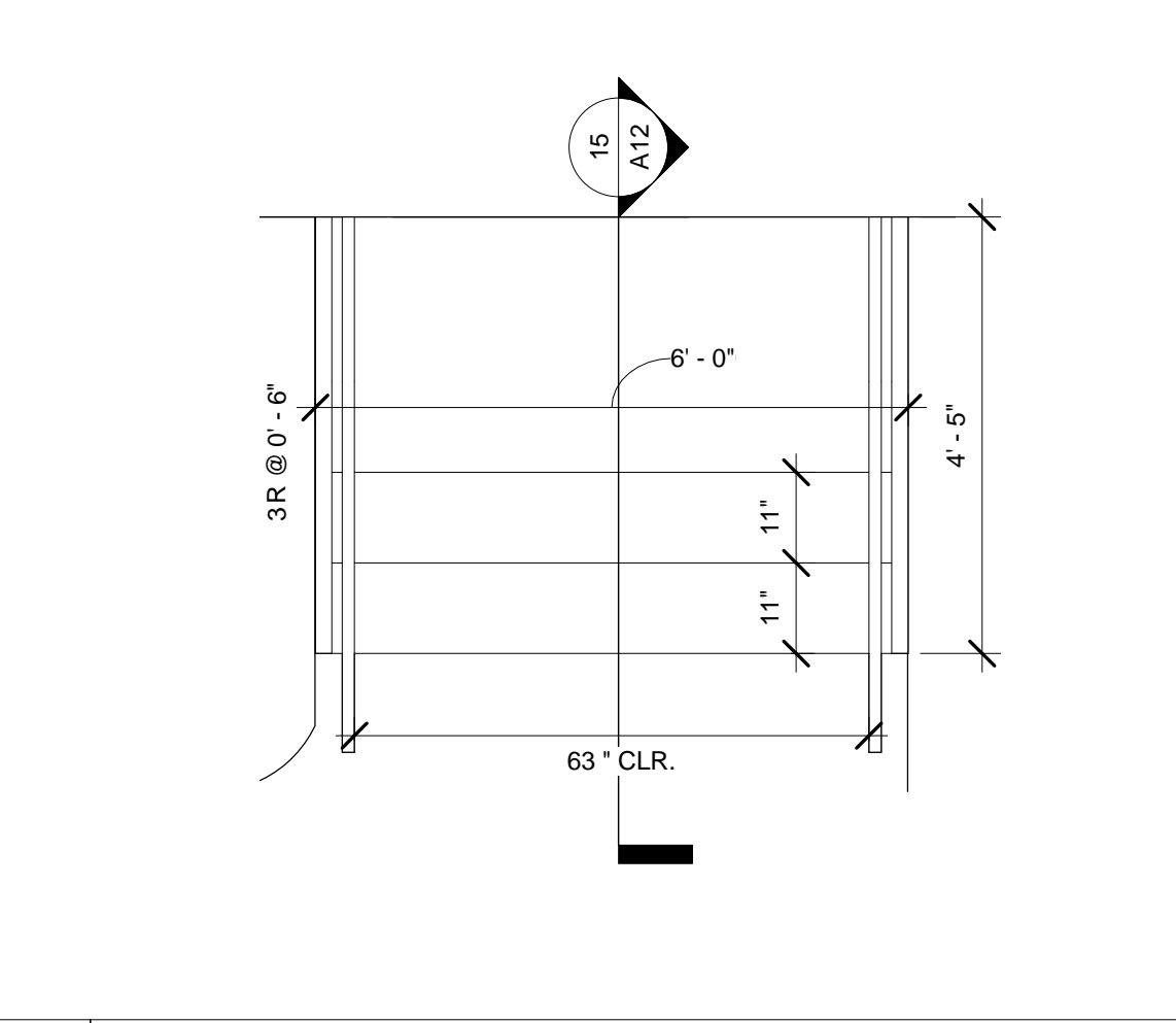
14 ALUMINUM STAIR ENLARGED PLAN SCALE: 1/2" = 1'-0"
