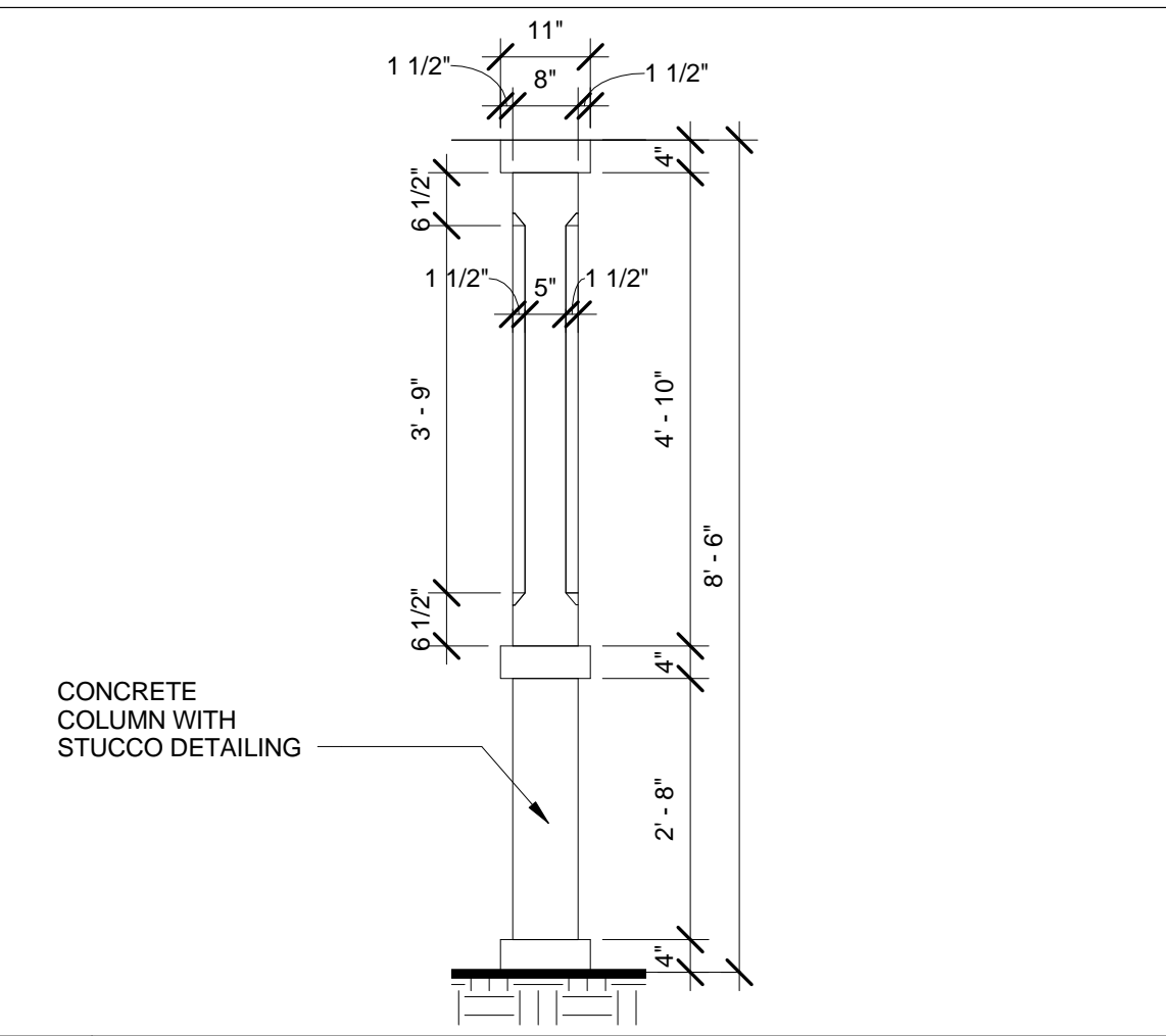
7 TRELLIS COLUMN DETAIL SCALE: 1/2" = 1'-0"
