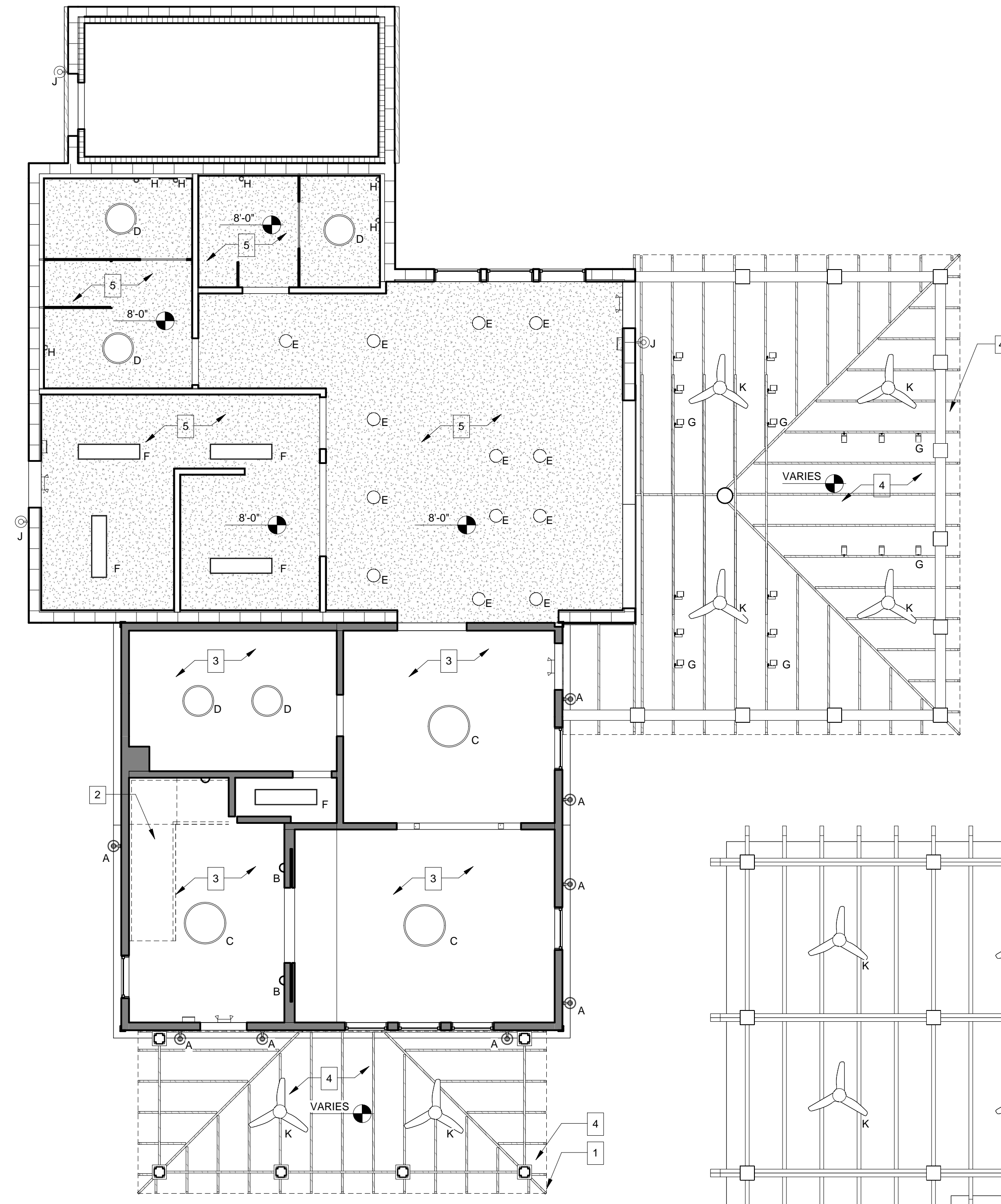
1 1ST FLOOR REFLECTED CEILING PLAN SCALE: 3/16"=1'-0"
