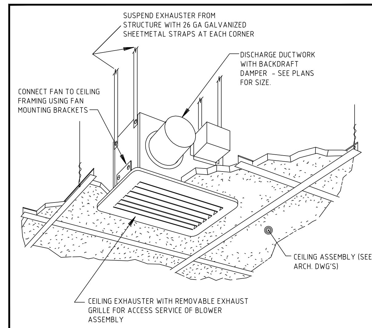
DETAIL NO. 3 CEILING MOUNTED FAN DETAIL NOT TO SCALE
