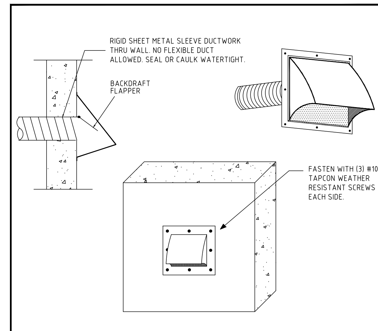
DETAIL NO. 4 WALL CAP DETAIL NOT TO SCALE
