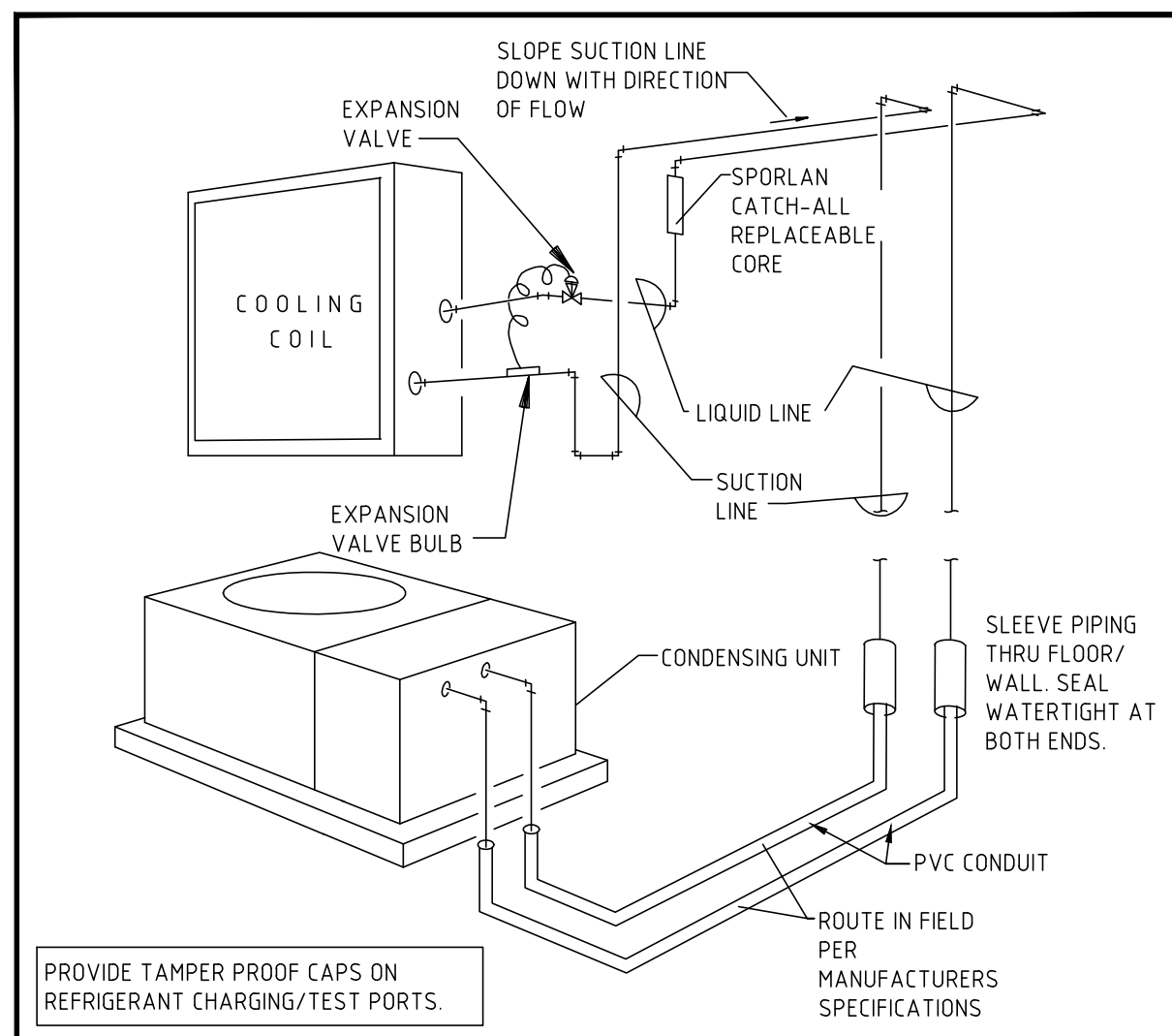
DETAIL NO. 1 REFRIGERANT PIPING DETAIL NOT TO SCALE
