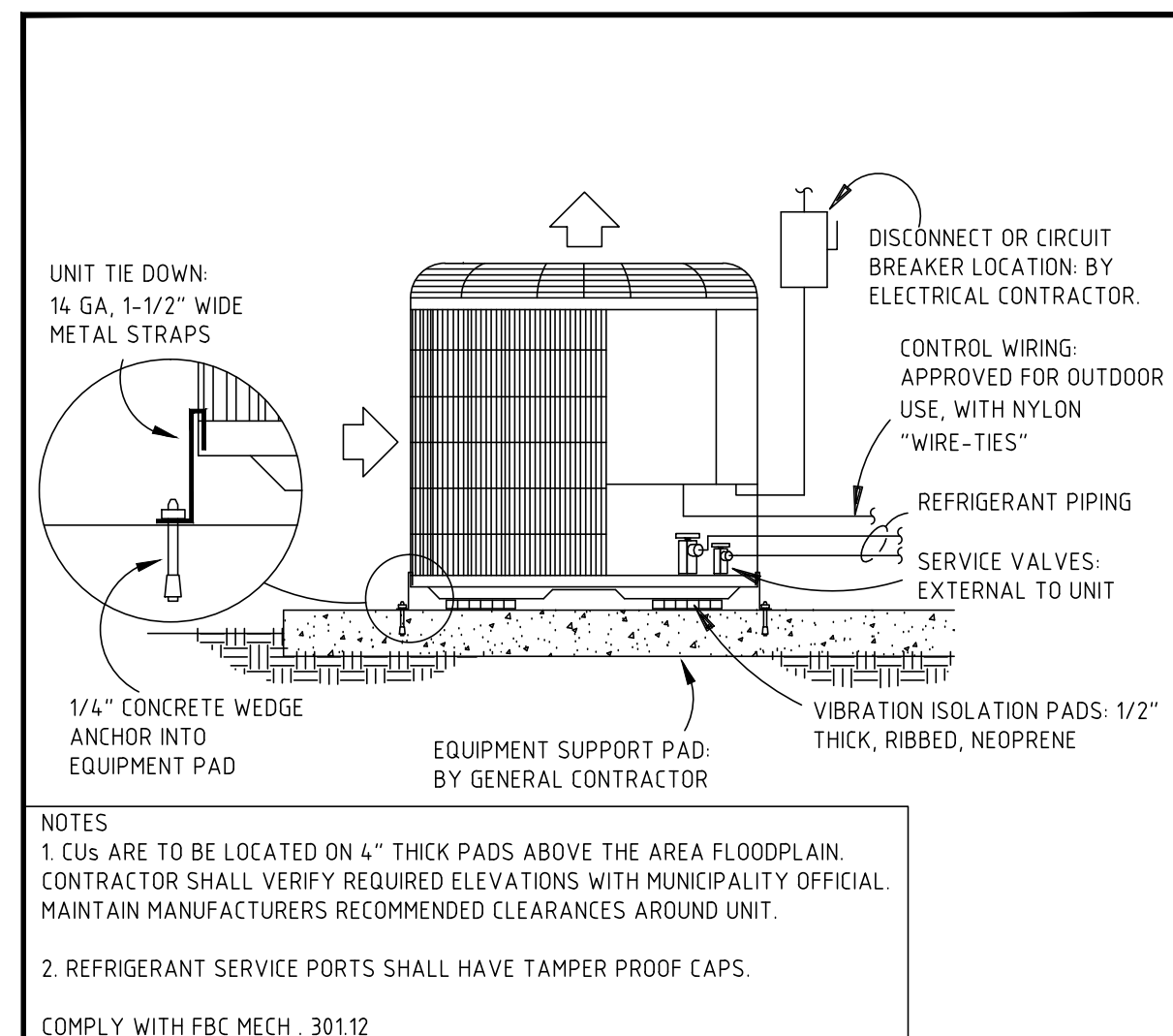
DETAIL NO. 2 CONDENSER MOUNTING DETAIL NOT TO SCALE
