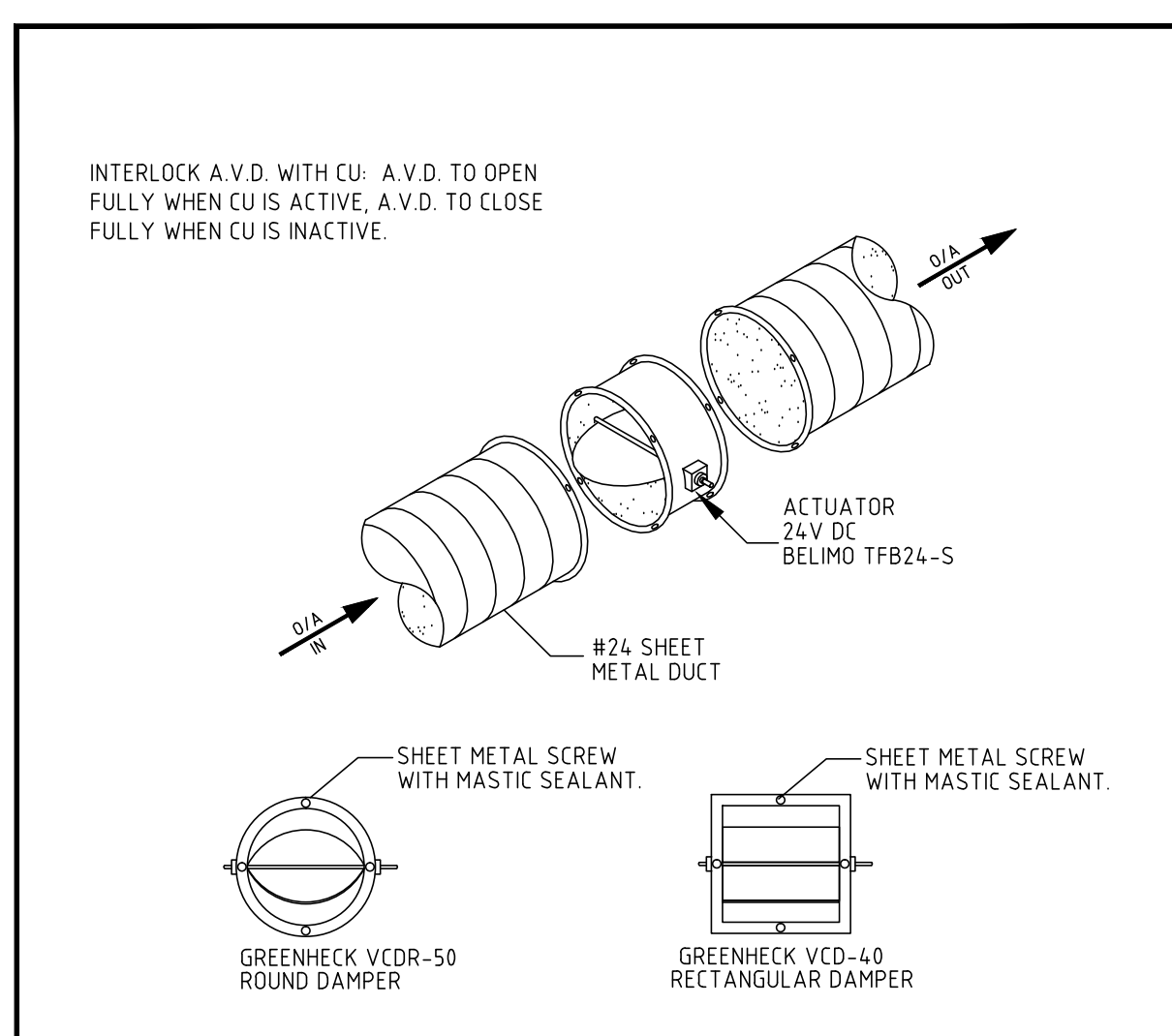
DETAIL NO. 7 AUTOMATIC VOLUME DAMPER (A.V.D) DETAIL NOT TO SCALE
