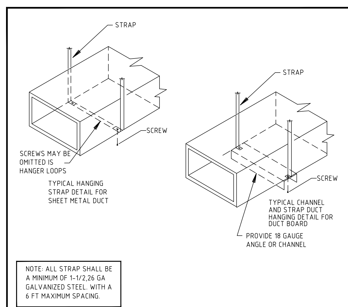
DETAIL NO. 8 METHODS OF HANGING RIGID DUCT DETAIL NOT TO SCALE
