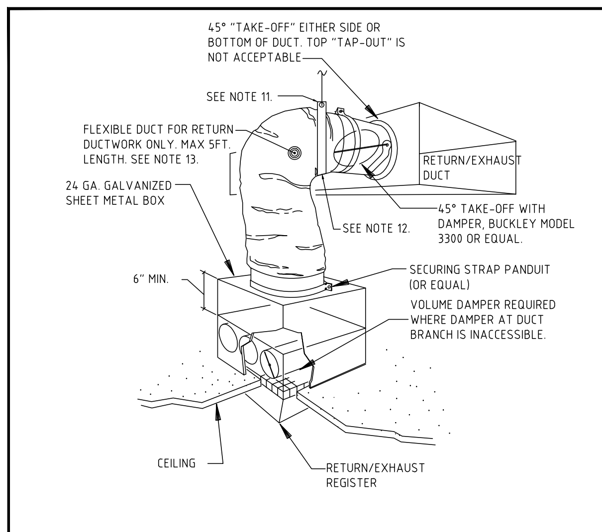
DETAIL NO. 5 DUCTWORK CONNECTION TO RETURN/EXHAUST GRILLE (FLEX DUCT) DETAIL NOT TO SCALE
