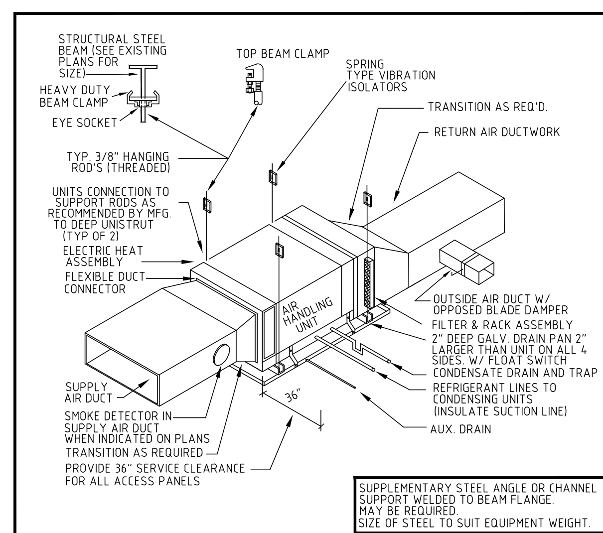
DETAIL NO. 9 AIR HANDLER DETAIL NOT TO SCALE
