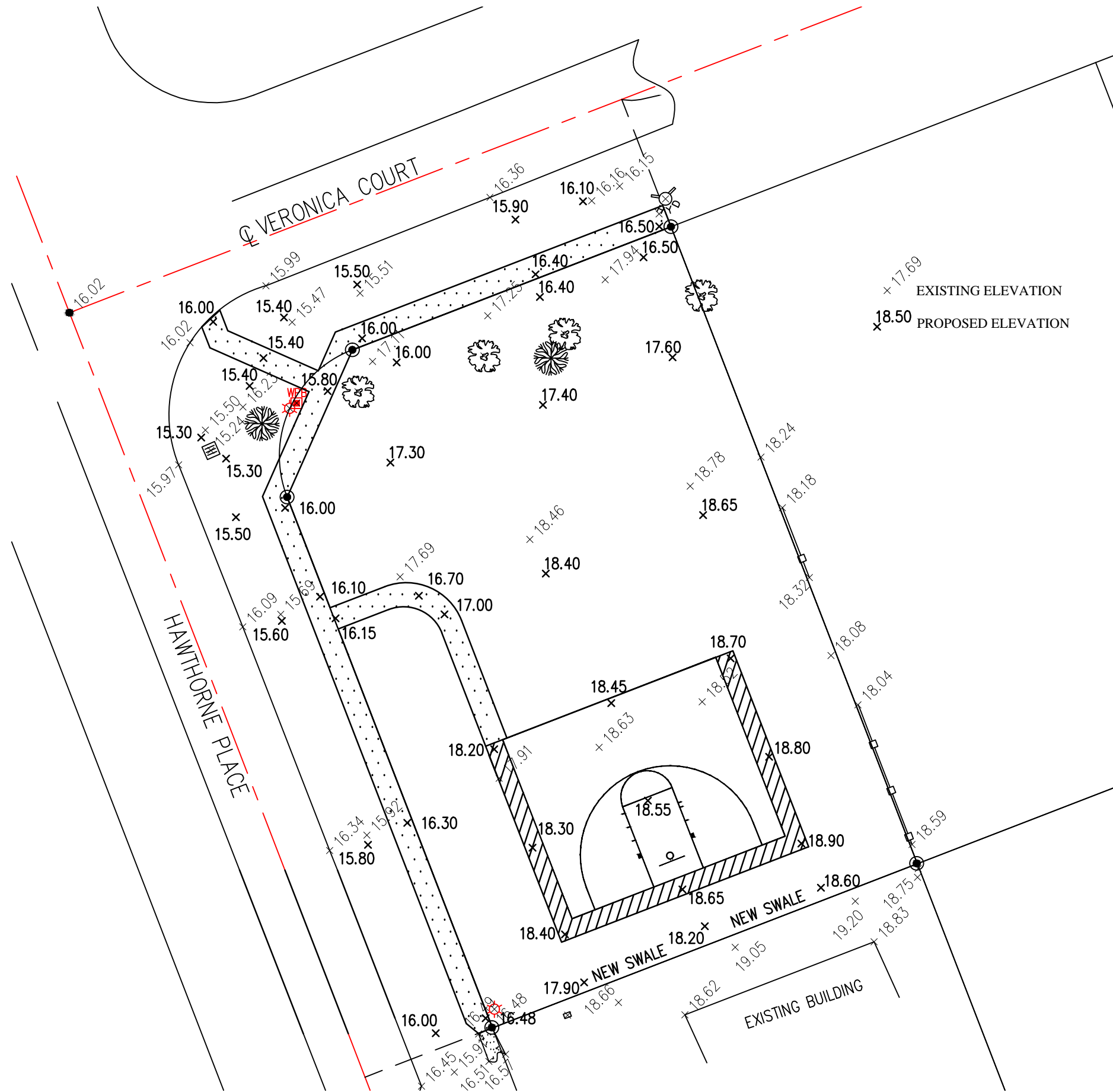
PROPOSED CIVIL PLAN- Scale: 1:300
