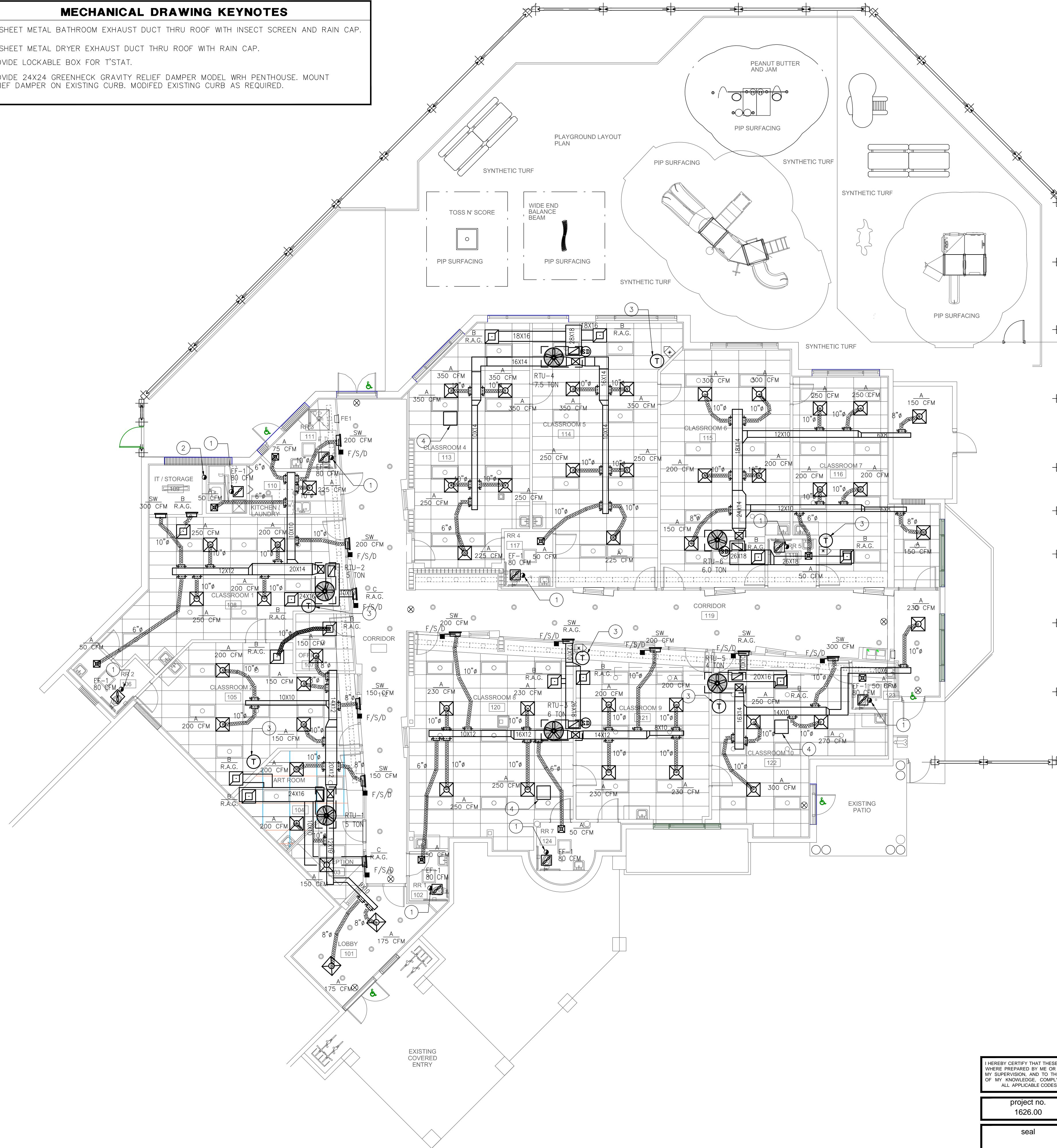
1ST FLOOR MECHANICAL PLAN scale: 1/8" = 1'-0"
