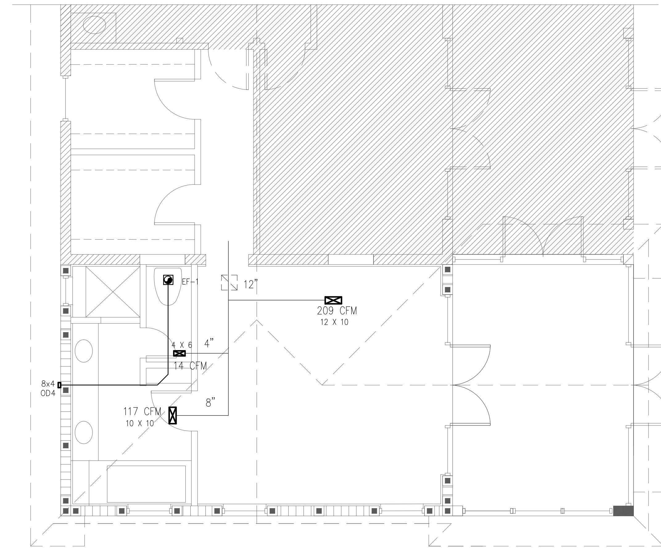
MECHANICAL PLAN SCALE: 1/8" = 1'-0"
