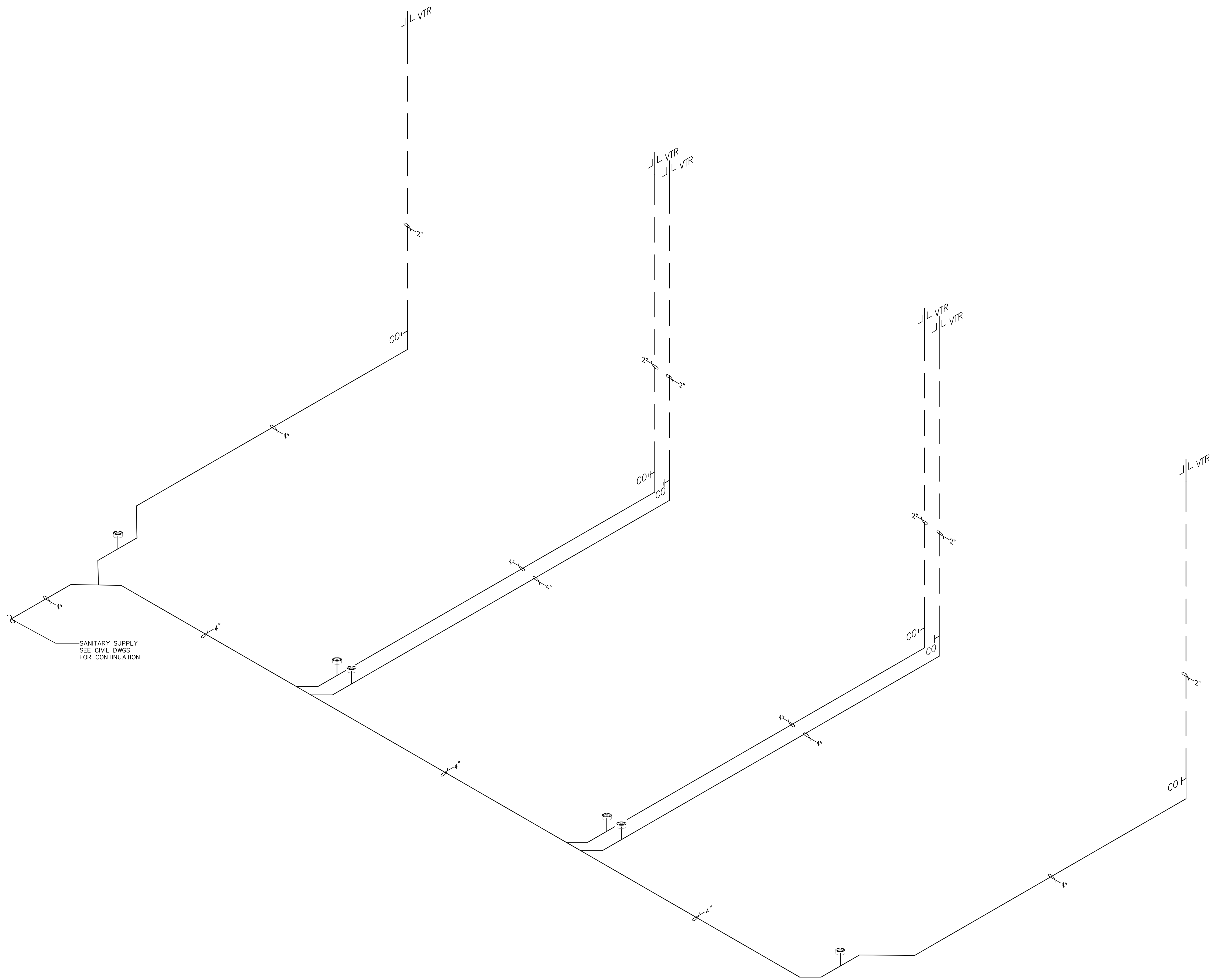
SANITARY PIPING ISOMETRIC NO SCALE
