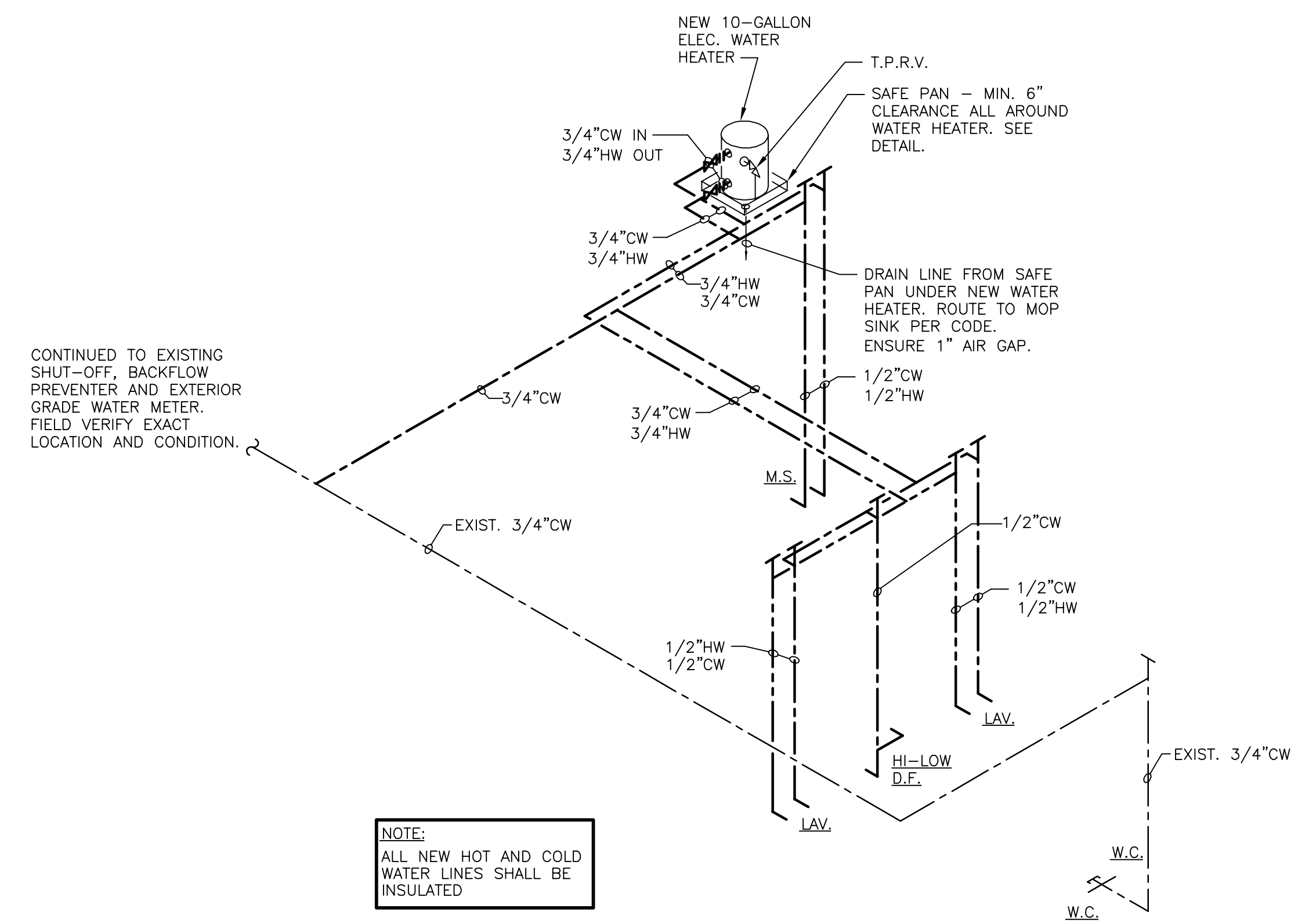
2 WATER RISER DIAGRAM SCALE: NONE
