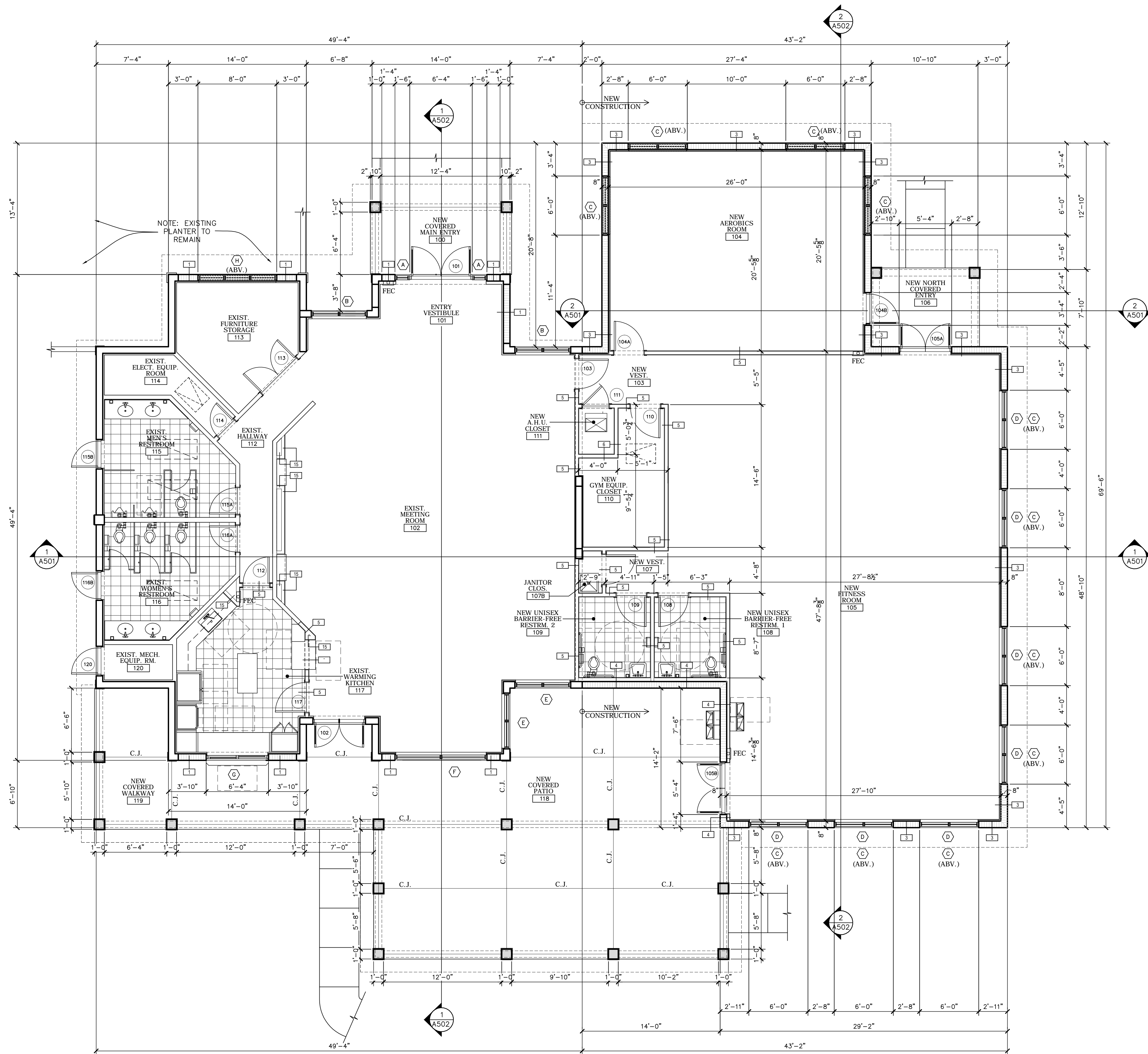
FLOOR PLAN CLUBHOUSE BUILDING SCALE: 3/16" = 1'-0"
