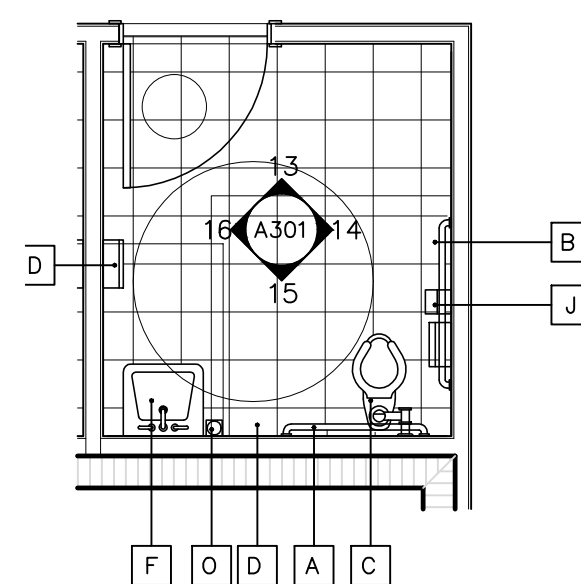
4 A301 RESTROOM PLAN SCALE: 1/4" = 1'-0" (SEE 'ID' DWGS. FOR RESTROOM FIXTURE & FINISHES SPECIFICATIONS)
