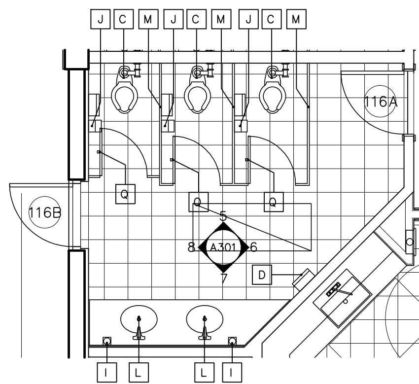
2 A301 RESTROOM PLAN SCALE: 1/4" = 1'-0" (SEE 'ID' DWGS. FOR RESTROOM FIXTURE & FINISHES SPECIFICATIONS)
