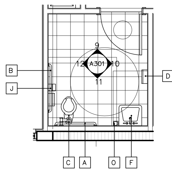
3 A301 RESTROOM PLAN SCALE: 1/4" = 1'-0" (SEE 'ID' DWGS. FOR RESTROOM FIXTURE & FINISHES SPECIFICATIONS)
