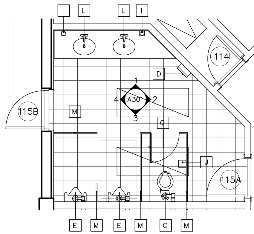
1 A301 RESTROOM PLAN SCALE: 1/4" = 1'-0" (SEE 'ID' DWGS. FOR RESTROOM FIXTURE & FINISHES SPECIFICATIONS)
