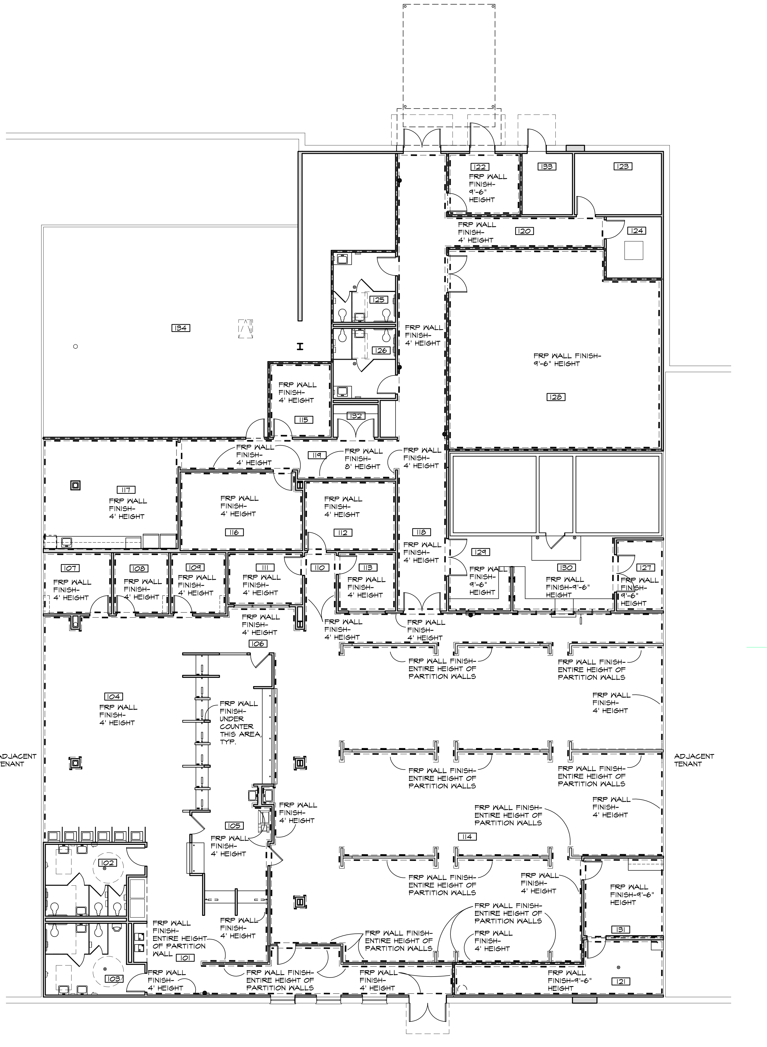
WALL FINISH KEY PLAN SCALE: 1/8"=1'-0"
