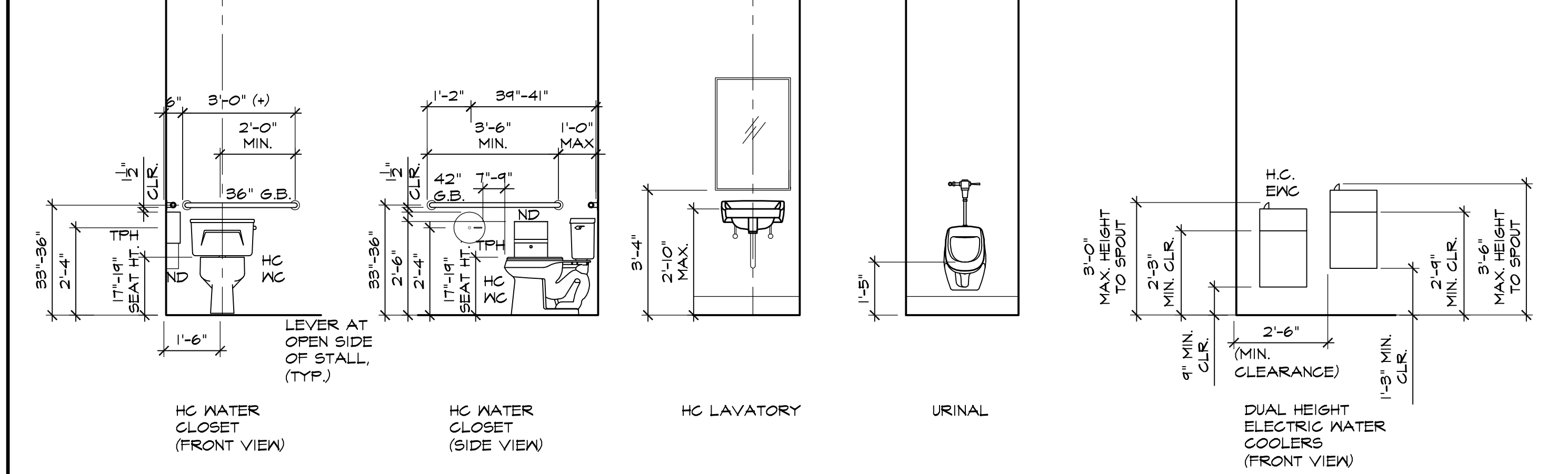
16 TYPICAL H.C. FIXTURES SCALE: 3/8"=1'-0"
