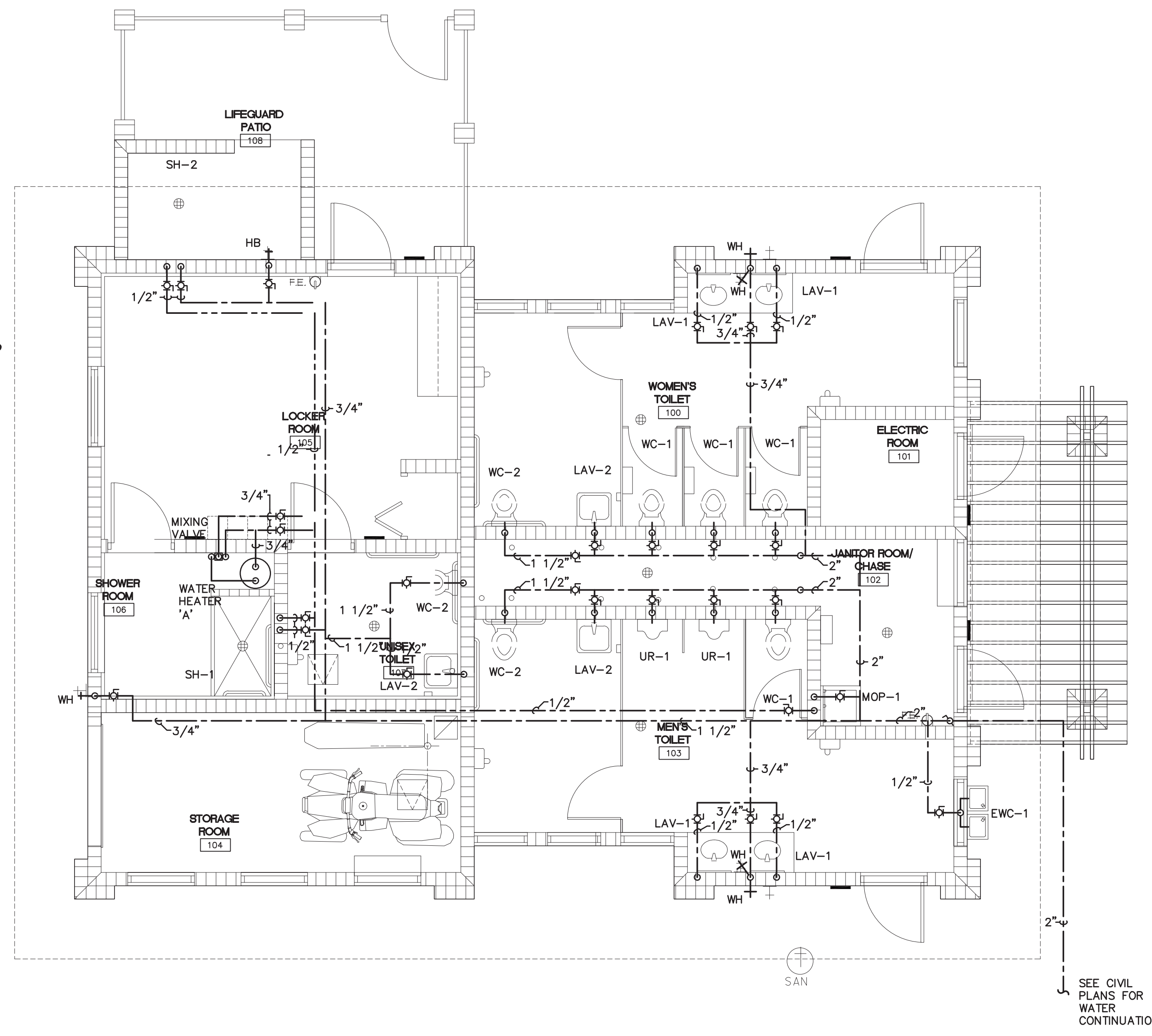
1 PLUMBING FLOOR PLAN - WATER PLAN P-3 SCALE: 1/4"=1'-0"
