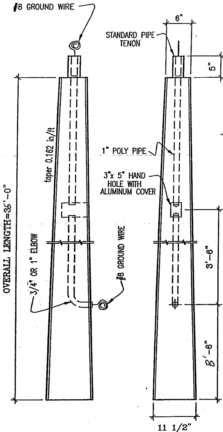
35 ft. TYPE II-0 POLE
