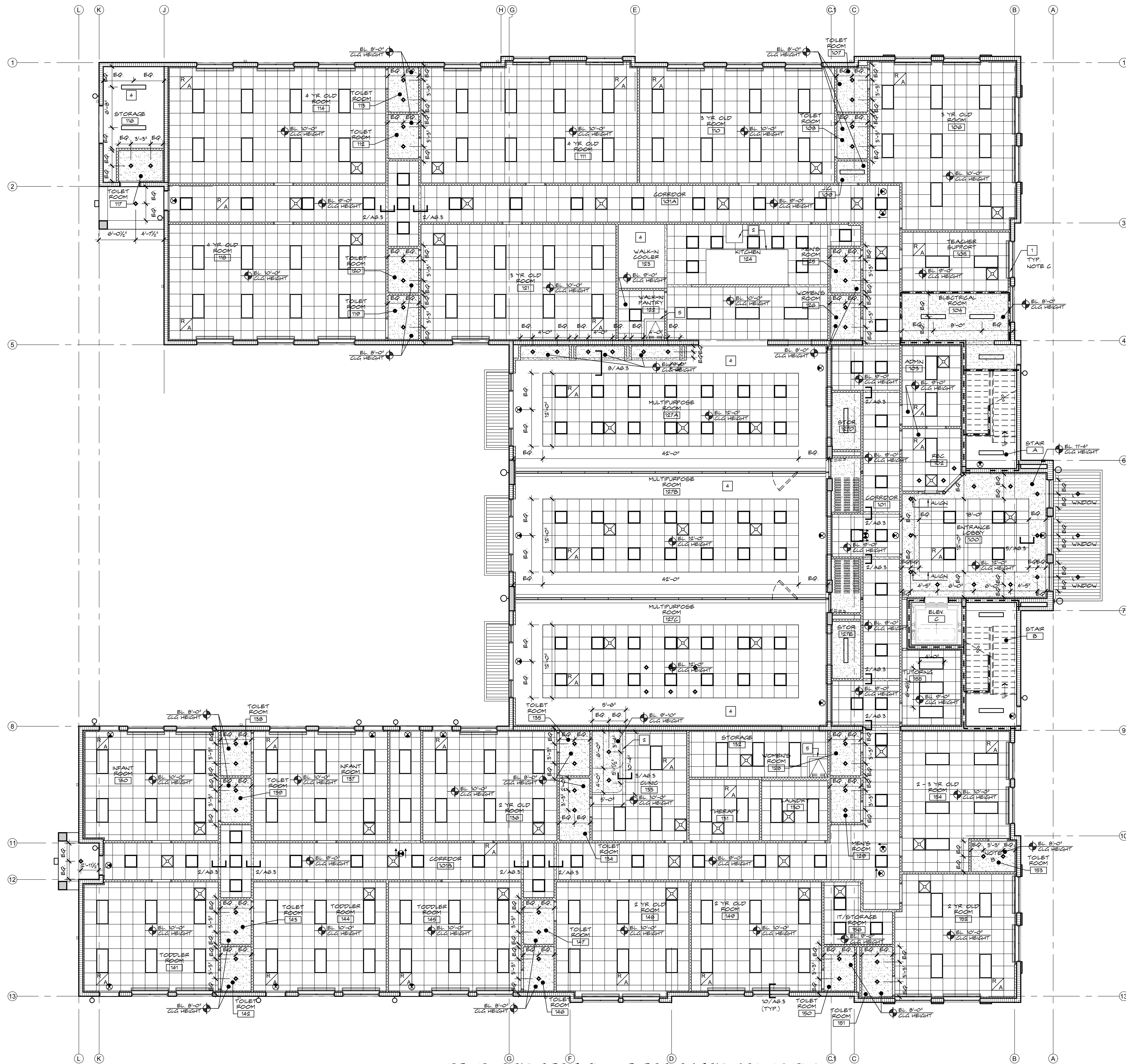
1 PROPOSED FIRST FLOOR REFLECTED CEILING PLAN SCALE: 1/8" = 1'-0"
