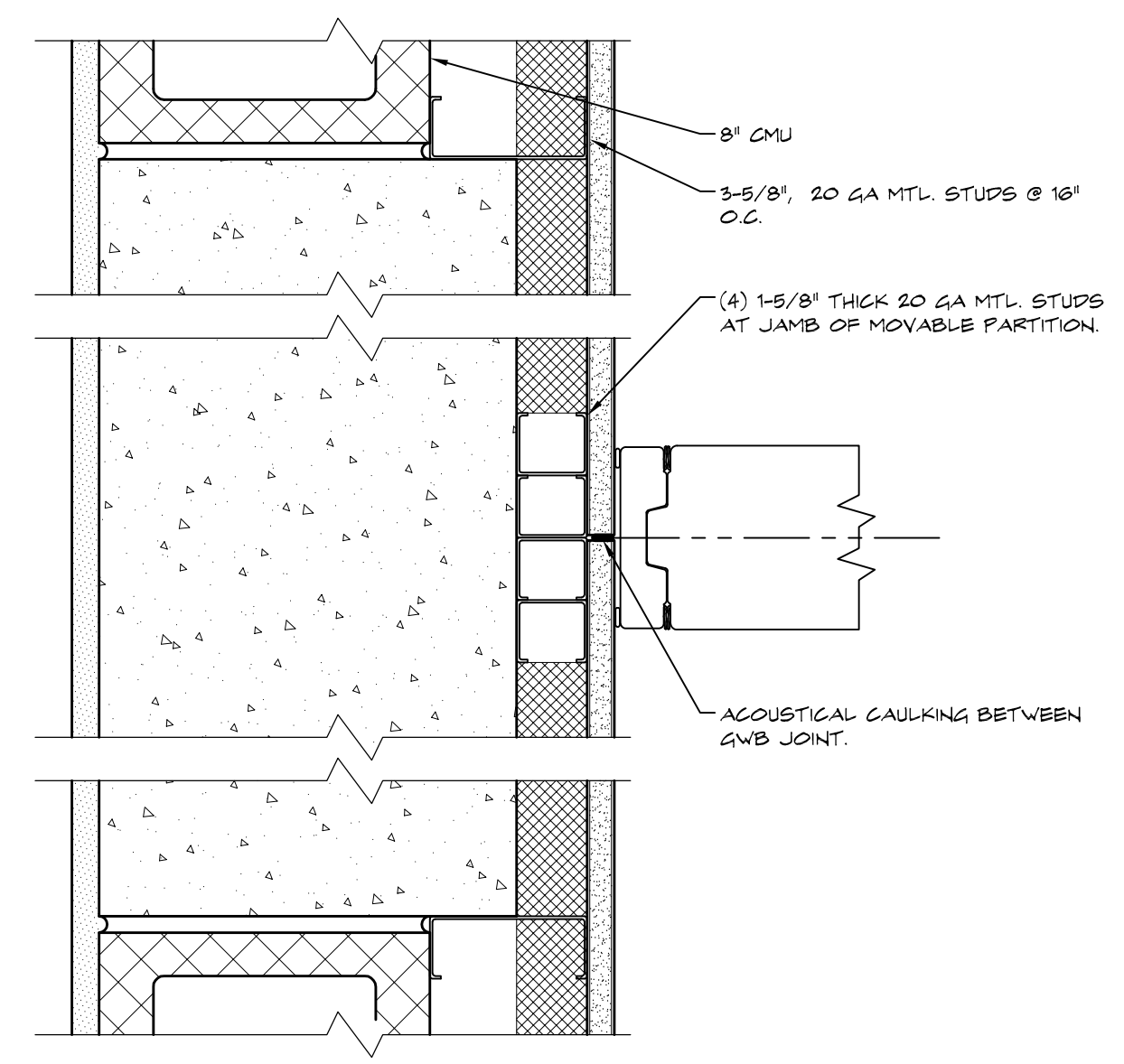
9 MOVABLE PARTITION JAMBS SCALE: 3/4" = 1'-0"
