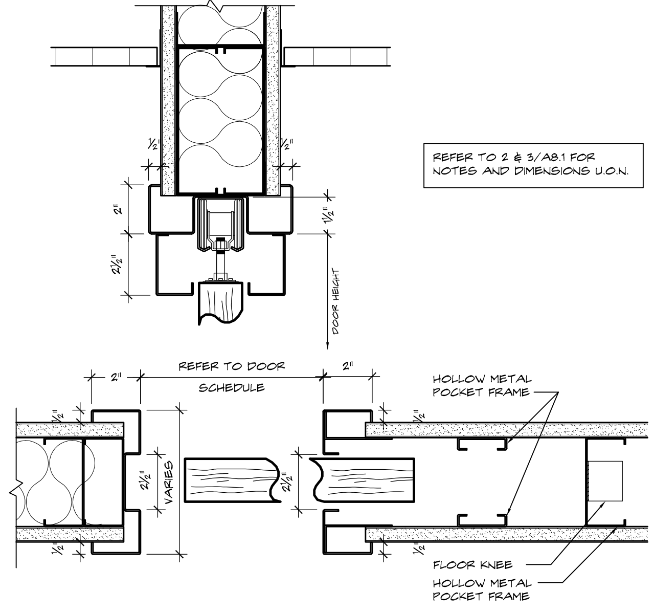
6 POCKET DOOR DETAILS SCALE: 3/4" = 1'-0"
