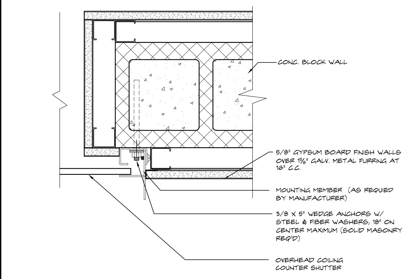
7 COILING COUNTER DOOR JAMB SCALE: 3/4" = 1'-0"
