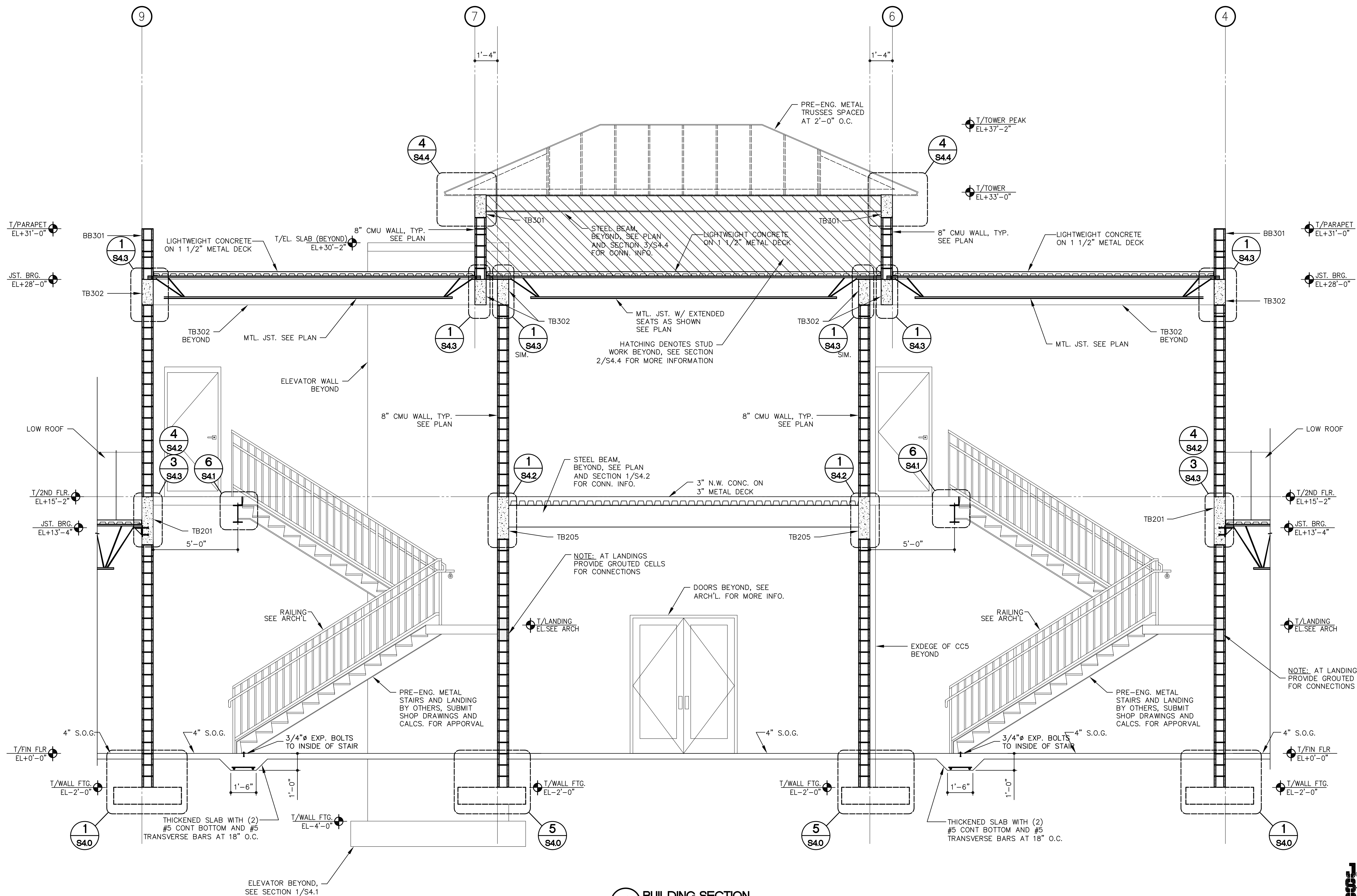
1 BUILDING SECTION SCALE: 3/8" = 1'-0" NOTE: FOR DTB REINF. INFO. REFER TO SECTION 8/S4.2
