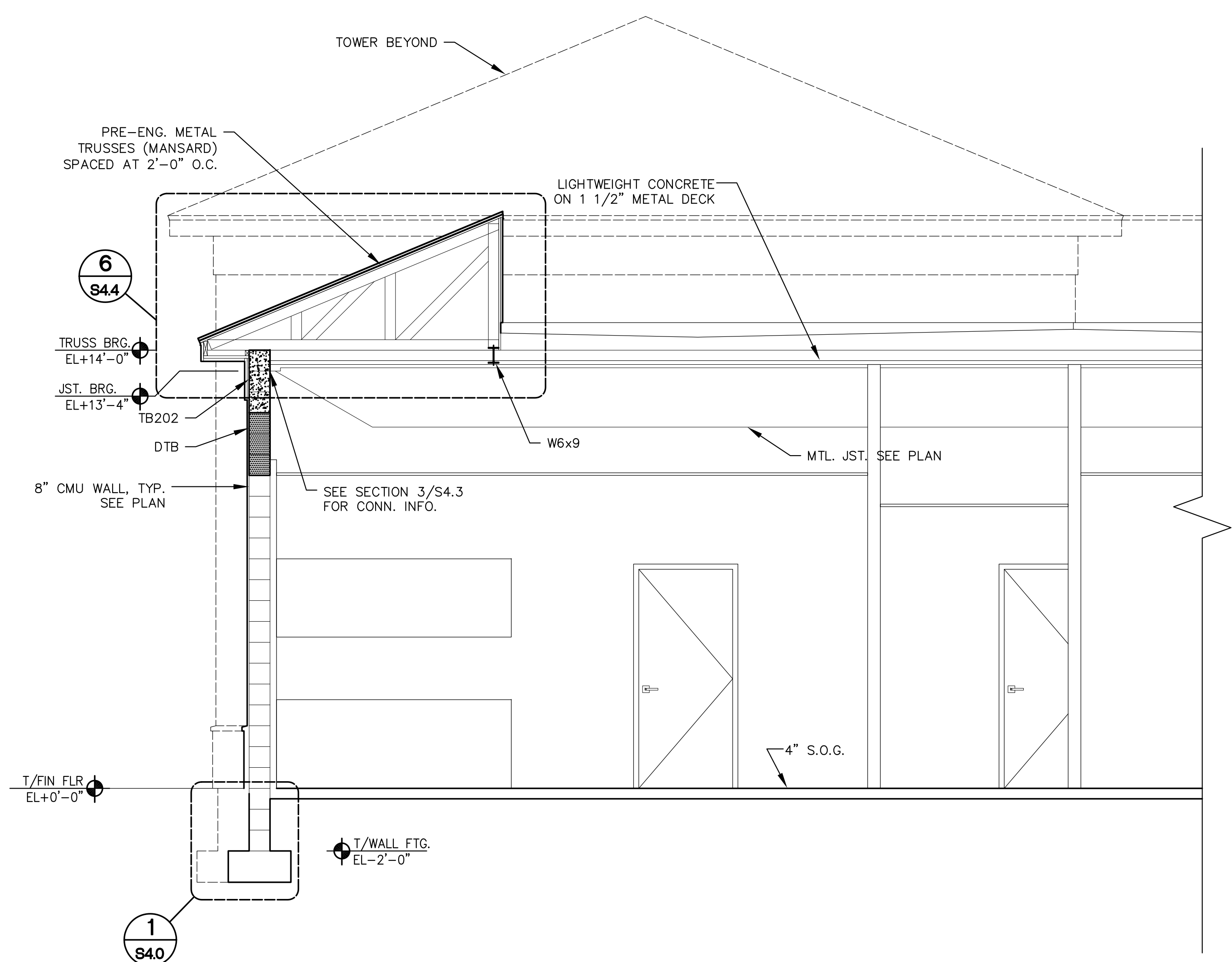
1 BUILDING SECTION SCALE: 3/8"=1'-0" NOTE: FOR DTB REINF. INFO. REFER TO SECTION 8/S4.2
