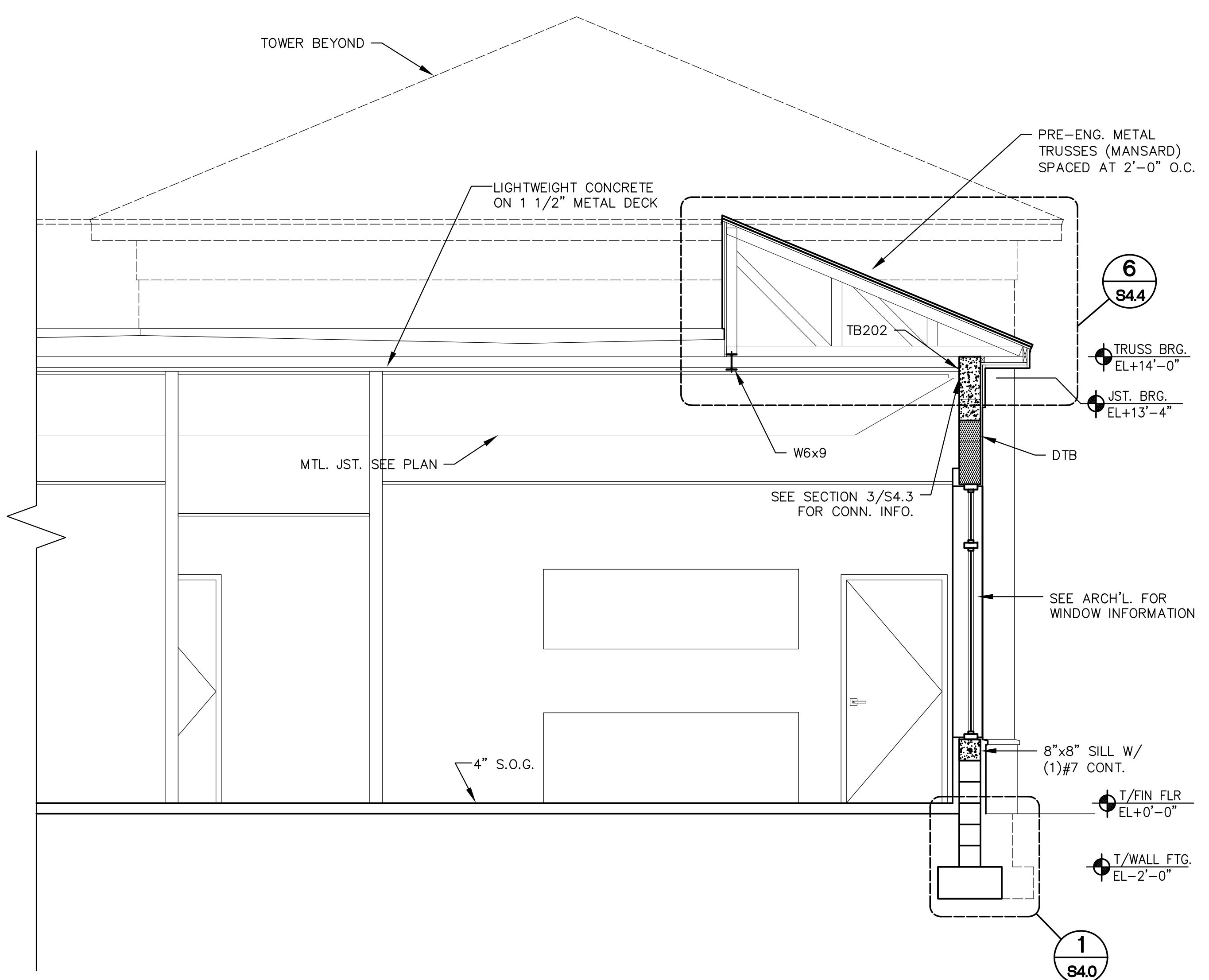
2 BUILDING SECTION SCALE: 3/8"=1'-0" NOTE: FOR DTB REINF. INFO. REFER TO SECTION 8/S4.2
