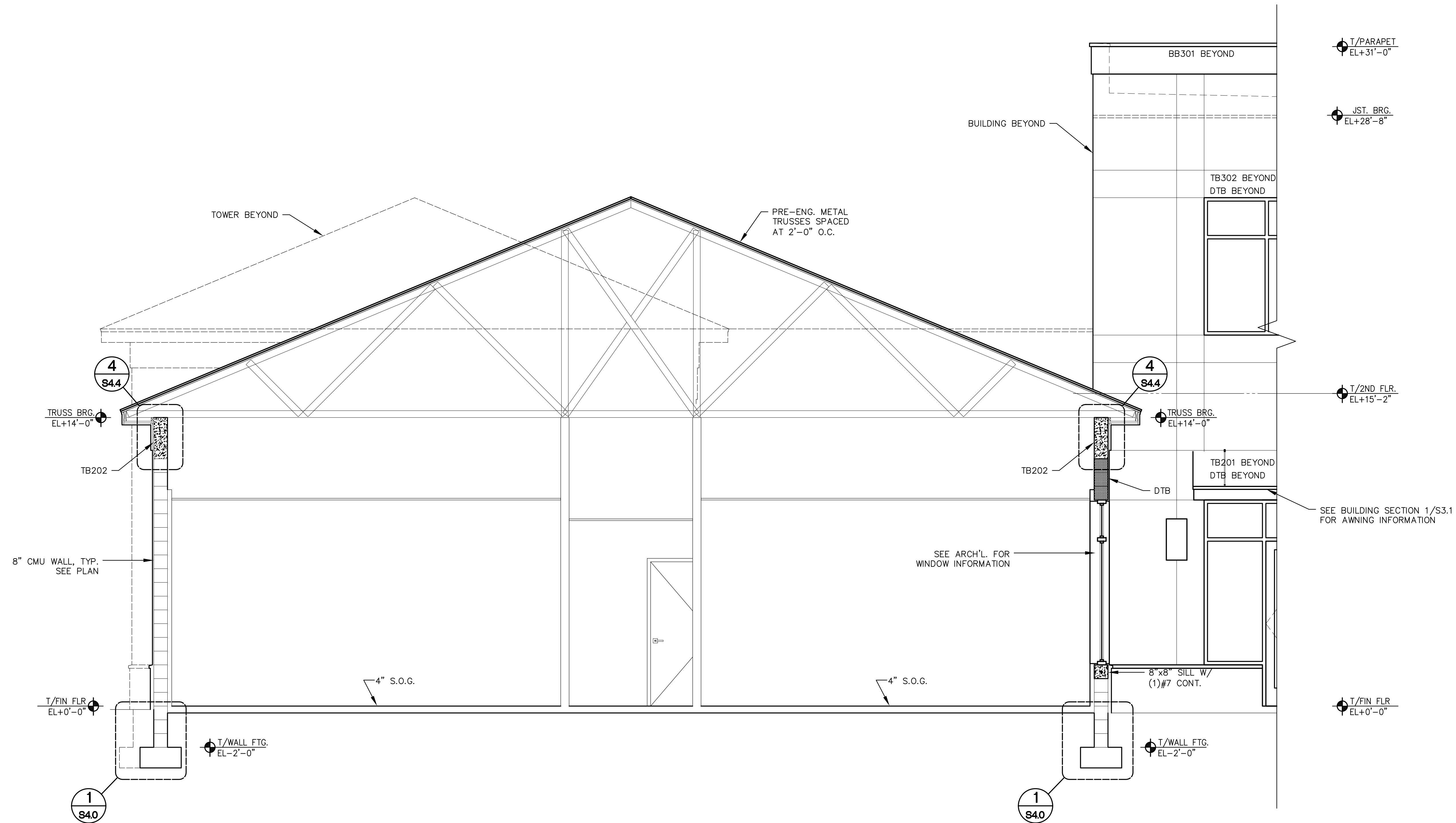
1 BUILDING SECTION SCALE: 3/8" = 1'-0" NOTE: FOR DTB REINF. INFO. REFER TO SECTION 8/S4.2
