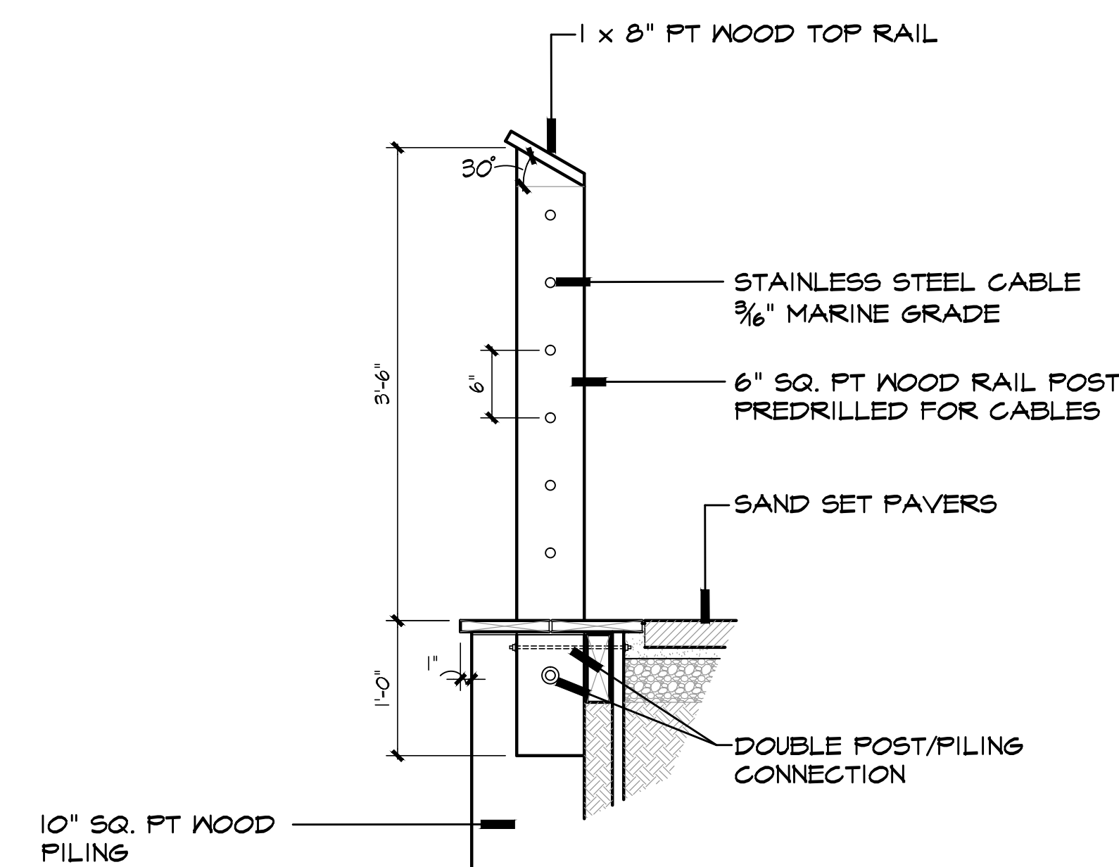
5 RAILING/BULKHEAD DETAIL SCALE: 1"=1'-0"
