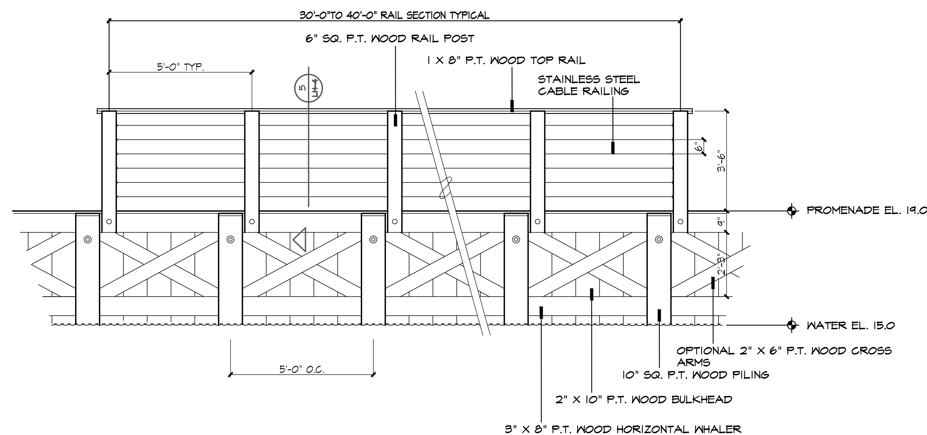
4 BULKHEAD RAILING ELEVATION SCALE: 1/2"=1'-0"
