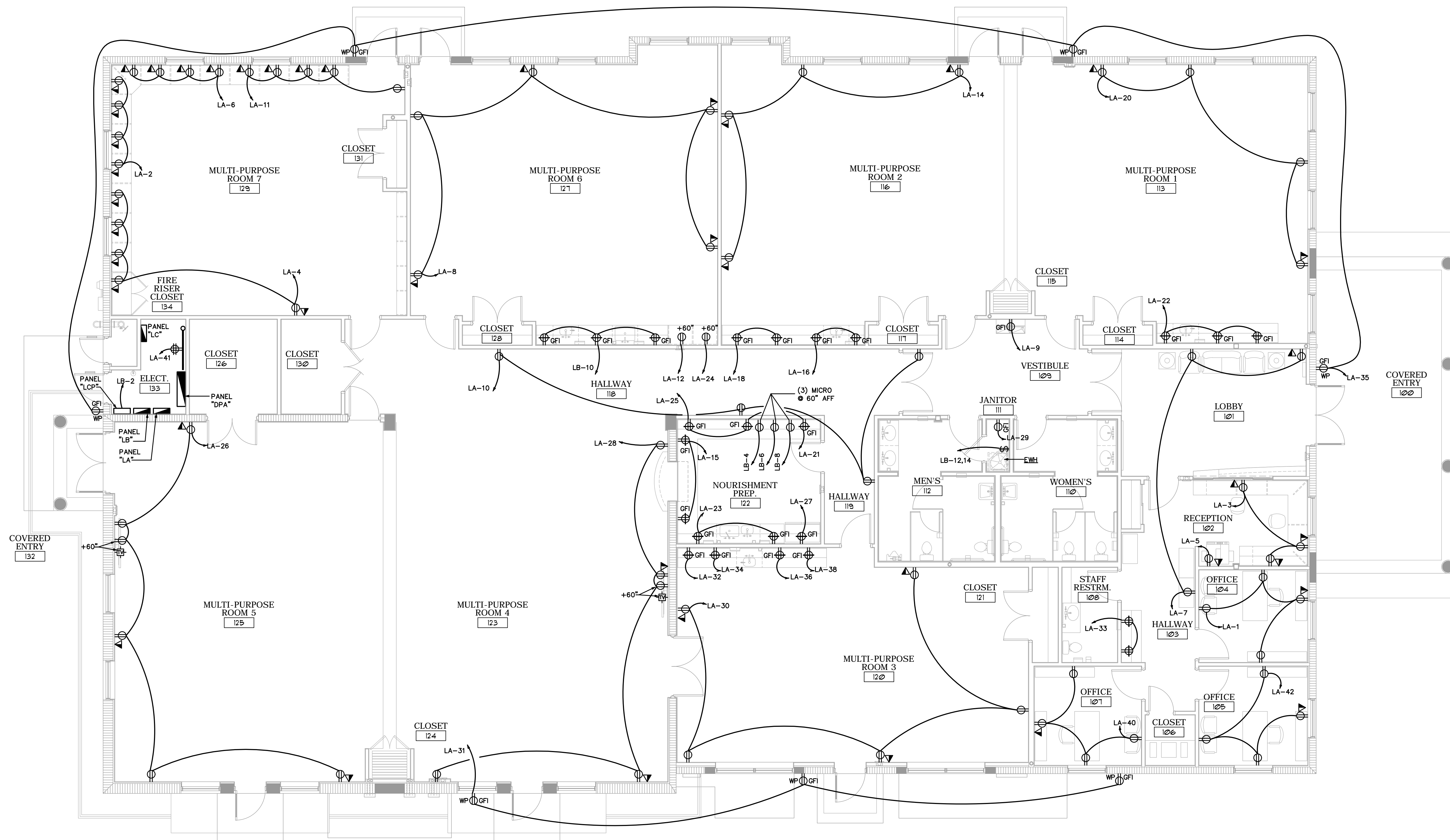
POWER PLAN 3/16"=1'-0" NORTH
