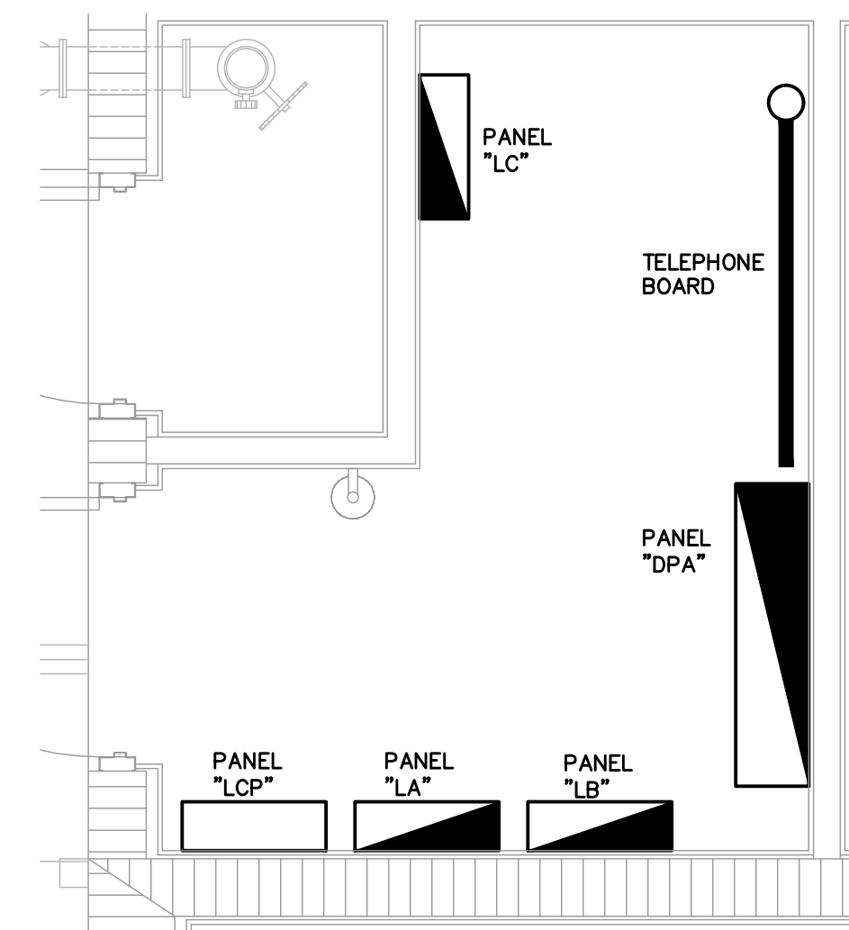
ENLARGED ELECTRIC ROOM 1/2"=1'-0" NORTH
