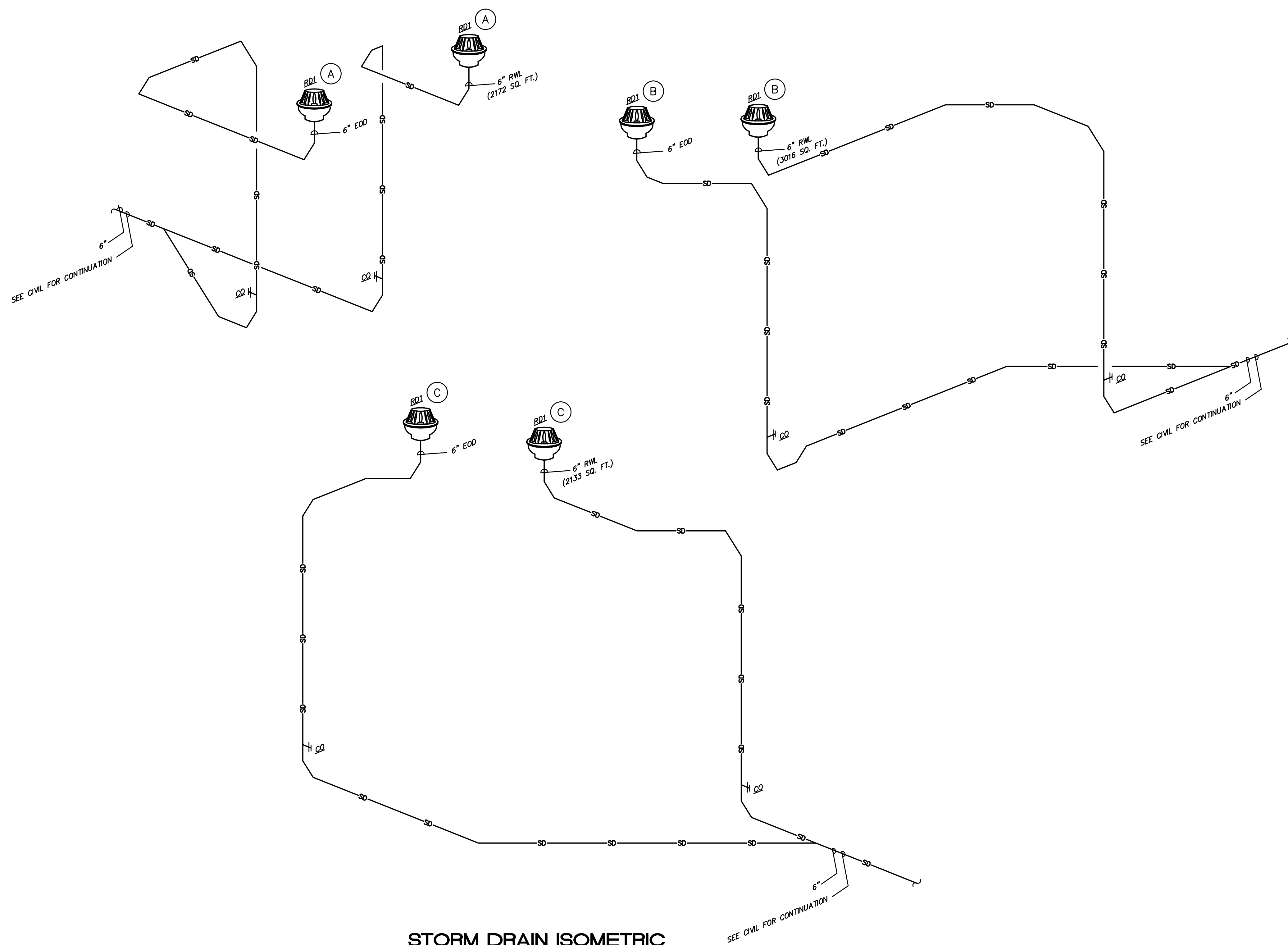
STORM DRAIN ISOMETRIC NOT TO SCALE
