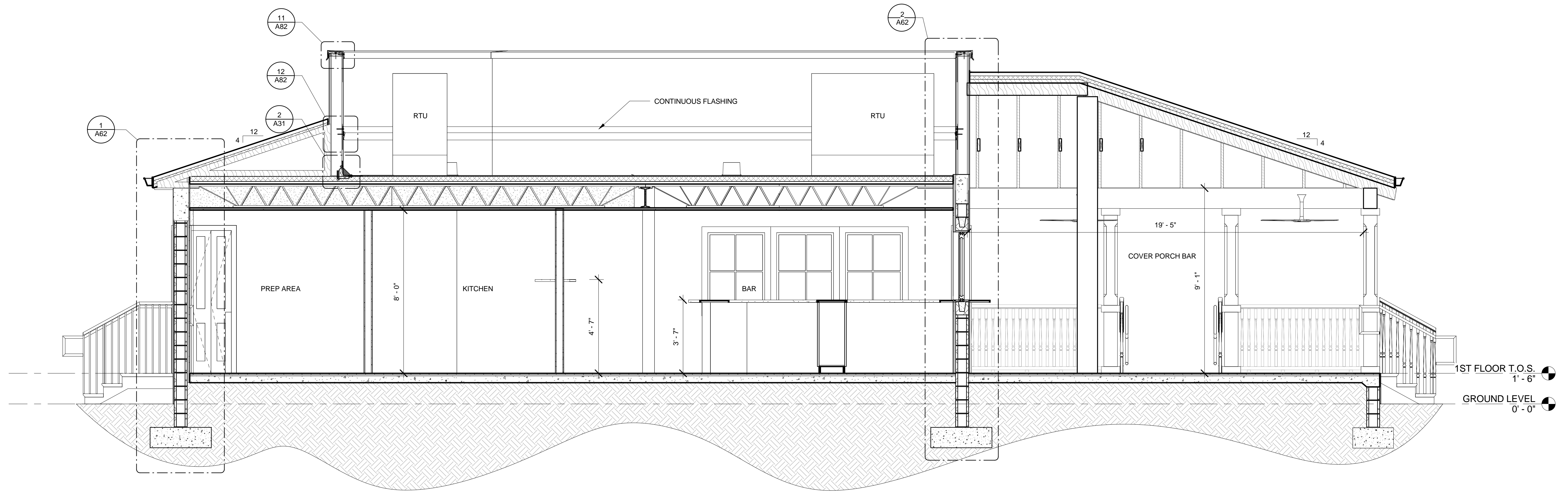
2 BUILDING SECTION SCALE: 3/8" = 1'-0"
