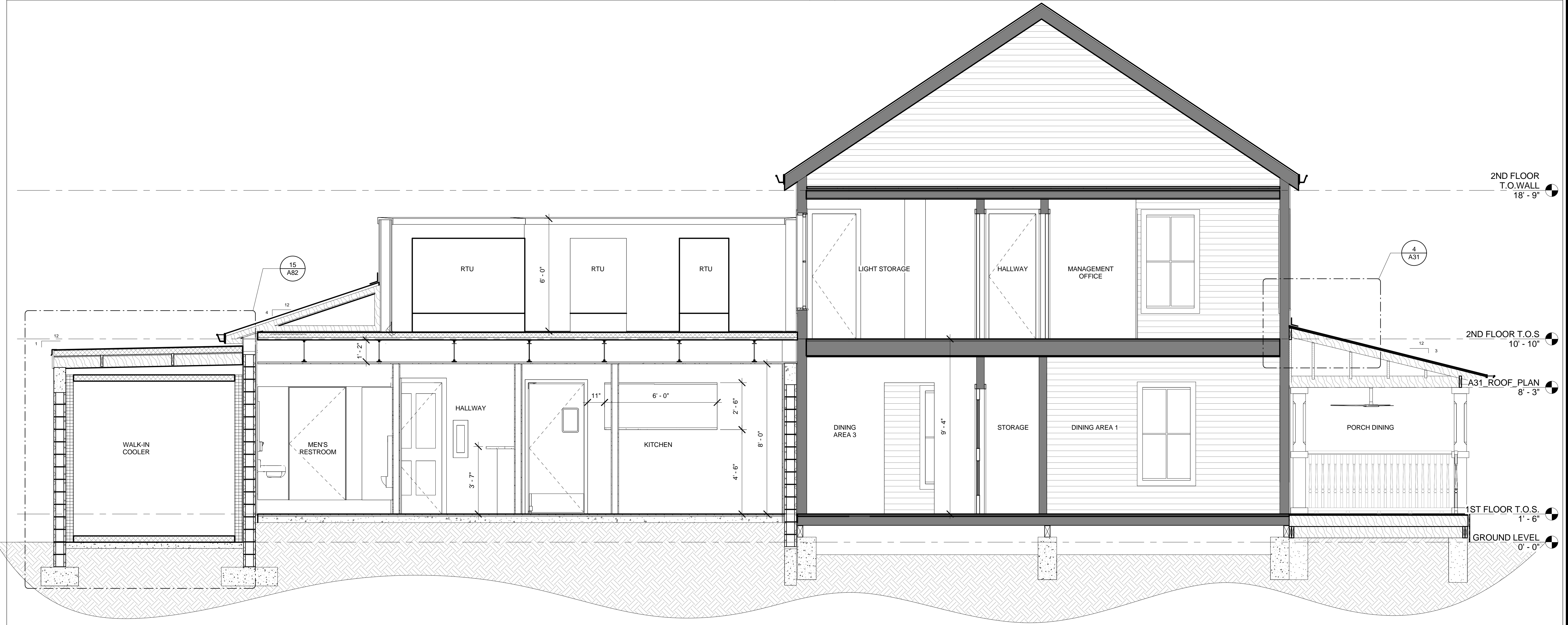
1 BUILDING SECTION SCALE: 3/8" = 1'-0"
