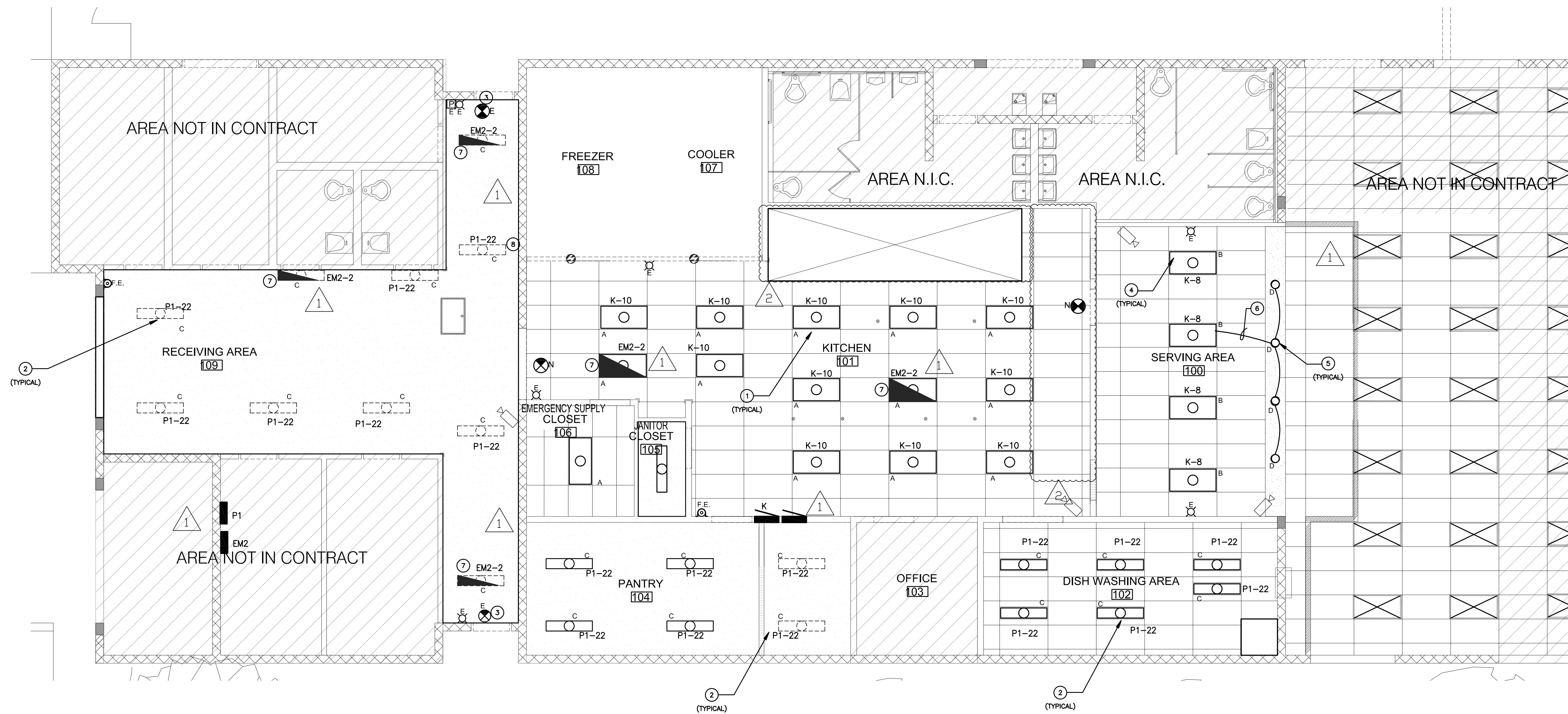
1 PROPOSED FLOOR PLAN - LIGHTING E-102 SCALE: 3/16" = 1'-0"
