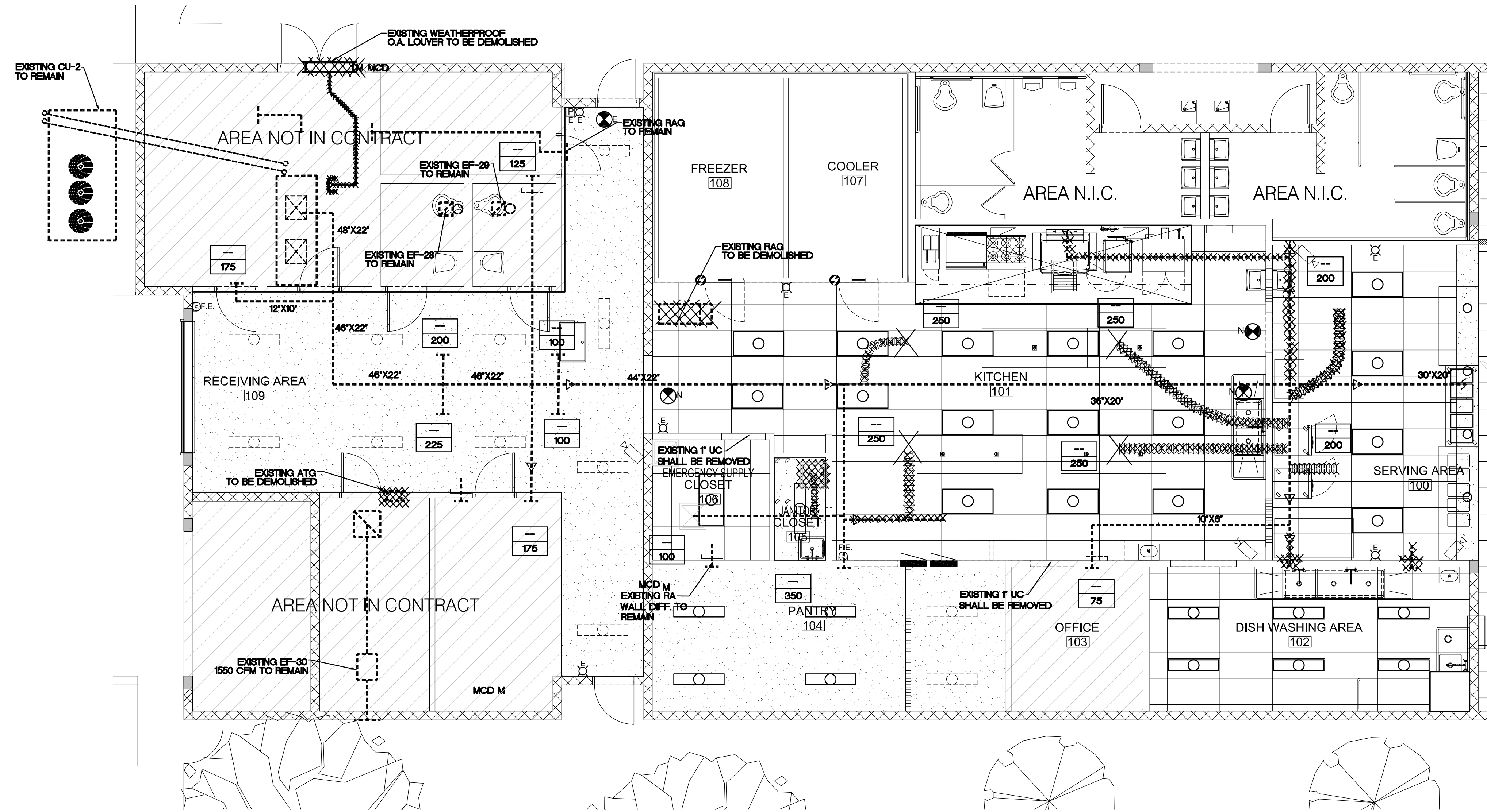
1 DEMOLITION FLOOR PLAN - MECHANICAL M-1 SCALE: 3/16" = 1'-0"
